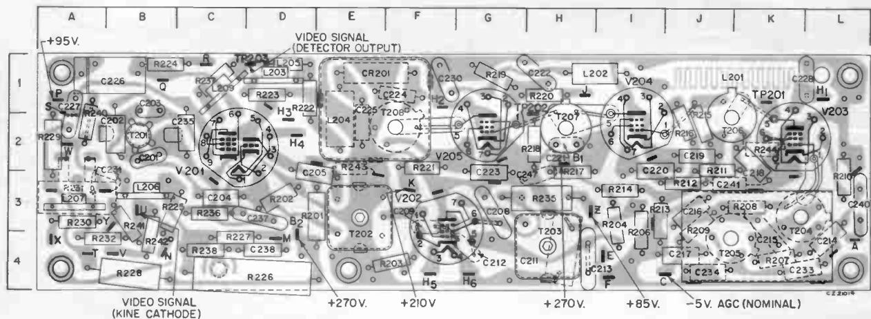
Figure 19—PW200 Sealed Circuit I-F and Video Assembly Composite Diagram
