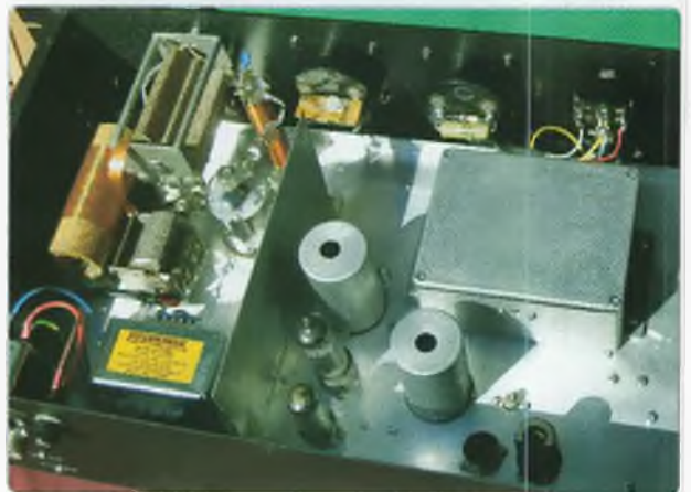
Photo 3: A view of the various components of the RF chassis.
