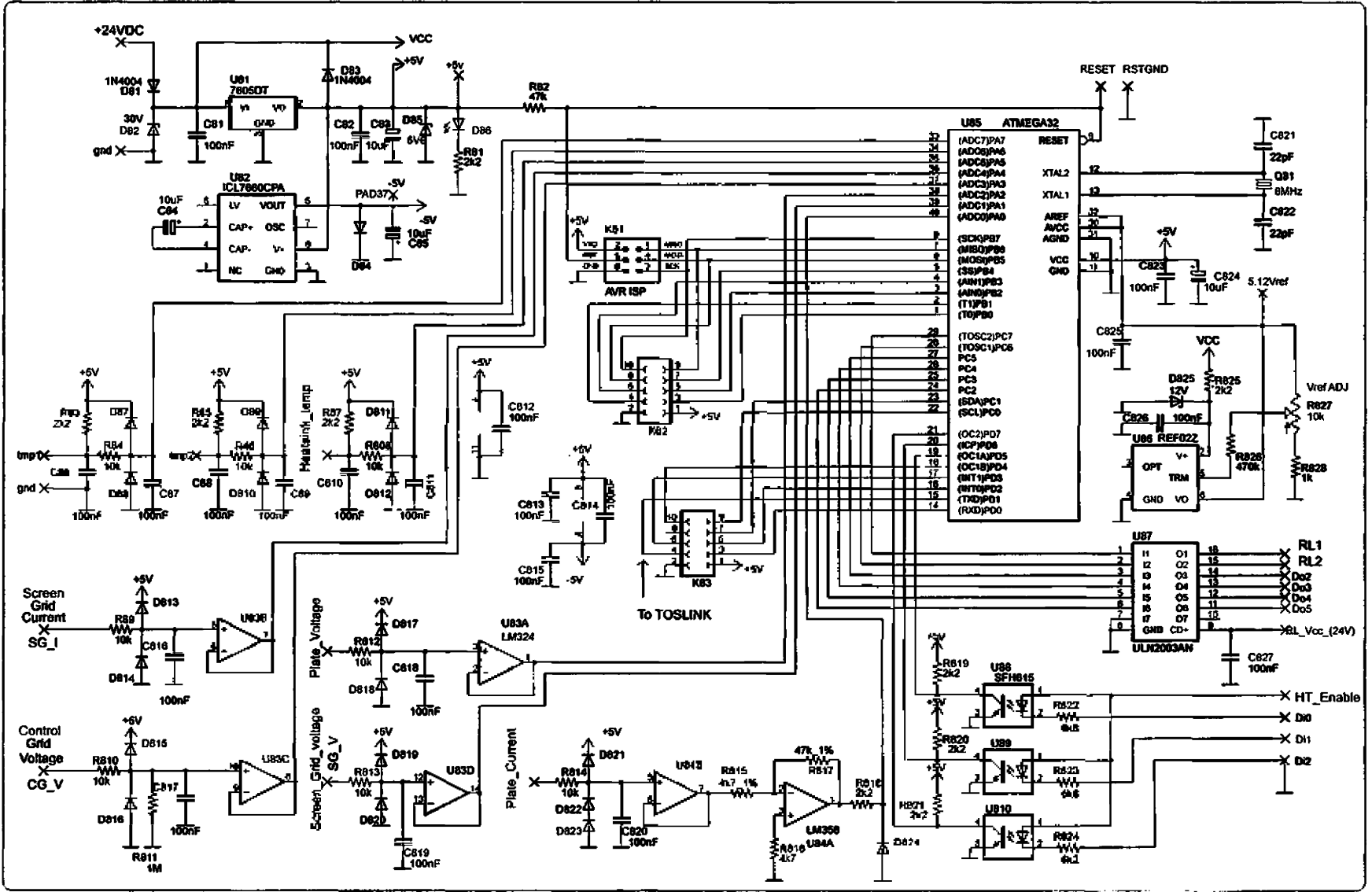
Figure 7: Main control board.
