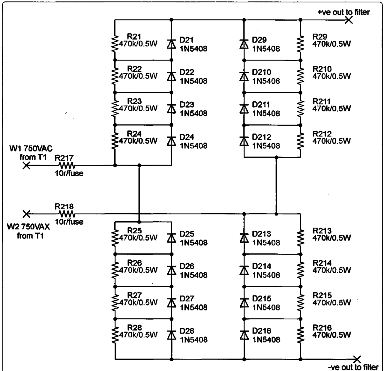
Figure 2: High voltage rectifier circuit board.
