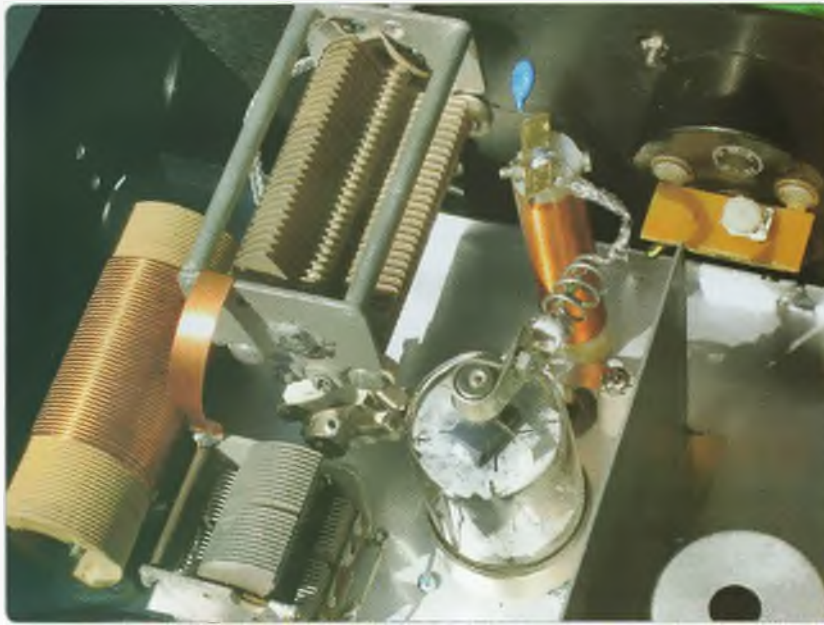
Photo 5: A close up view of the RF chassis.
