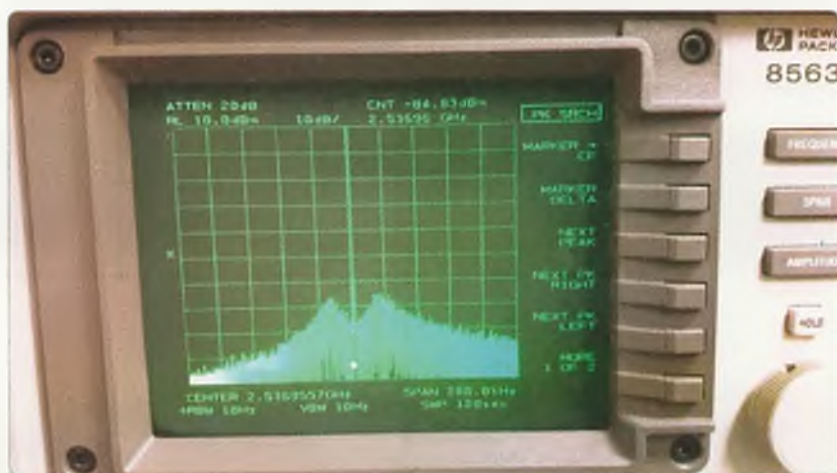
Photo 3: Spectrum analyser phase noise plot for ADF4351 PLL, with/without rail bypass.
