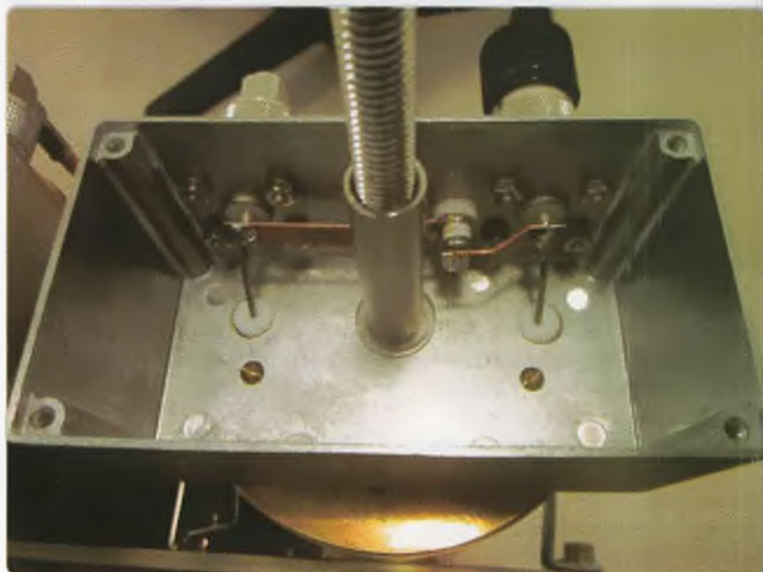
Photo 1: Low-side notch cavity showing location of Johanson 5202 trimmer capacitor on PTFE insulated bushing.
