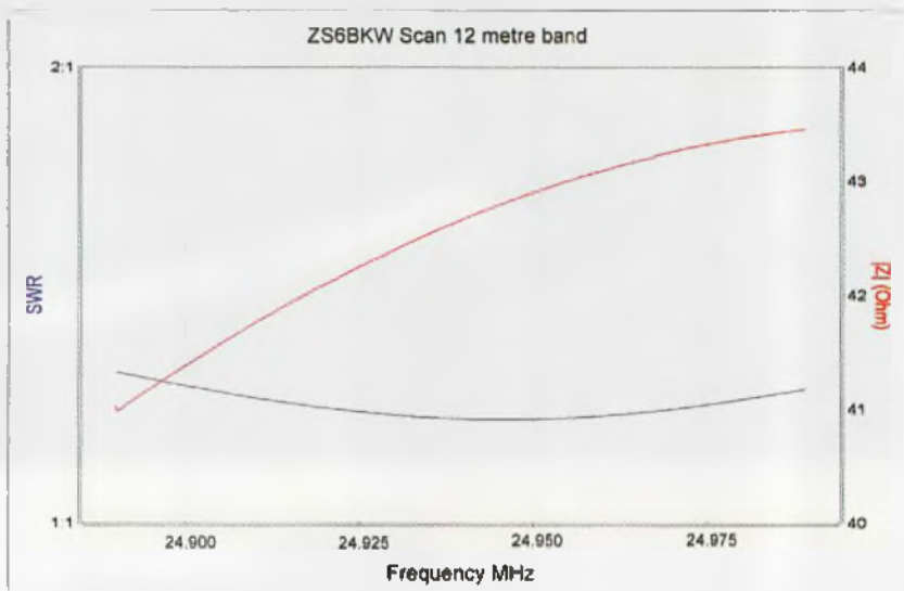
Figure 4: The 12 metre scan shows a very nice spread of low SWR across the whole band.
