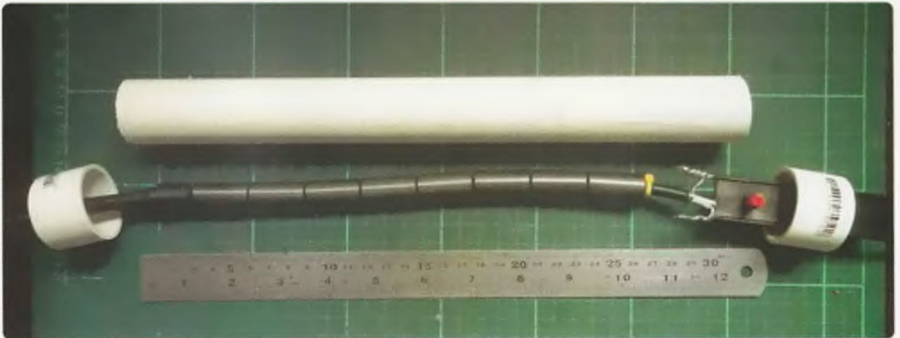
Photo 3: Assembly of the balun.
