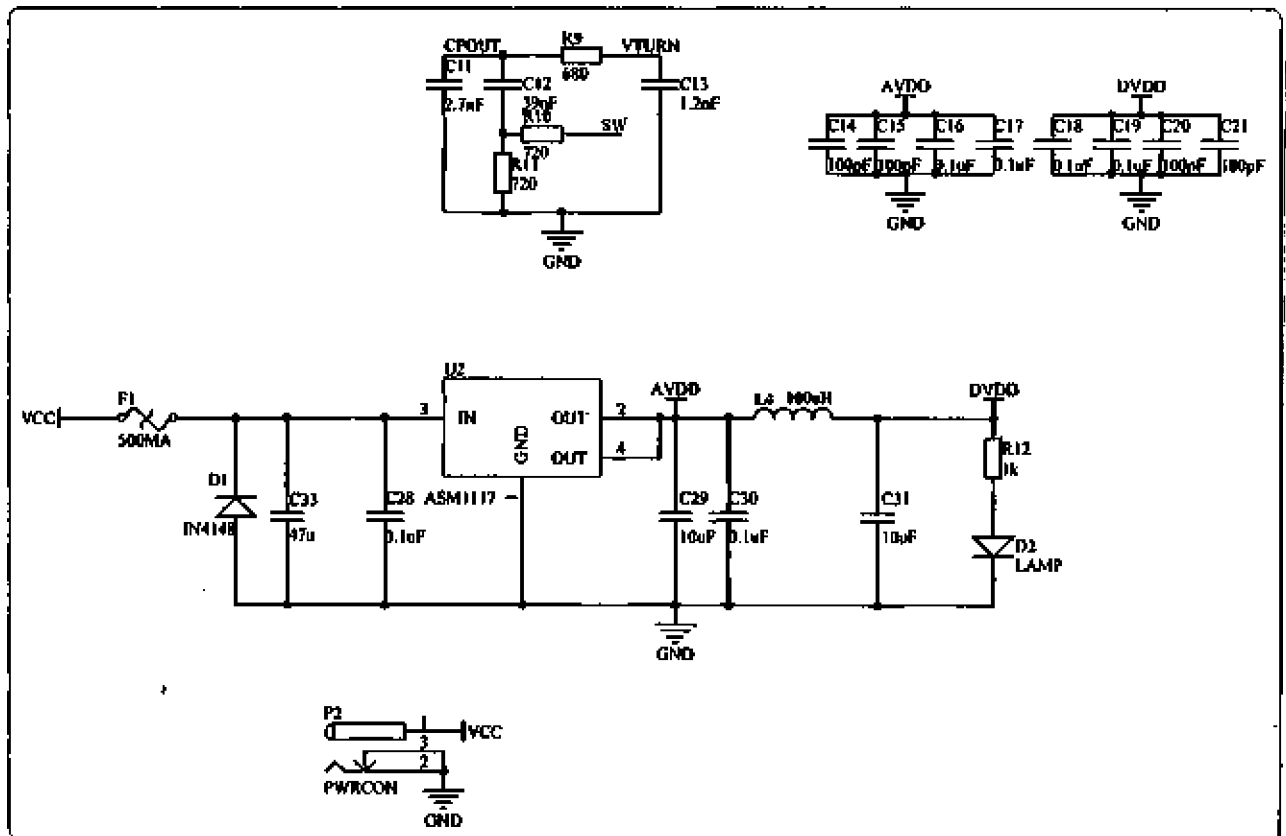
Photo 4: Suggested DC circuitry for the "Online" ADF4351 PLLs.
