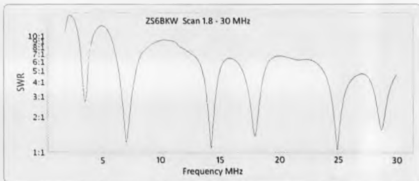
Figure 2: The full HF scan shows the dips for the five bands. Note the very good dips for 7, 14 and 24 MHz. 18 and 28 MHz are not as deep but still quite good, though some tuning would be desirable. 3.5 MHz is usable with a tuner. 10 and 21 MHz are poor.
