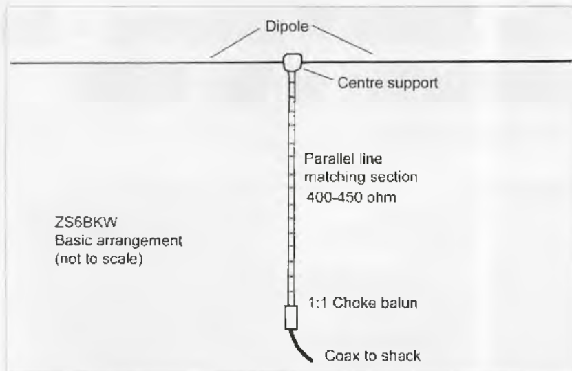
Figure 1: The basic arrangement of the ZS6BKW antenna.
