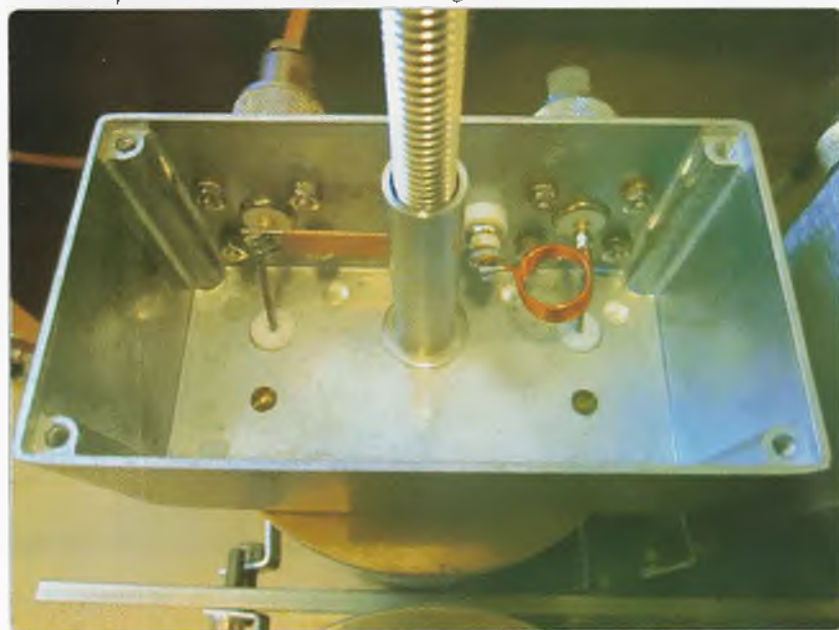
Photo 2: High-side notch cavity showing location of inductor and Johanson 5202 trimmer capacitor on PTFE insulated bushing.
