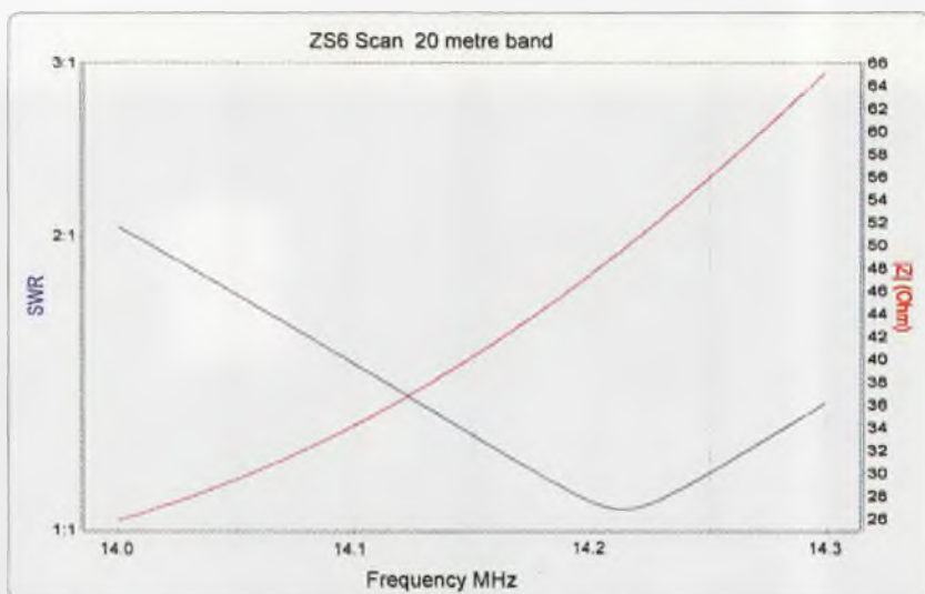
Figure 3: The 20 metre scan shows a good SWR curve, favouring the higher part of the band.
