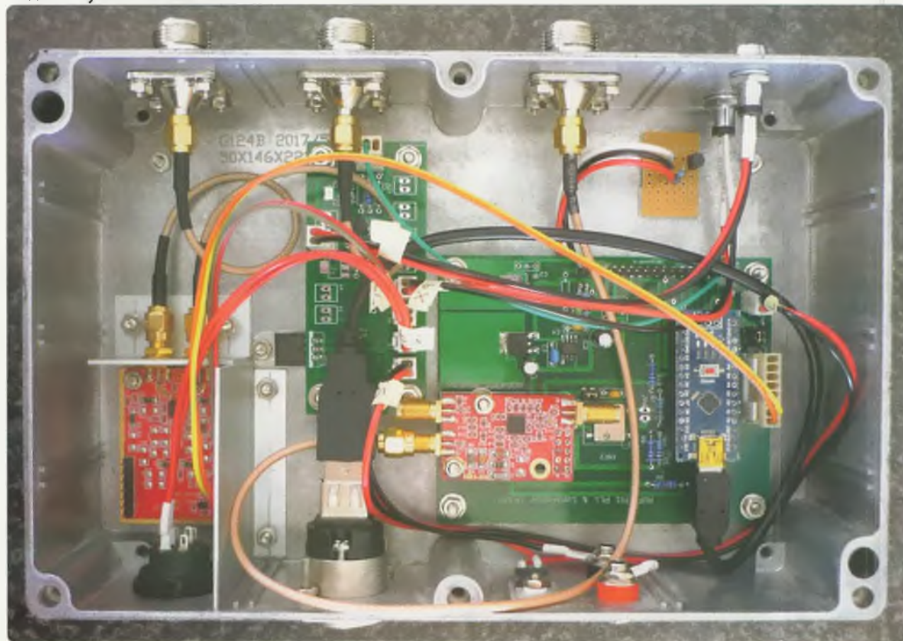
Photo 2: Layout in diecast box.
