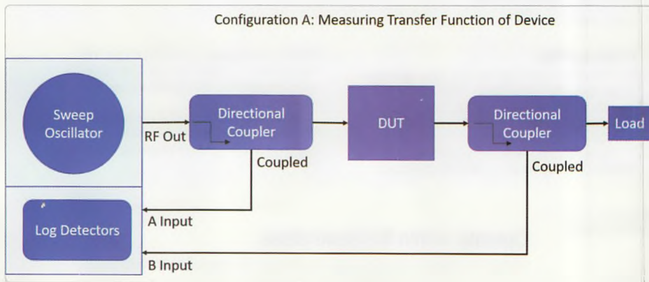
Figure 1: The classic configuration for measuring two port transmission gain / loss.
