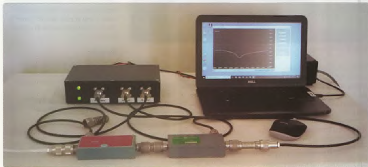
Photo 1: The Scalar Network Analyser with strip-line directional couplers.
