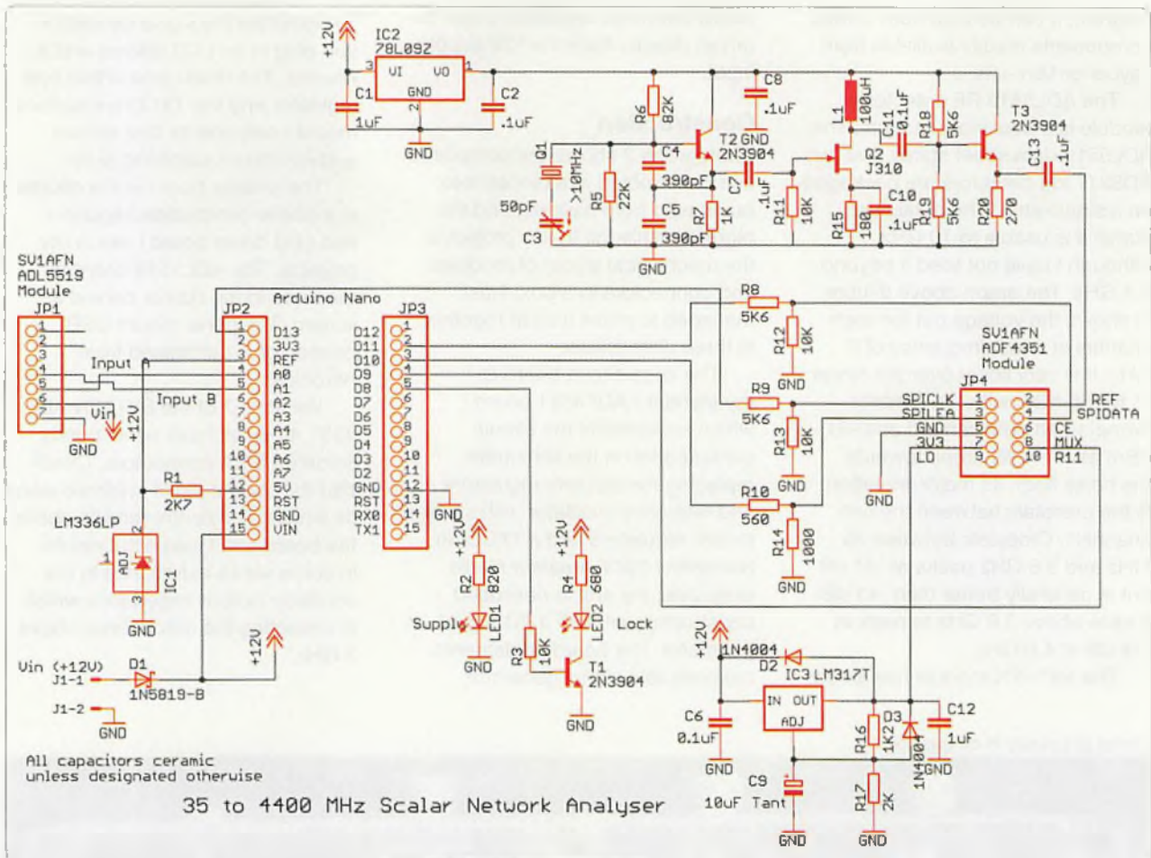
Figure 5: Circuit Diagram.
