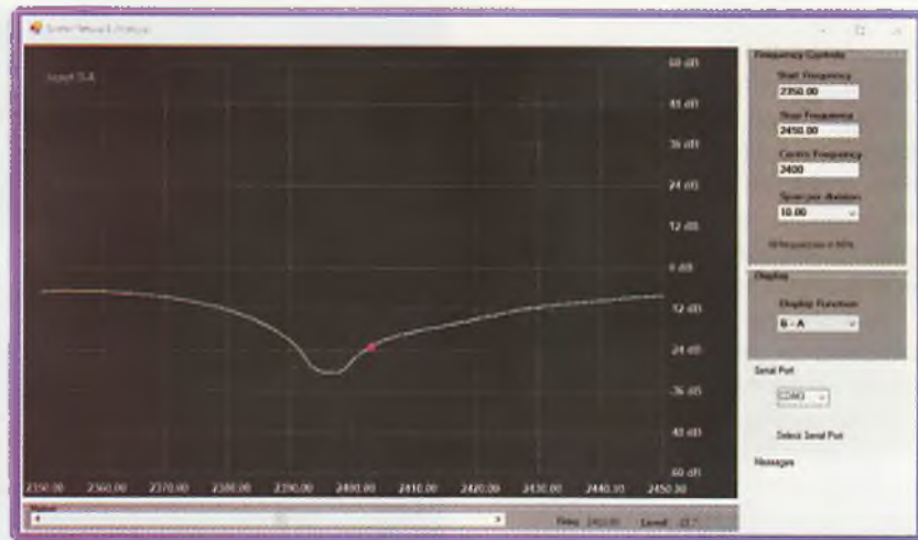
Figure 7: The Windows user interface, showing the swept return loss for a 13 cm Yagi.
