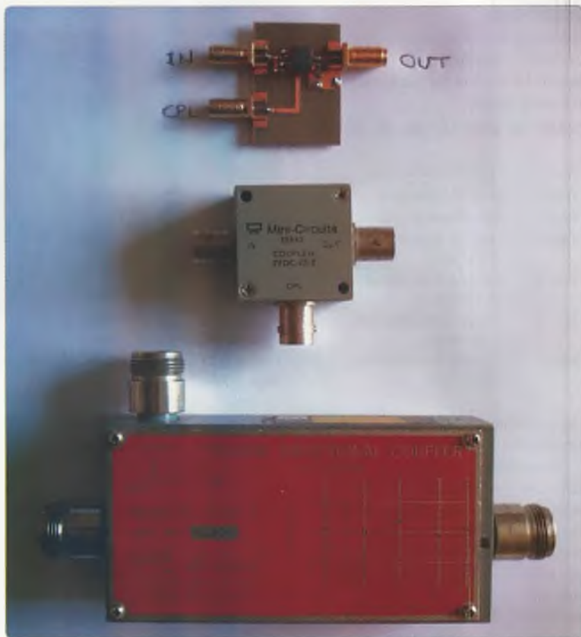
Photo 3: VHF homebrew, and commercial transformer couplers with a microwave strip-line coupler.
