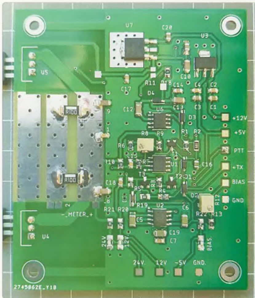
Photo 10: GasFET/GaN amplifier Power Supply – VK5KK.
