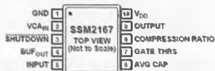
Figure 17: The microphone amplifier and compressor is based on a surface mount device (SMD) that integrates all the functions.
