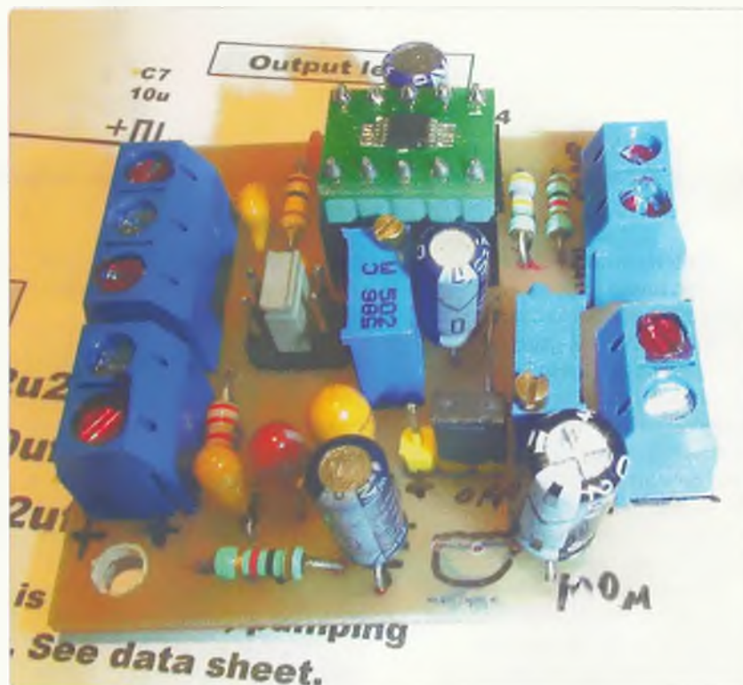
Photo 2B: The mic amplifier compressor board. Note the SSM2167 IC mounted on a plug-in adapter DIL board.
