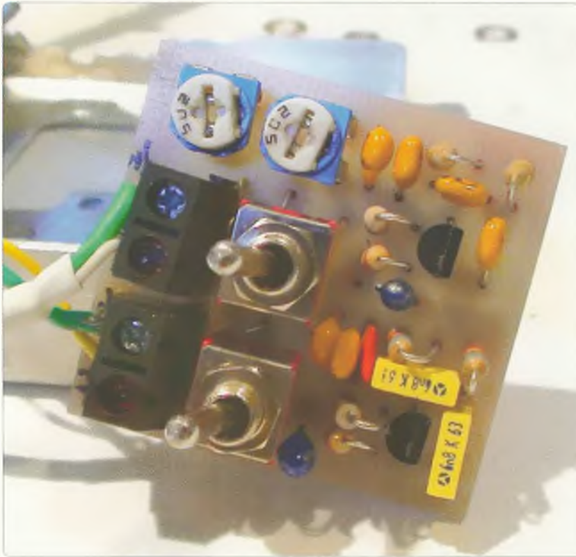
Photo 2C: The two-tone oscillator board. It mounts to a subpanel with the two toggle switch shafts.
