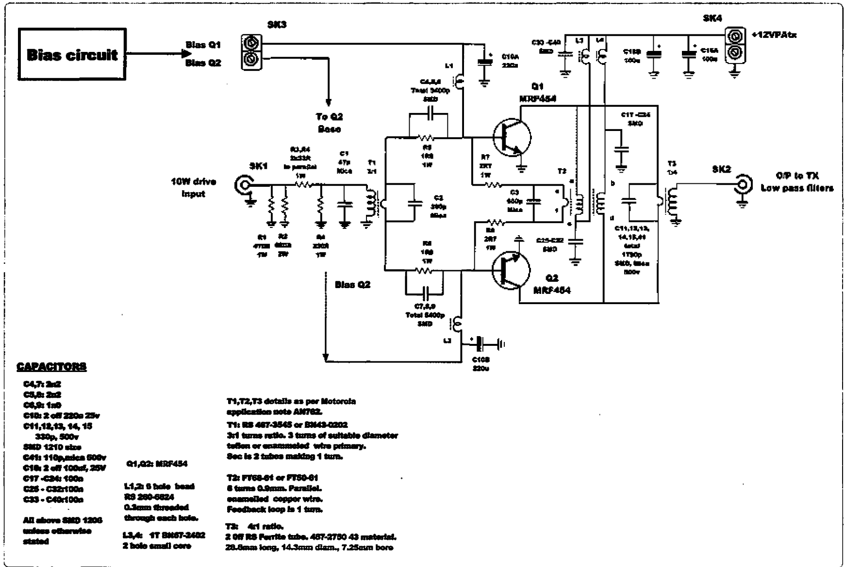
Figure 22: 100 W RF Power amplifier.
