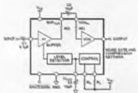
Figure 17: The microphone amplifier and compressor is based on a surface mount device (SMD) that integrates all the functions.
