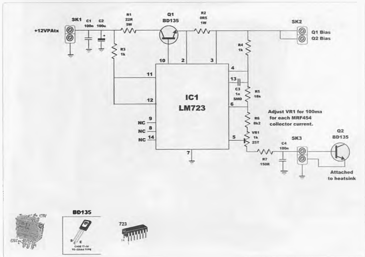
Figure 23: 100 W RF Power amplifier bias.
