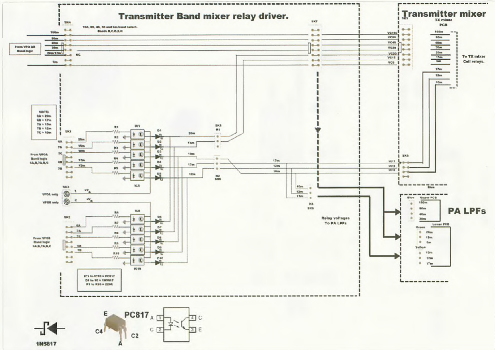
Figure 20: Transmitter Band mixer relay driver.
