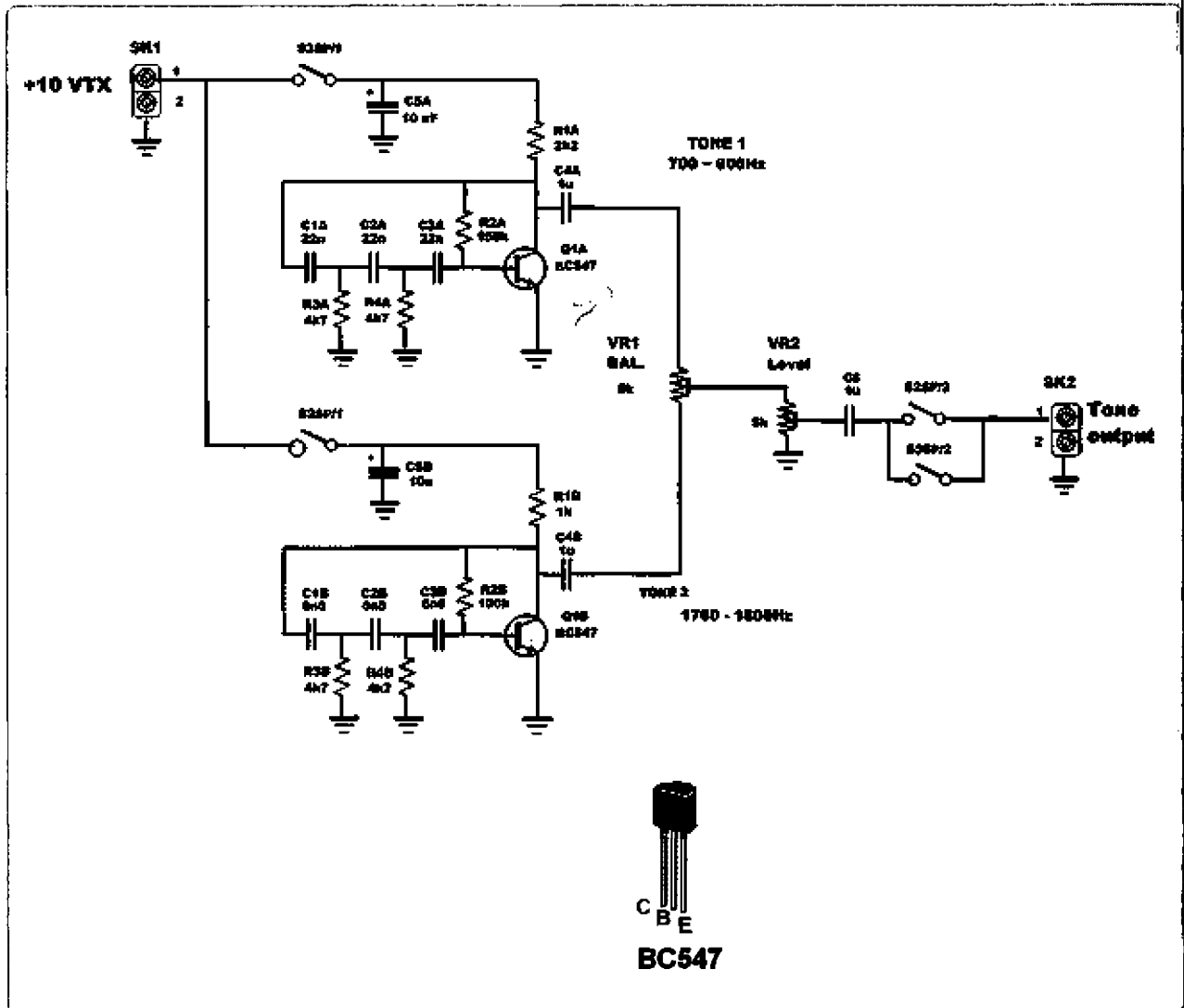
Figure 18: The two-tone oscillator is based on a simple phase-shift network design for each oscillator, each different by about 1 kHz.
