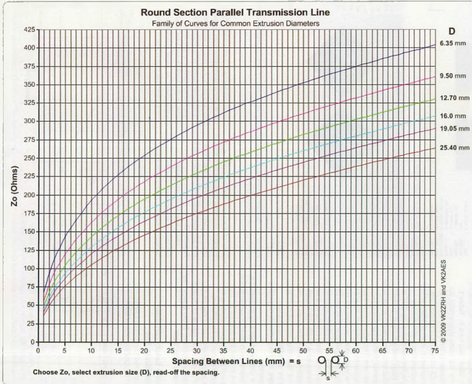
Figure 18. Family of transmission line impedance curves for common round-section lines (rod or tube) with between-line spacings from 1 mm to 75 mm.
