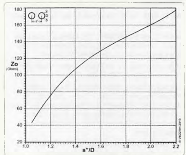
Figure 15. Transmission line impedance – Zo – versus shape ratio ( s''/D ) for close-spaced round-section parallel transmission lines.
