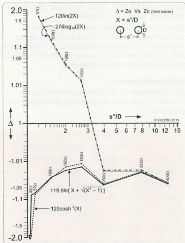
Figure 14. Accuracy of handbook equations (for round-section lines) – Zo – versus calculated results from CST – Zc. The four equations here are those illustrated in Panel A.
