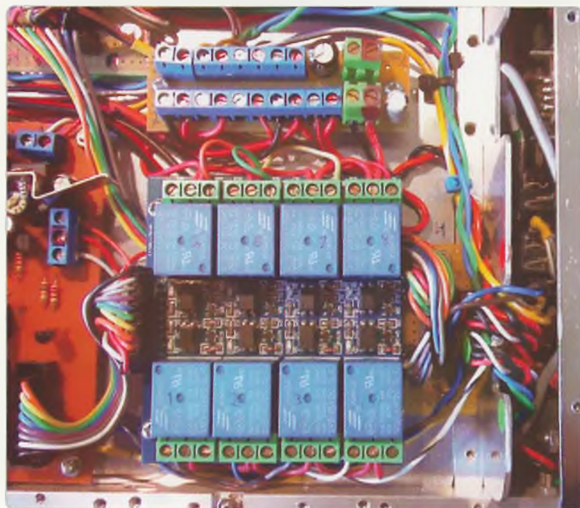
Photo 3HB: The Arduino 8-channel relay board – a module bought on the web.
