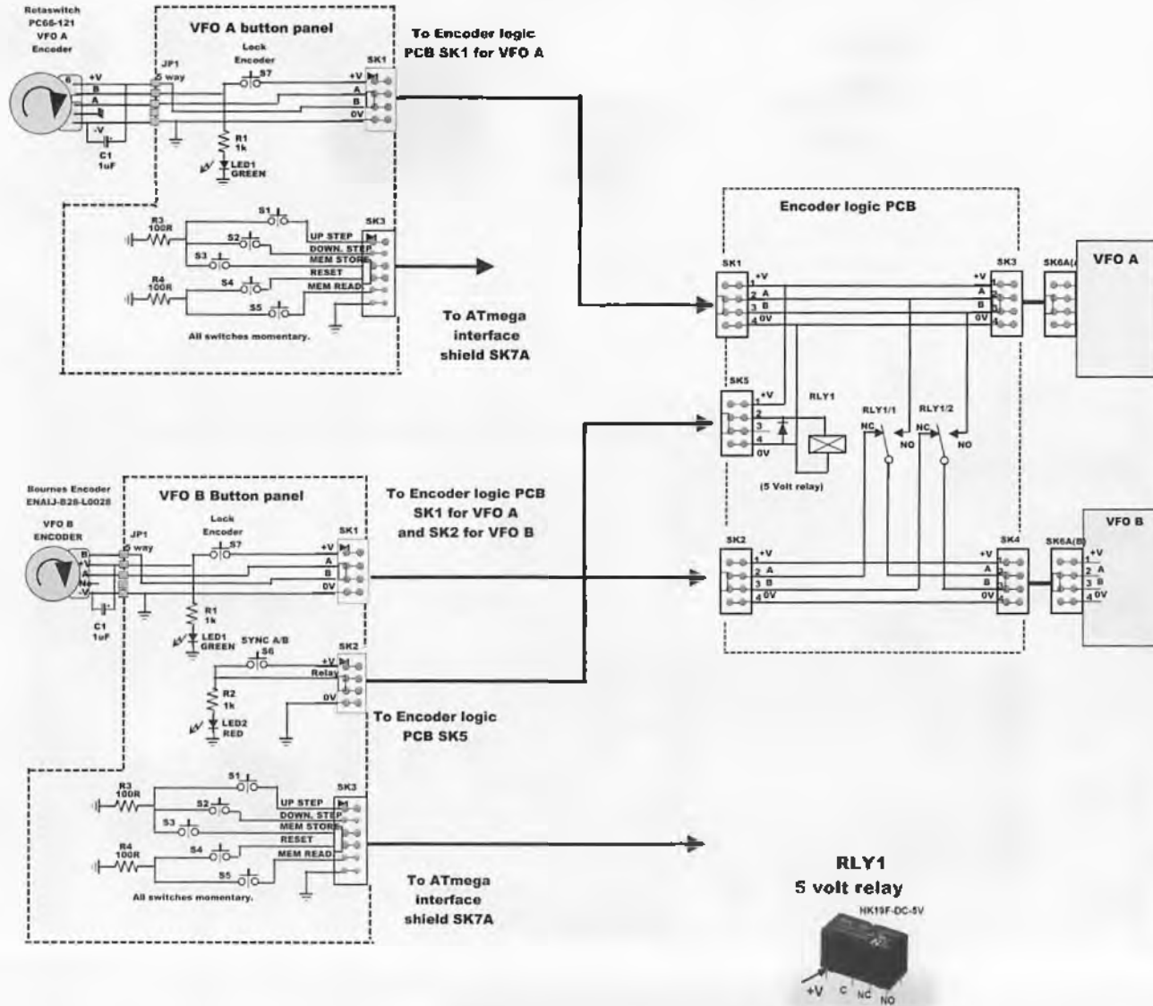
Figure 30. Showing the VFO encoder circuitry and momentary pushbuttons.
