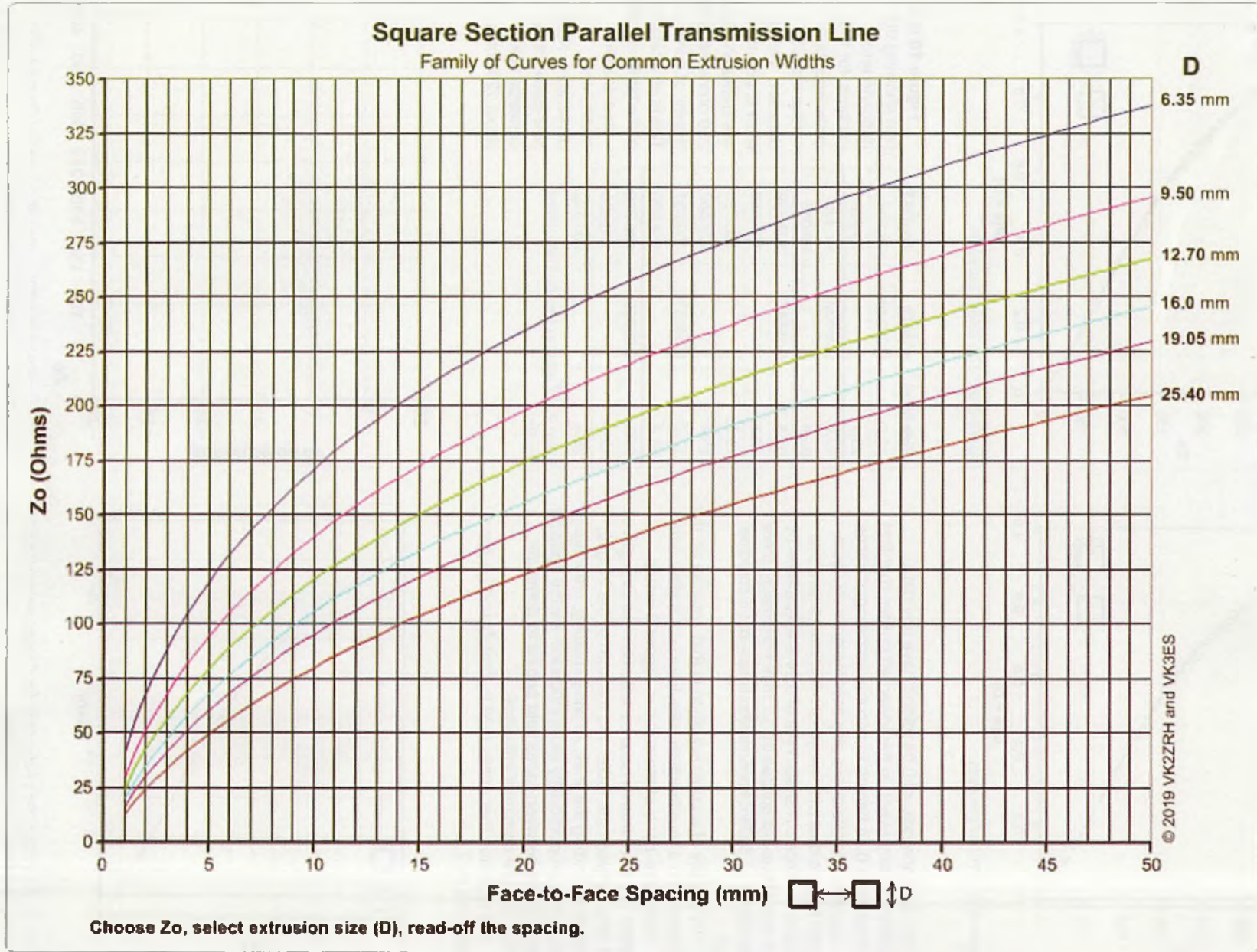
Figure 12. Family of transmission line impedance curves for common square-section aluminium extrusions with face-to-face spacings from 1 mm to 50 mm.
