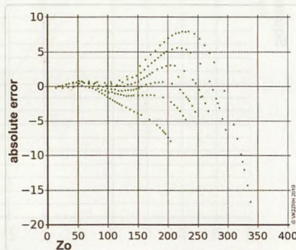
Figure 10. Absolute error, curve-fit Zo versus Zo data from CST tables, for square-section lines.
