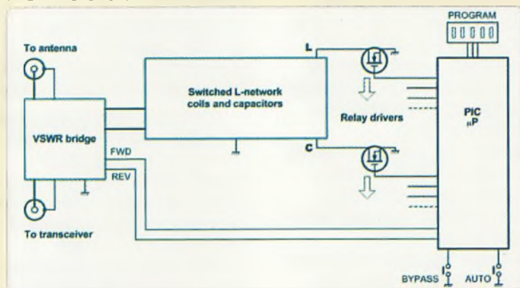
Generic auto-matcher block diagram.
