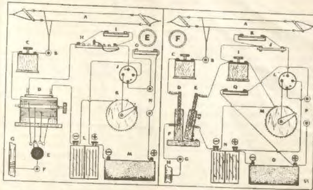
A. Aerial; B. Aerial Terminal; C. .0005 Mfd. variable condenser; D. Vario-coupler; E. Multiple switch; F. Earth Terminal; G. Earth; H. Variable grid leak; I. Grid condenser; J. Valve; K. Filament rheostat; L. Accumulator or low tension battery; M. High tension battery; N. Phone terminals; O. Phone condenser.
