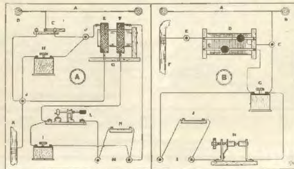
A. Aerial; B. Insulators; C. S.P.D. F. Switch; D. Aerial terminal; E. Primary coil; F. Secondary coil; G. Coil support; H. .0005 Mfd. variable condenser; I. .0003 Mfd. variable condenser; J. Earth terminal; K. Earth; L. Crystal detector; M. Telephone terminals; N. .002 or .003 Mfd. Fixed condenser.
