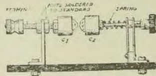
Fig. 6.—The converted Perikon detector.
