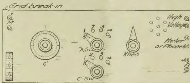
Fig. 2. Suggested Panel Layout
