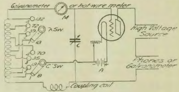
Fig. 1. Wave-meter Wiring Diagram
