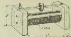
Fig. 2.—The finished potentiometer.
