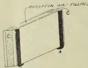
Fig. 10.—Finished condenser.
