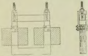
Fig. 77. A choke suitable for its experimental inductance may be inserted over a wide range by moving the top tooth of the core which is mounted so that it may be slipped between the brass end pieces.
