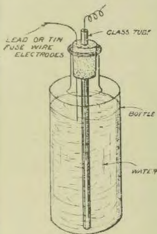
Fig. 8.—The completed resistance.
