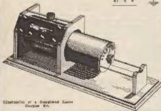
Illustration of a Douglas's Lark Crystal Set.
