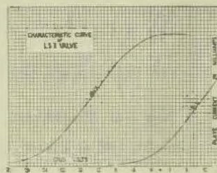
L.S.3 VALVE.
