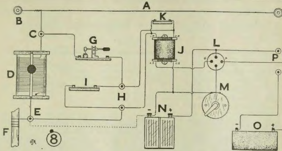
A. Aerial, B. Insulator, C. Aerial terminal, D. Tuning inductance, E. Earth Terminal, F. Wave-pipe earth, G. Crystal detector, H. Phone terminals of crystal circuit, I. Phone condenser, J. L.F. Interstage transformer, K. Fixed condenser shunting primary winding, L. Valve, M. Filament rheostat, N. accumulator, O. High-tension battery, P. Output to H. K. telephones.
