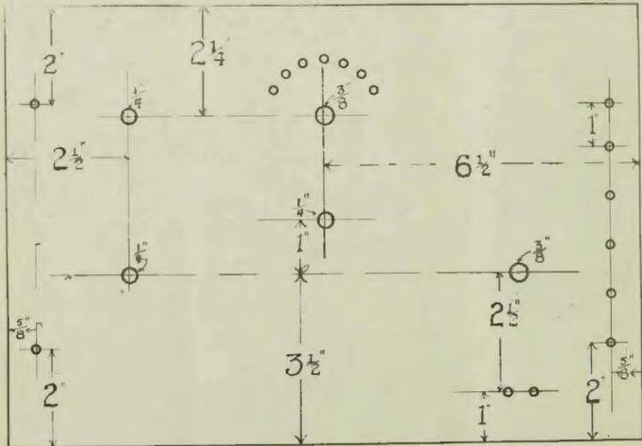
Panel Layout Fig 4
