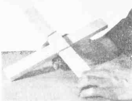
The instructions for building the indoor pusher tell you that the wing is held to the motor stick by a single rubber band. If that statement puzzled you, glance at this picture. See how the single band holds two sticks together? Imagine that the upper stick is your wing and the lower the motor stick, and your bewilderment will be over.
