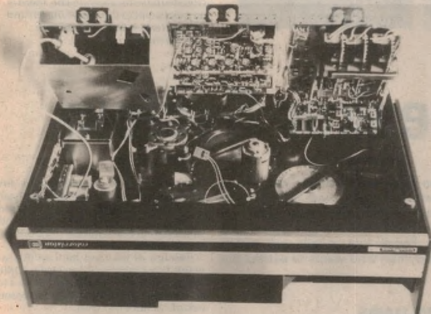
The underside of the Colorvision scanner, showing various sections swung out for easy service access. The main drive motor may be seen slightly left of centre, together with the capstan flywheels.
