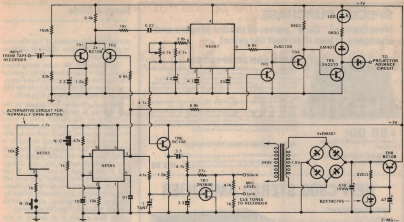
The complete circuit diagram for the Sync-a-Slide automatic slide advance.
