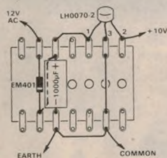
The above photograph, together with the two wiring diagrams given below, should make construction a straightforward process. Note that the front panel is earthed.
