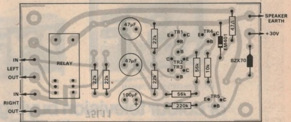
Below is the orientation of the Protector board with respect to the main PC board.
