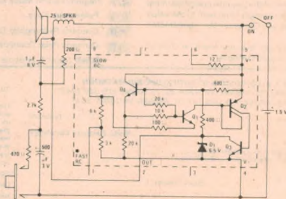
Fig. 2: A "fire siren" oscillator circuit.
