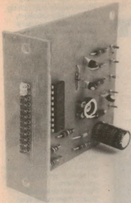
Here is a photograph of the finished unit, showing how the LEDs are mounted at right angles to the main board.
