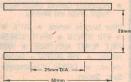
Fig. 4: The inductors can be wound up on bobbins made to these dimensions from plywood, masonite or other non-metallic material.
