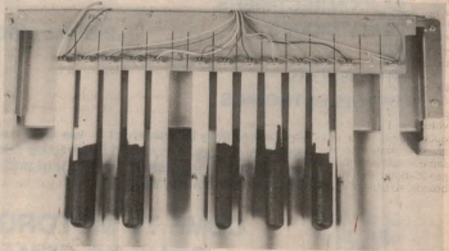
A close-up of the pedal assembly, showing the switches mounted on a slotted strip of epoxy fibreglass. Details of the strip are shown above.
