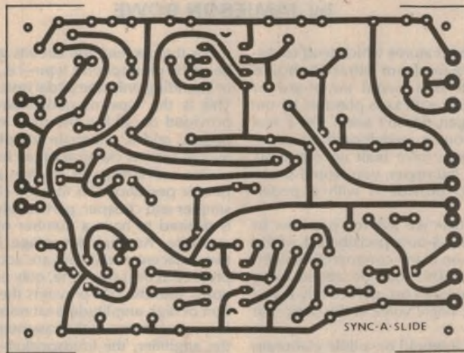
At top is the component overlay pattern on the PC board, viewed from the component side. Directly above is an actual size reproduction of the PC pattern.
