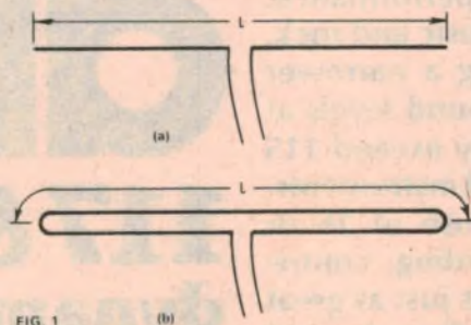
FIG 1 Basic resonant aerials: a simple dipole (a) and a folded dipole (b). The dimension "L" should be 5% less than a half wavelength at the desired operating frequency.
