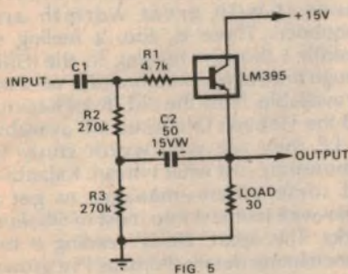
FIG 5 An emitter follower with a very high input impedance.
