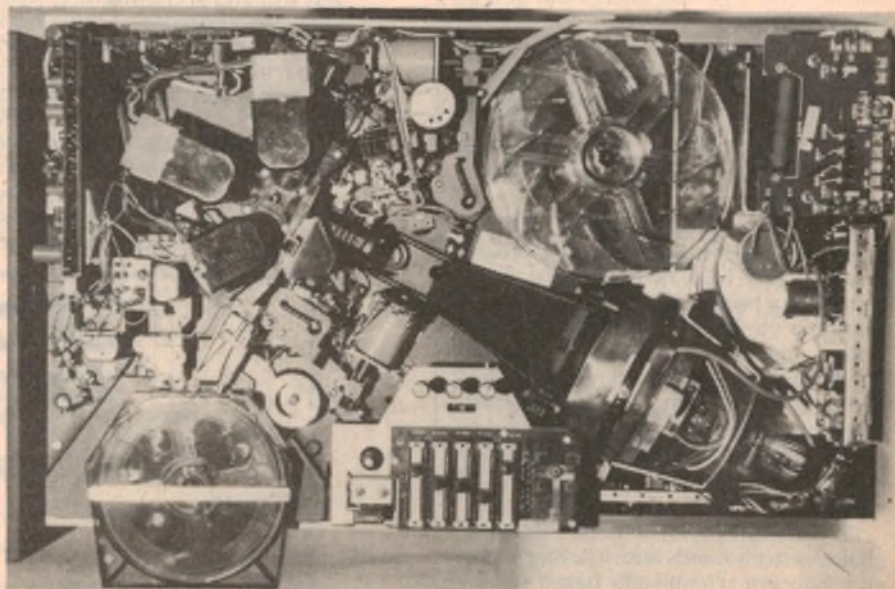
The operating deck of the Colorvision CCS 8mm flying spot scanner. The cassette is in the bottom left hand corner and the takeup spool at top right. The CRO and photomultiplier housings are clearly visible. See diagram on next page.
