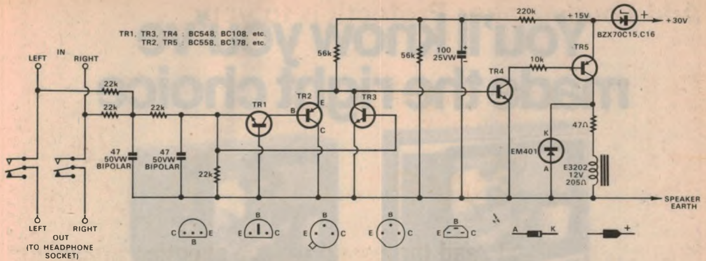
EA LOUDSPEAKER PROTECTOR (PLAYMASTER TWIN TWENTY FIVE)
