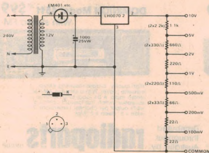
DC VOLTAGE REFERENCE
