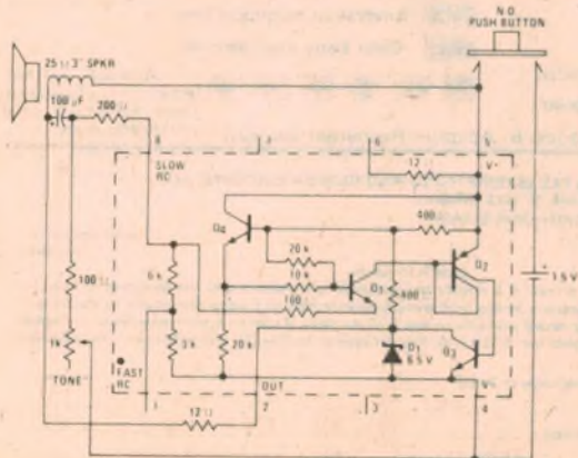
Fig. 1: An electronic "trombone" game.
