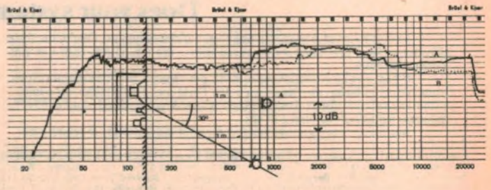
Curve A: Axial pressure response frequency characteristic measured as per DIN 45500. Curve B: Corresponding curve measured 30° from axis (normal listening direction by stereo).
