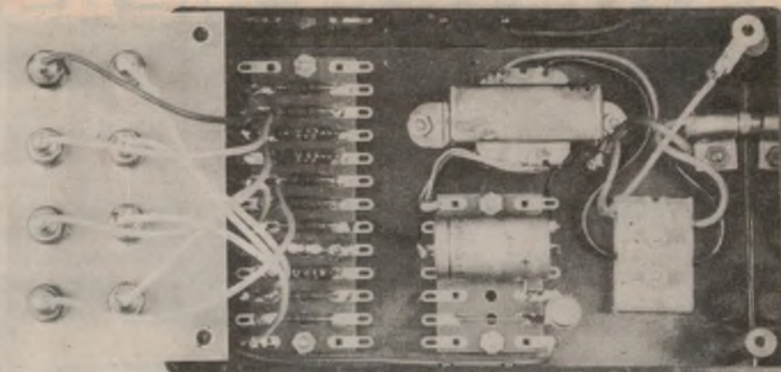
The above photograph, together with the two wiring diagrams given below, should make construction a straightforward process. Note that the front panel is earthed.
