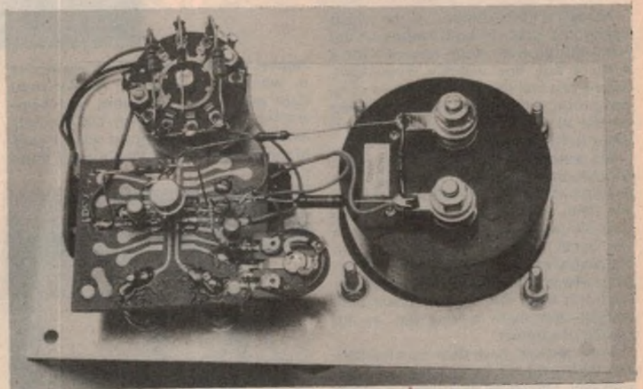
This photograph clearly shows the internal construction of the ohmmeter. The 741 IC and associated components are mounted on the DIP board, with other components strung across the switch wafer and to the meter terminals.
