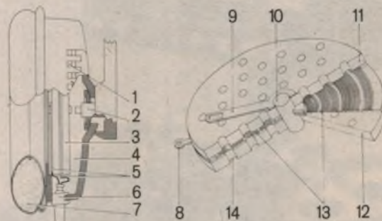
1. Air holes 2. Ball joint suspension 3. Drive unit 4. Damping material 5. Terminals 6. Cable grip 7. Ear pads 8. Terminal 9. Terminal 10. Centre axle 11. Magnet 12. Magnet 13. Diaphragm/voice coil 14. Hole in magnet.
