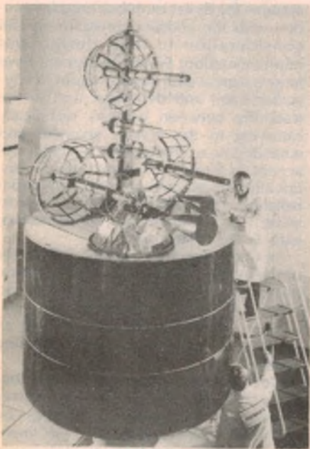
A Marisat satellite before launch. The unusual antenna design allows both US Navy and merchant marine vessels to communicate to shore bases.
