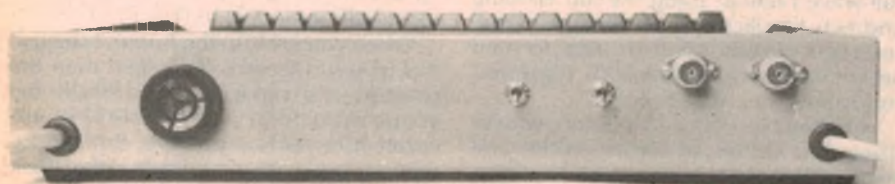
This view of the rear of the terminal shows the audio alarm, two small toggle switches for terminal-TV typewriter switching, and the output connectors.
