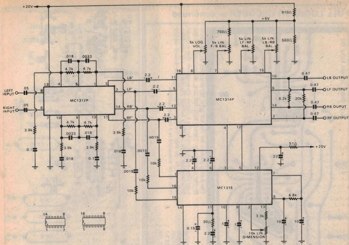
The circuit diagram of the basic decoder/logic system, issued by Motorola Semiconductor Products Inc, who manufacture the ICs under licence to CBS, owners of the SQ trademark. Limited stocks of the ICs are held in Australia by Motorola
