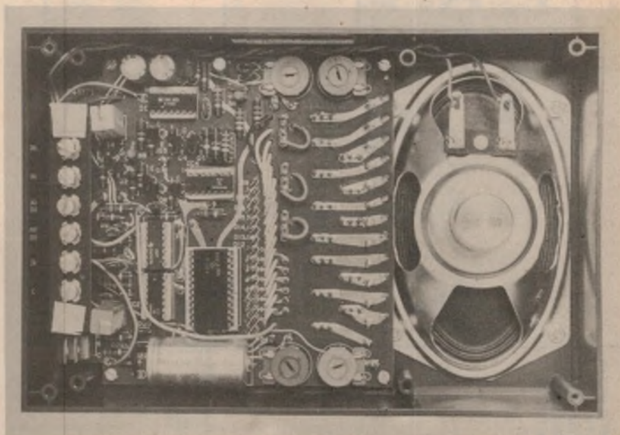
All components are accommodated on a single PC board. The four preset pots are for setting the volume, tuning, speed and decay characteristics.
