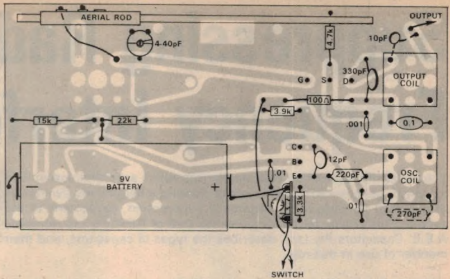
The component layout shows the PC board viewed from the component side. A full-size reproduction of the PC pattern was published in the January issue.
