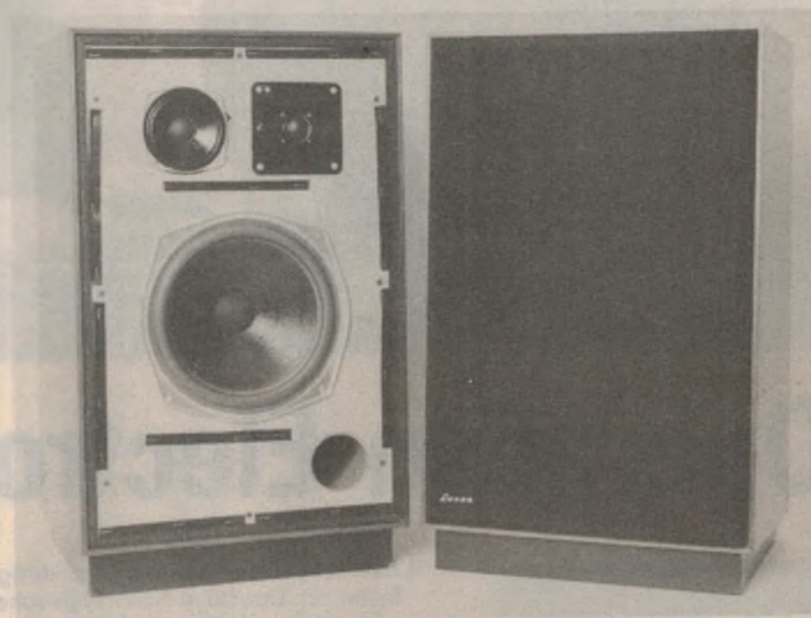
The panels of this Luxor system are angled slightly to reduce internal reflections.
