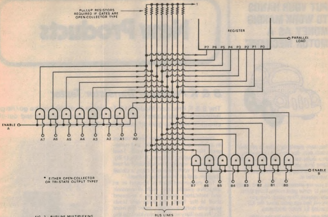
FIG. 7 - BUSLINE MULTIPLEXING
