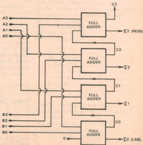
FIG. 4: 4-BIT PARALLEL ADDER
