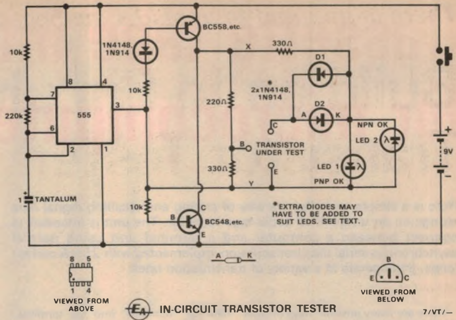
The circuit is basically a 3Hz oscillator with complementary outputs.
