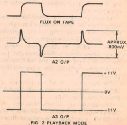
FIG. 2 PLAYBACK MODE
