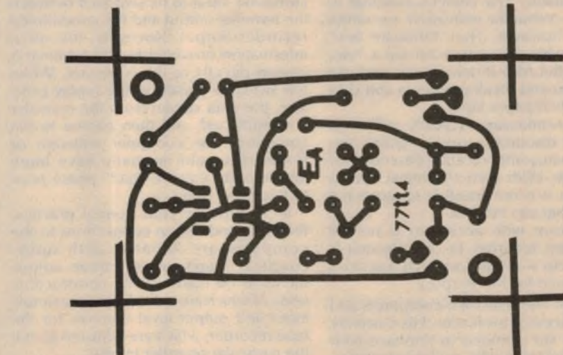
The circuit is basically a 3Hz oscillator with complementary outputs.
