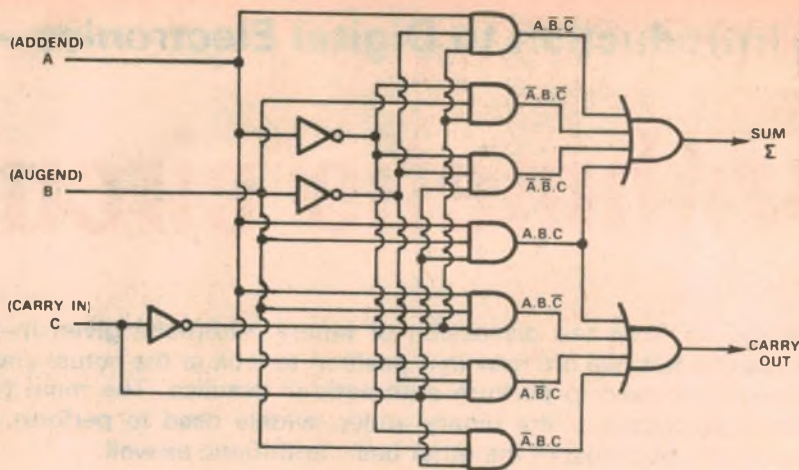
FIG. 2: FULL ADDER
