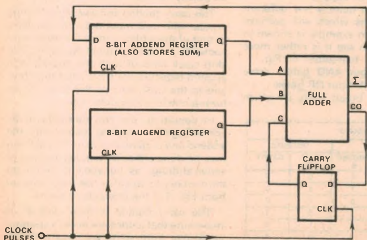
FIG. 3: 8-BIT SERIAL ADDER
