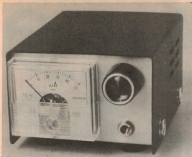
Our prototype SWR meter, housed in a standard commercial case. Meter calibrations are shown on the following page.
