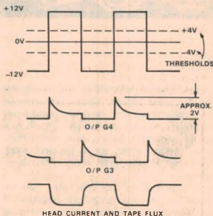
FIG. 1 RECORD MODE
