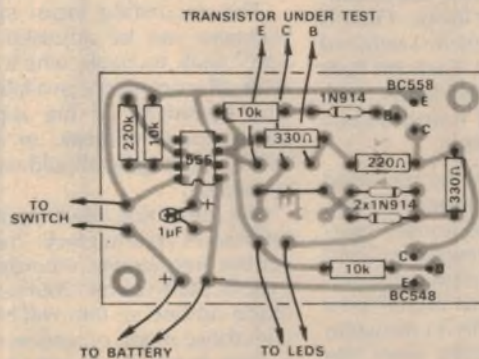
Above is the PC pattern, actual size. At left is the component layout.
