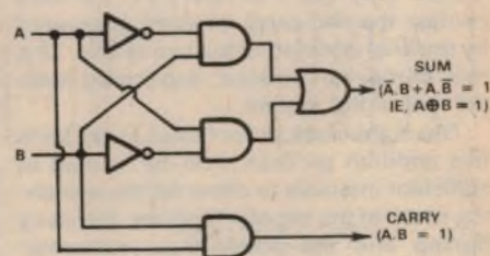
FIG. 1: HALF ADDER CIRCUIT
