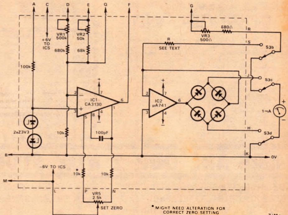
The modified circuit for the active part of the multimeter. A CA3130 FET-input op amp replaces the original discrete FET and 741 input IC, while the meter is now switched for AC and DC.
