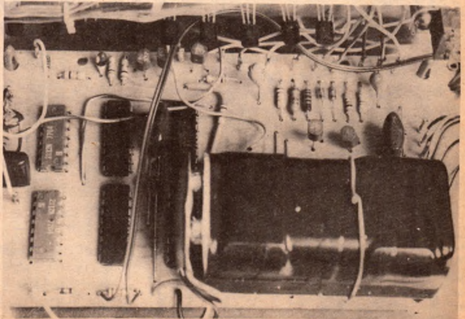
This photograph shows how the battery assembly is secured to the PCB. Note the additional components.
