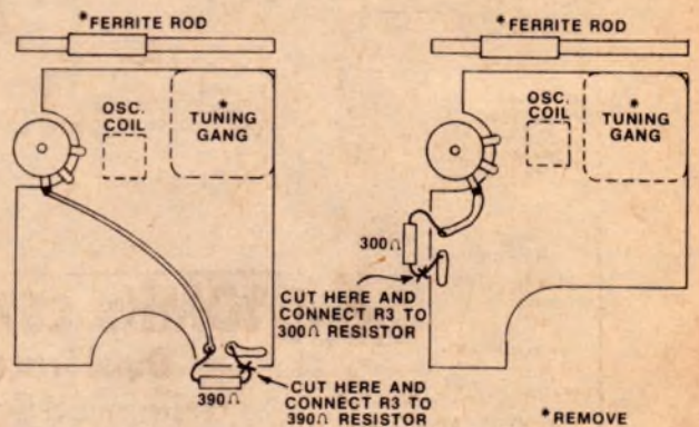
These two wiring diagrams show the modifications necessary to the two different model K-Mart transistor radios.
