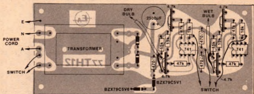
The component overlay diagram shows the PC board from the component side.
