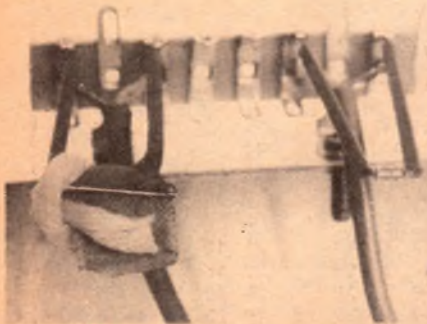
The set up for the wet "bulb". The small piece of cloth around the diode is kept wet by water drawn from the reservoir via the wick.
