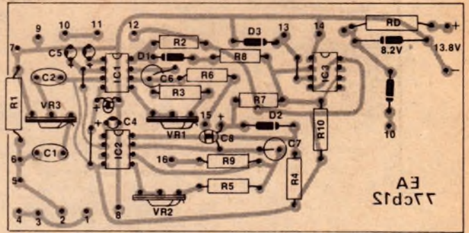
The component layout shows the PCB from the component side. Ensure correct polarity of polarised components.
