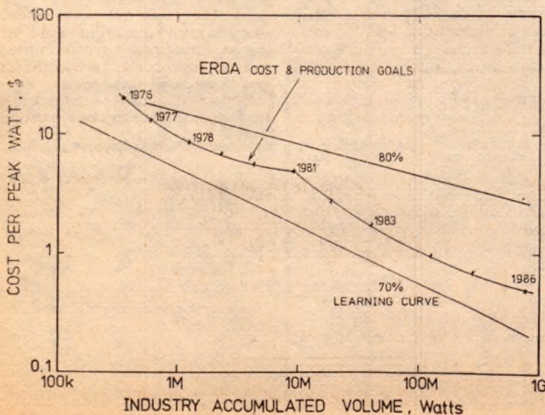
◀ Fig. 1: The ERDA cost and production goals. Shown is the manner in which the cost of solar cell arrays is expected to decrease as the volume produced increases. The goal: to produce arrays costing 50 cents per peak watt output by 1986.
