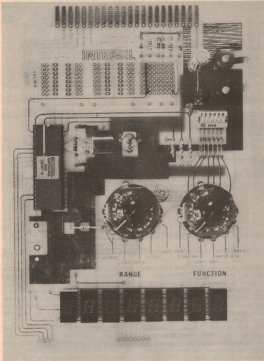
When assembled the PCB looks like this, with a breadboarding area at the top of the PCB.
