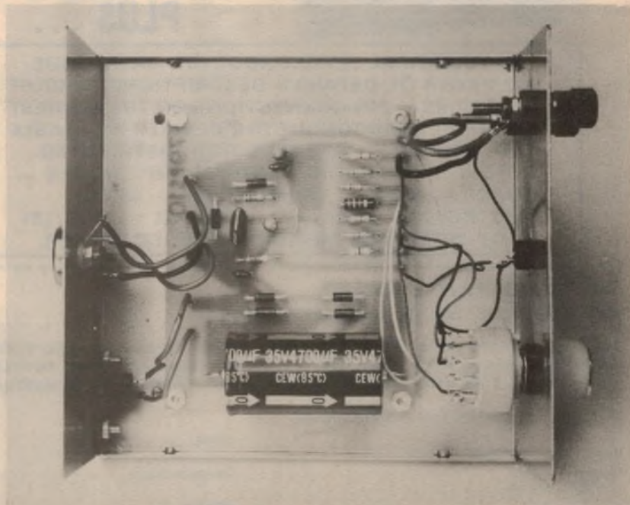
Inside the completed prototype. Note the heavier wiring between the PCB and the AC input socket, the regulator IC and the terminal posts on the front panel.
