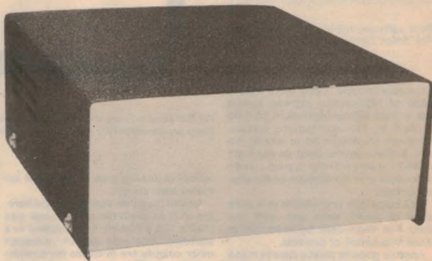
Above: The "deluxe metal cabinet" as sold by Dick Smith Electronics. It makes an ideal case for the 30V 2A regulated power supply shown below.
