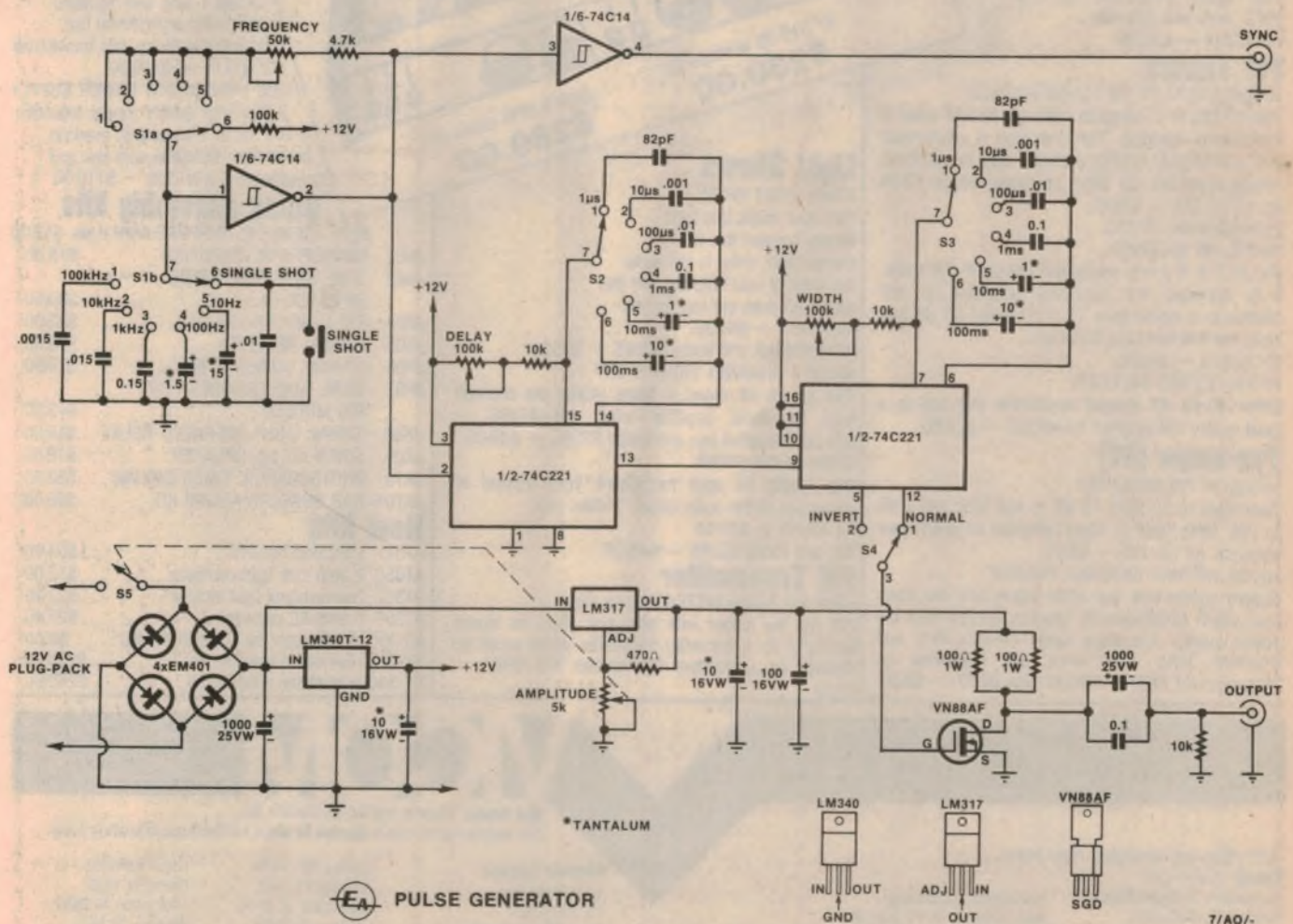
At the top left is the Schmitt trigger oscillator, followed by the delay circuit and the width circuit. At the lower right is the VMOS output stage which is largely responsible for the generator's high performance.
