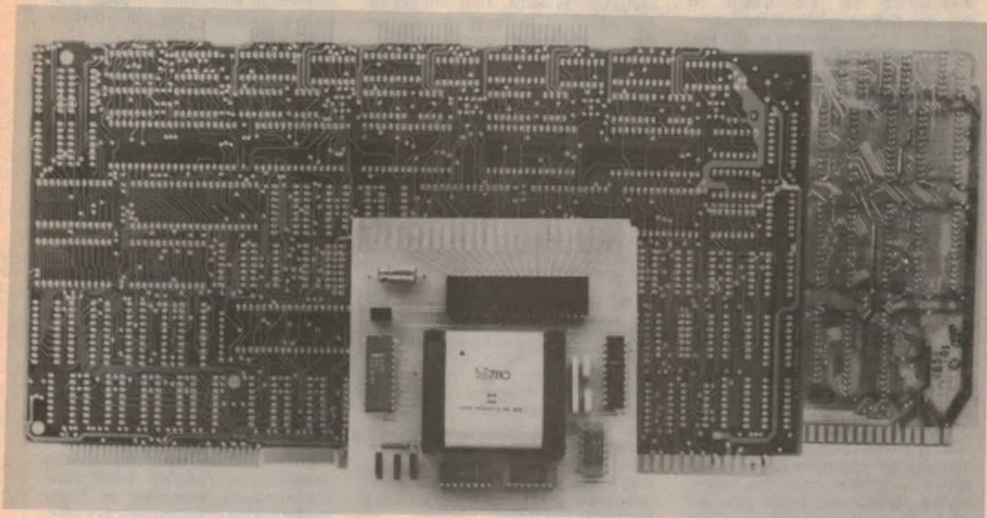
Space saver — new Intel 7110 MBM device and supporting LSI family reduce space and component count for a 1-megabit bubble system by an order of magnitude, replacing two PC boards, four 256K modules, and about 85 ICs.
