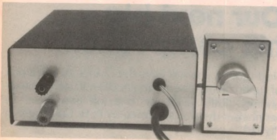
Here is the completed control unit, built into a standard metal case. A separate hand-held plastic case is used to house the speed control potentiometer.
