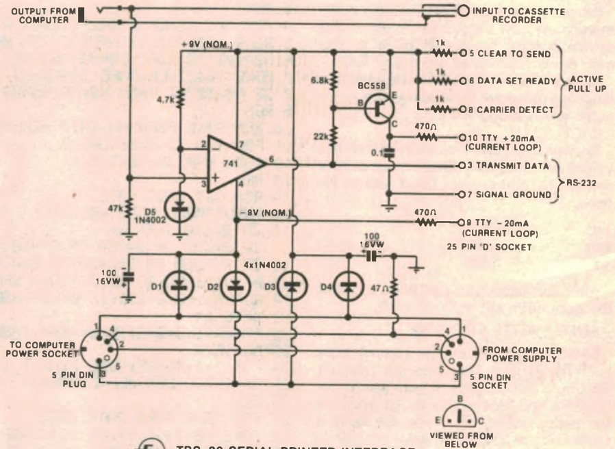
EA TRS-80 SERIAL PRINTER INTERFACE
