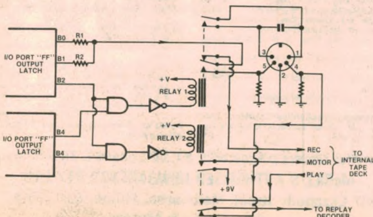
FIG. 2: SYSTEM-80 CASSETTE INTERFACE
