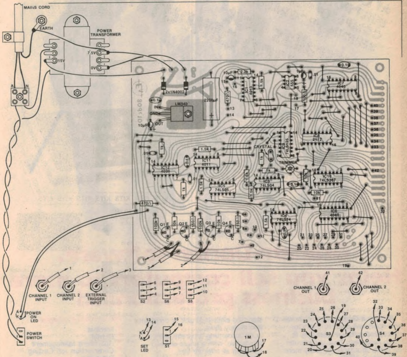
Follow this wiring diagram in conjunction with the circuit on p55. The PC board is shown from the component side.
