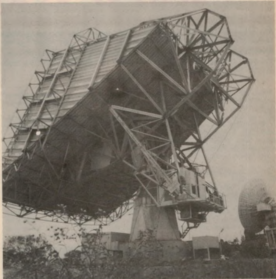
The Cassegrain horn antenna at Carnarvon, WA. Major modifications have been made to the antenna so that it can monitor the new Intelsat Series V satellites.
