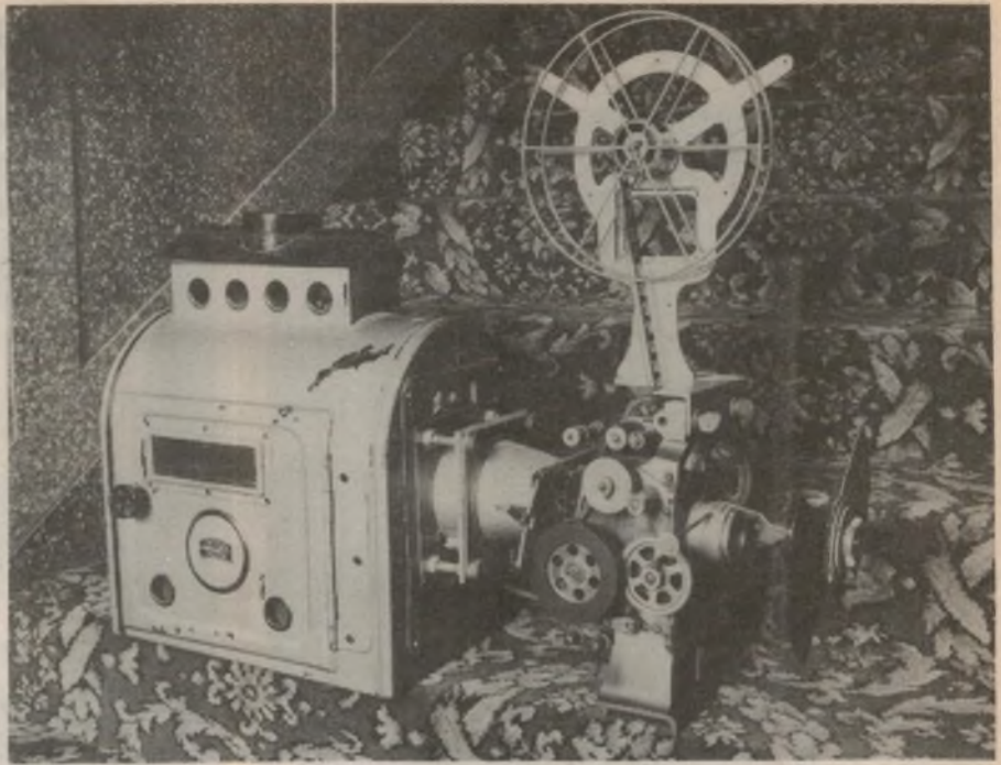
A 1912 Powers Bioscope projector. The extensive ventilation arrangements indicate that this projector was originally a "lime-burner", illuminating the film with an acetylene lamp, although this unit was subsequently converted to use a carbon arc lamp. Some later model Powers projectors were also converted for use with sound films by adding a sound head underneath the projector body.
