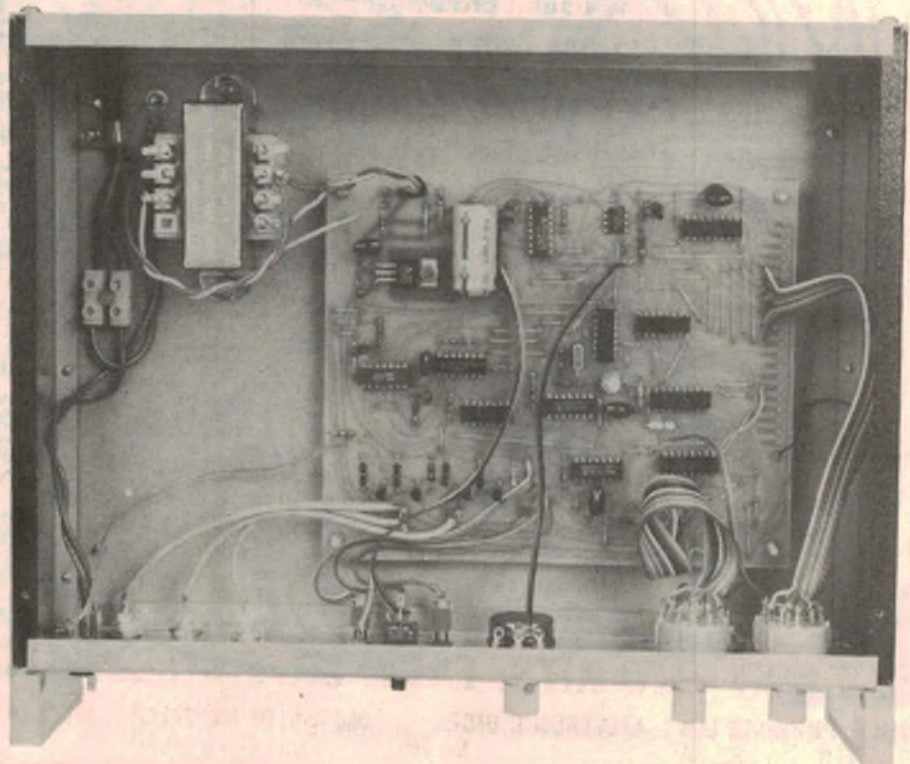
ABOVE: the Digital Storage CRO Adapter at work, capturing and displaying ASCII codes. BELOW: inside the prototype.
