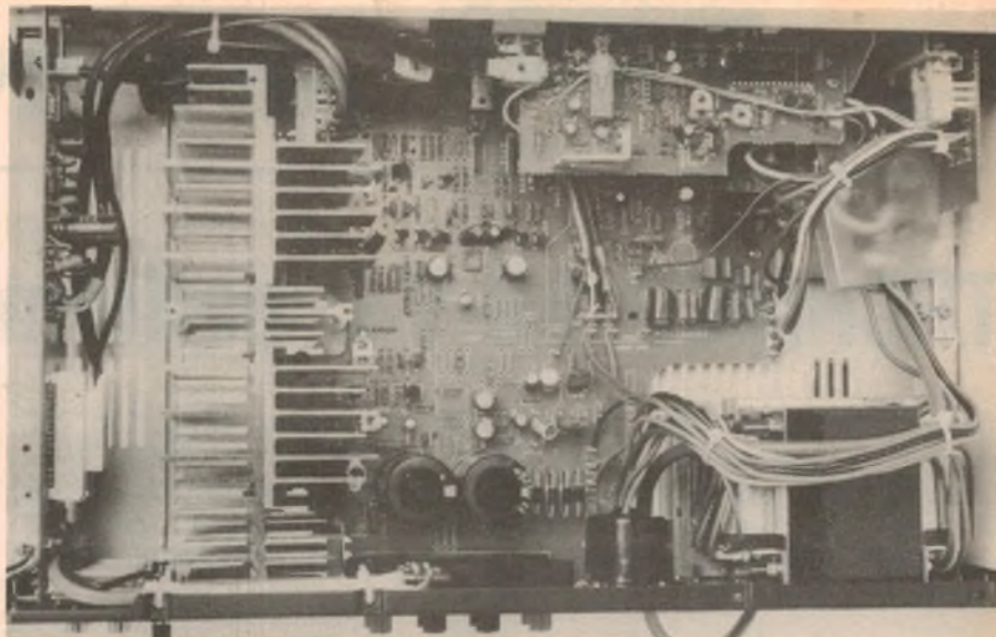
Above: An inside view of the Technics SU-V4 amplifier, looking down from the rear. Note the very large internal heat sink. Below is a plot of the THD at full rated power; but note that the distortion scale is from 0 to 0.1%. The rated figure is 0.02%.
