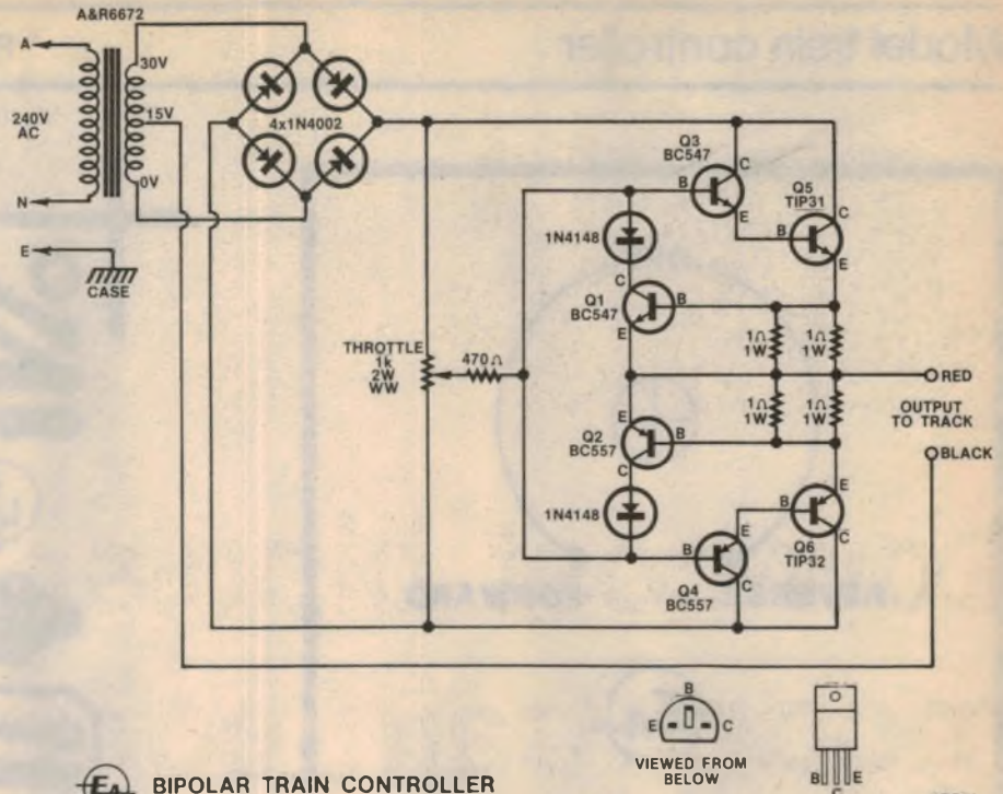
BIPOLAR TRAIN CONTROLLER
