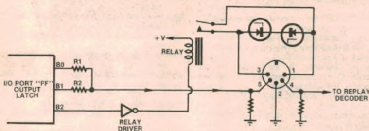
FIG. 1: TRS-80 CASSETTE INTERFACE
