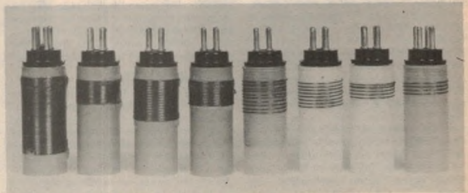
Eight plug-in coils are used to cover the frequency range from 0.5 to 30MHz. Full winding details for the coils are given in the text.
