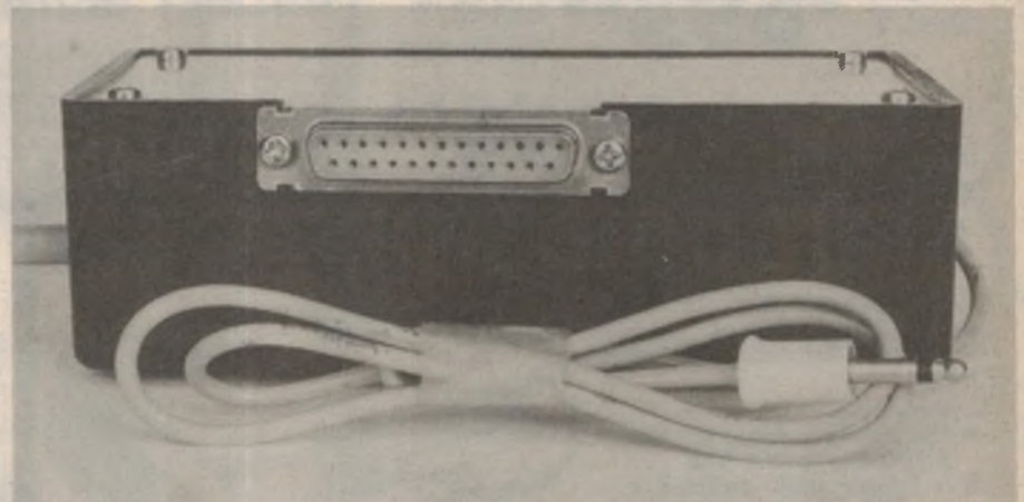
The unit is designed to plug straight into a standard printer with an RS232 interface input. A 20mA current loop interface is also provided.
