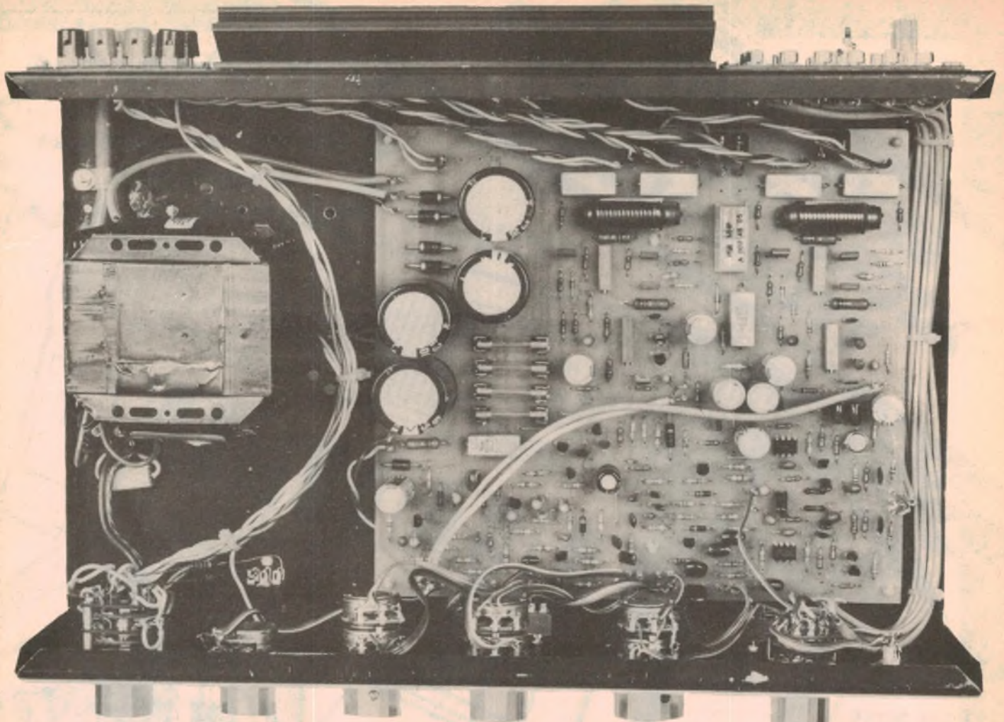
This photo shows the internal layout of the amplifier with the optional Ferguson transformer which is fitted with a copper strap to reduce hum radiation to a minimum.
