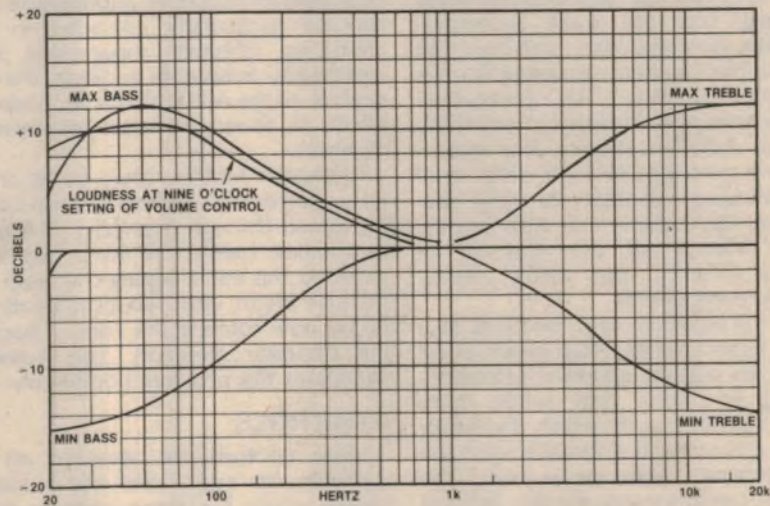
Above is a set of curves showing the distortion performance of the amplifier while below are the tone control and loudness characteristics.
