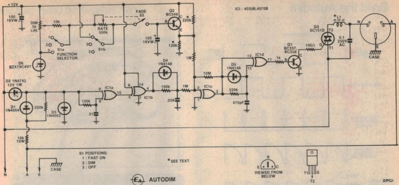
Variable light dimming is achieved by means of a phase-controlled Triac power control circuit.
