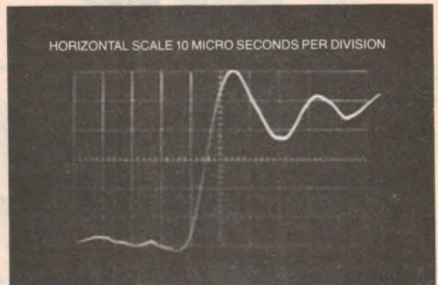
Actual unretouched oscilloscope photograph showing rise time of 980LZS using CBS STR112 record.
