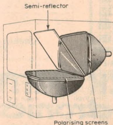
Fig. 1: Screens that polarise the image for each eye and polaroid glasses make 3D easy, but are too bulky for the home.
