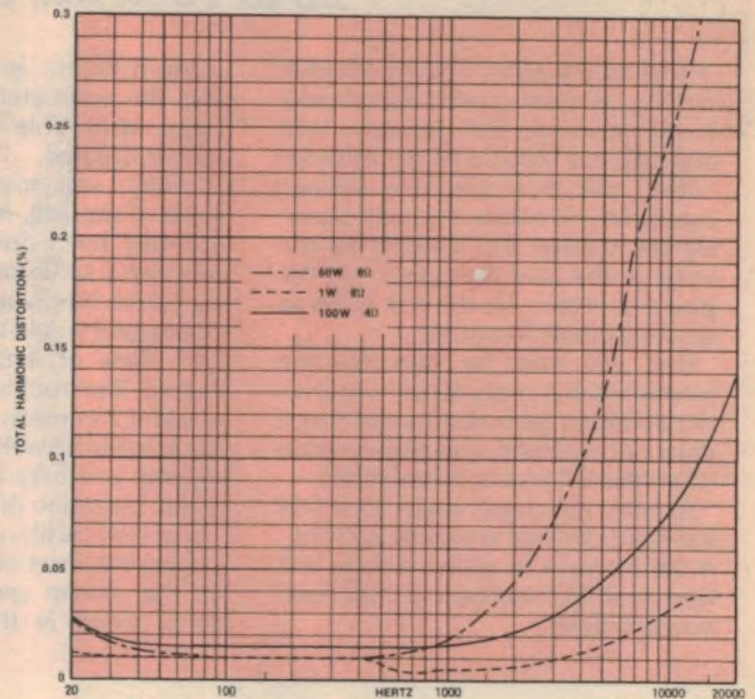
Above is the frequency response curve of the low pass filter stage, while at right are the distortion versus frequency curves for the power amplifier stage.
