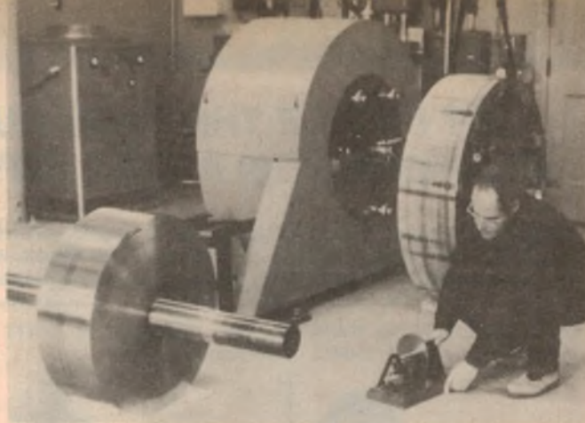
University of Texas' homopolar generator (disassembled). Alongside David Lampe views a model of an 1821 design.
