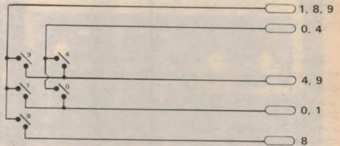
The circuit consists of four LED displays wired in parallel with the existing displays, together with five pushbutton switches wired in parallel with the five most useful function switches.
