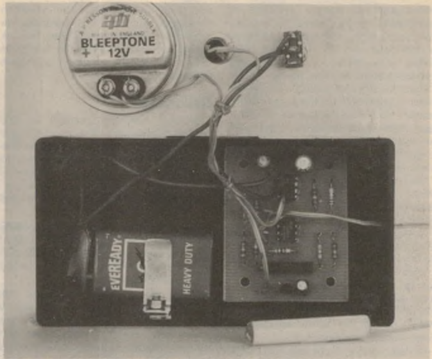
This picture gives a good idea of how the various sections fit together in the plastic box. Note that the battery should be mounted so that it does not foul the piezo-electric buzzer.
