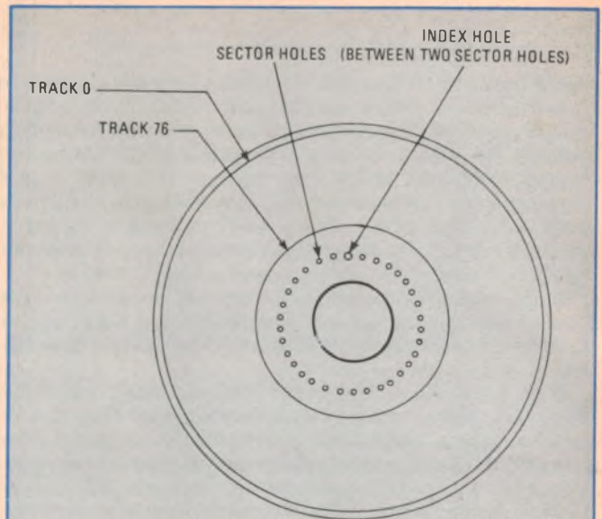
Fig. 4: Hard sectored disks use sector holes.
