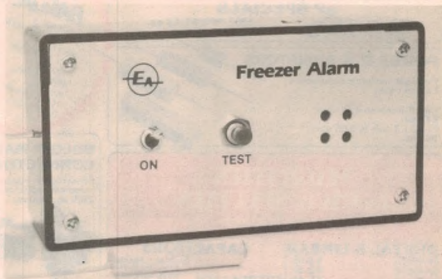
The complete Freezer Alarm is housed in a small plastic box, and the panel we have prepared gives it a professional appearance. The sensing probe, which is normally in the freezer, is shown in front of the box.
