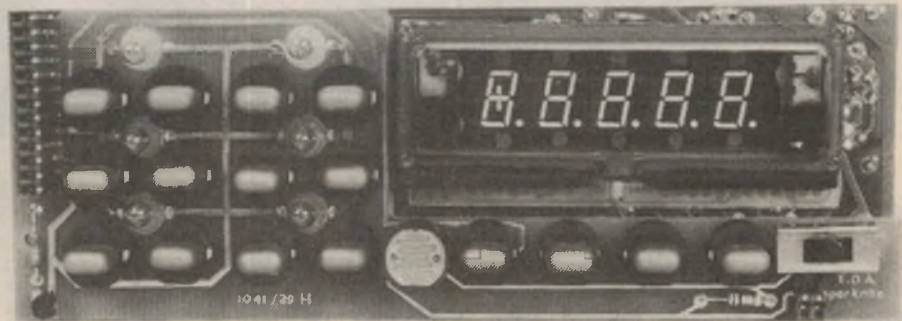
The keyboard and mainboard are sandwiched together by connectors at each end. Six incandescent lamps illuminate the keyboard during night driving.
