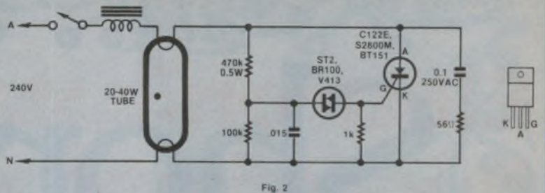
Fig. 2: Circuit diagram for our electronic "instant" starter.
