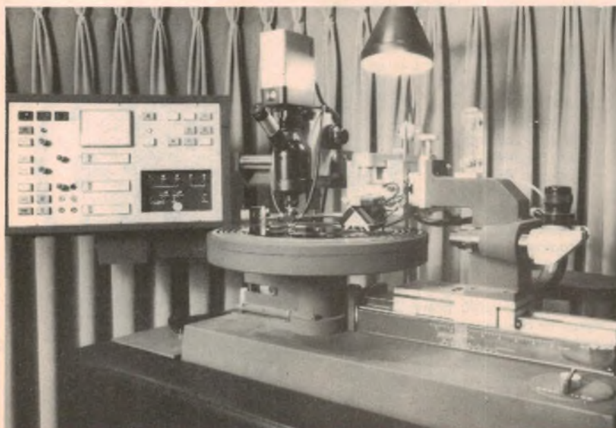
The Neumann VMS-80 recording lathe, the only one of its kind in Australia. Note the optical microscope and the macro TV camera which displays the grooves on a TV monitor screen, normally accommodated on the pedestal at right. The panel (left) is the logic control system for the automatic groove spacing.
