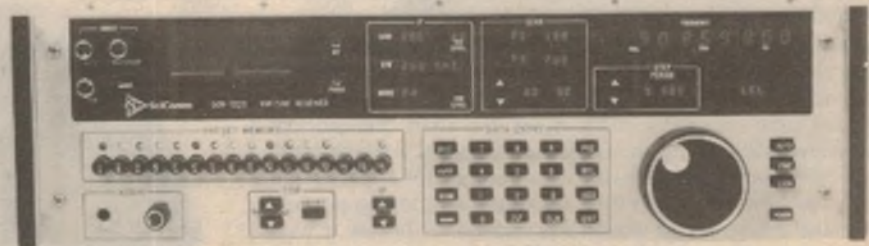
Illustrating the modern trend in communications receivers, this VHF-UHF unit distributed by Vicom International provides program scanning and monitoring functions over a range of 20-1200MHz. It uses a microprocessor to control search and memory functions.
