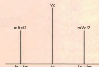
Fig. 2: frequency spectrum of an AM waveform.
