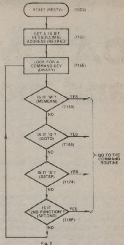
Fig. 3 is a more detailed flowchart of the command routine, showing the actual names and addresses of the individual command routines in the DATUM Monitor ROM.
