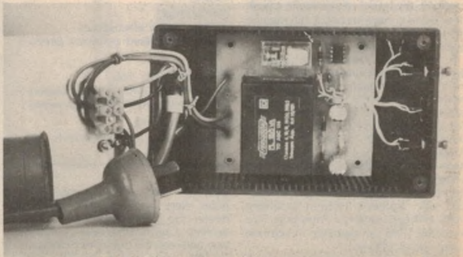
View inside the completed Driveway Sentry. Keep mains wiring neat and tidy, and make sure that you earth the lid of the case.
