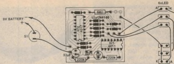
Parts overlay diagram for the Boggle Goggles. Make sure that all polarised components are inserted the right way round (ICs, diodes, LEDs, electrolytic capacitors).
