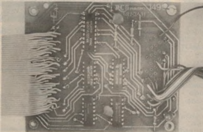
This photograph shows the top side of the parallel interface board. Connection to the TRS-80 is via the 40-way cable at the left of the board.
