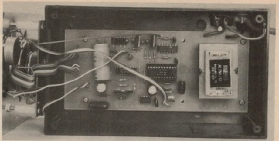
Fig. 1 left, is the overlay of the printer interface board showing connection points to the voice synthesiser unit. Photo above shows the Compuvoice board installed.
