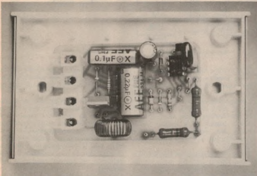
This photograph shows the dimmer circuit mounted on the back of the face plate.
