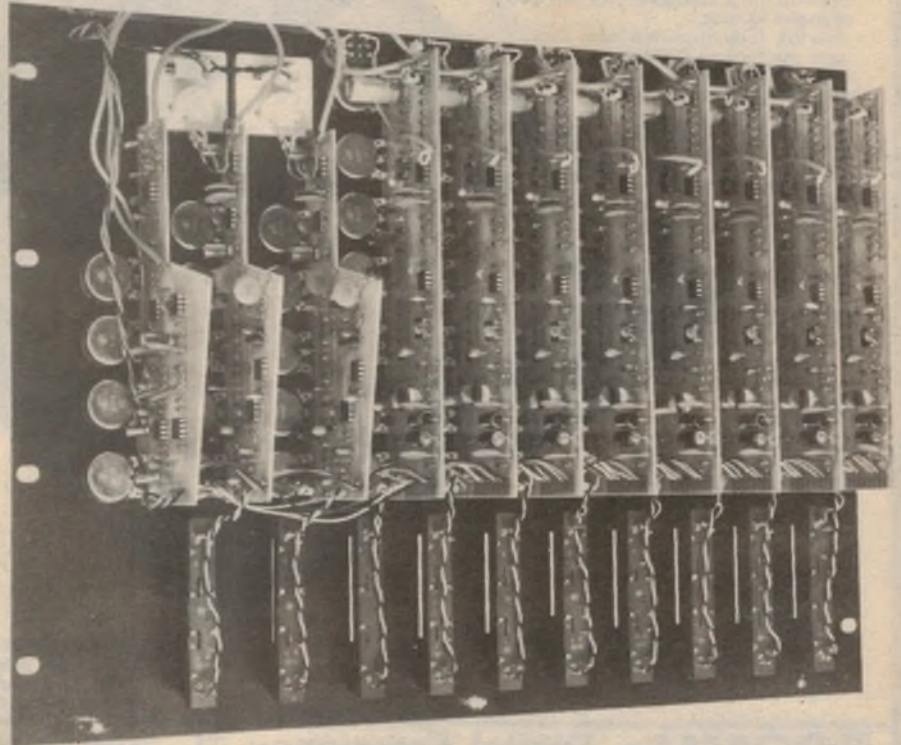
Very little wiring is required for the Mixer and what little there is mostly repetitive. All potentiometers are soldered directly to the PC boards.
