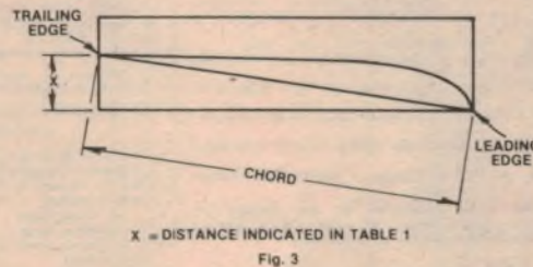
Fig. 2, above, shows the initial shaping of the block from which the propeller is carved. Shaded area must be removed before marking off. Fig. 3 at left shows the dimensions which are referred to in Table 1.
