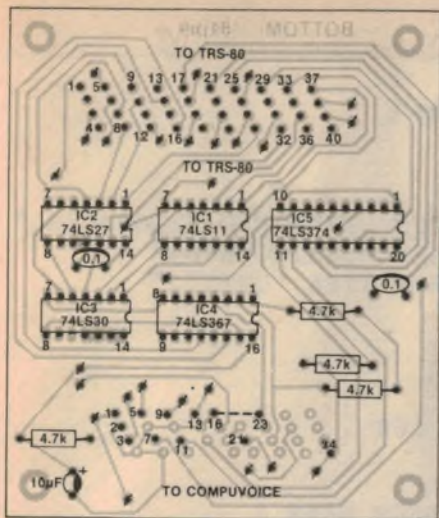
Fig. 1 left, is the overlay of the printer interface board showing connection points to the voice synthesiser unit. Photo above shows the Compuvoice board installed.
