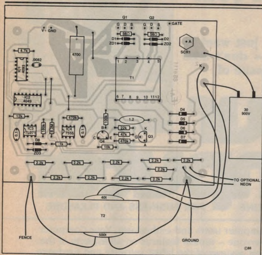
Above: this new wiring diagram shows the parts layout on the corrected PCB pattern. Note the extra link near the 4700 \mu F capacitor.
