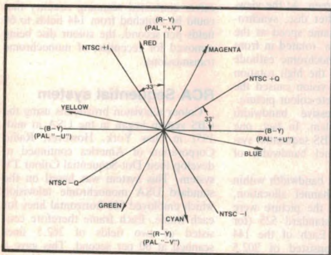
This diagram shows the relative phase angles of the "I" and "Q" signals and the respective colours for NTSC and PAL systems.
