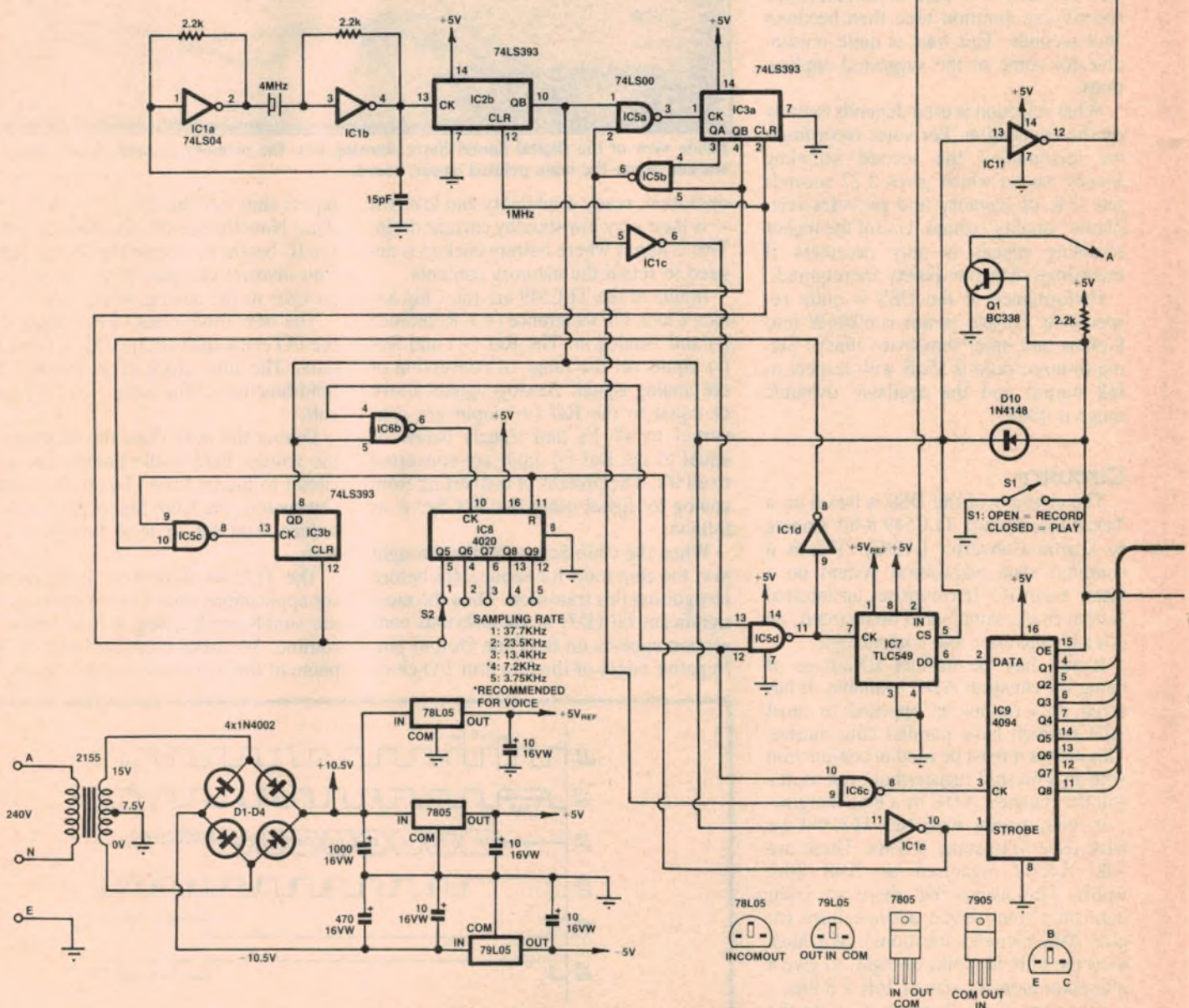
Here is the complete circuit diagram for the Digital Sound Store.
