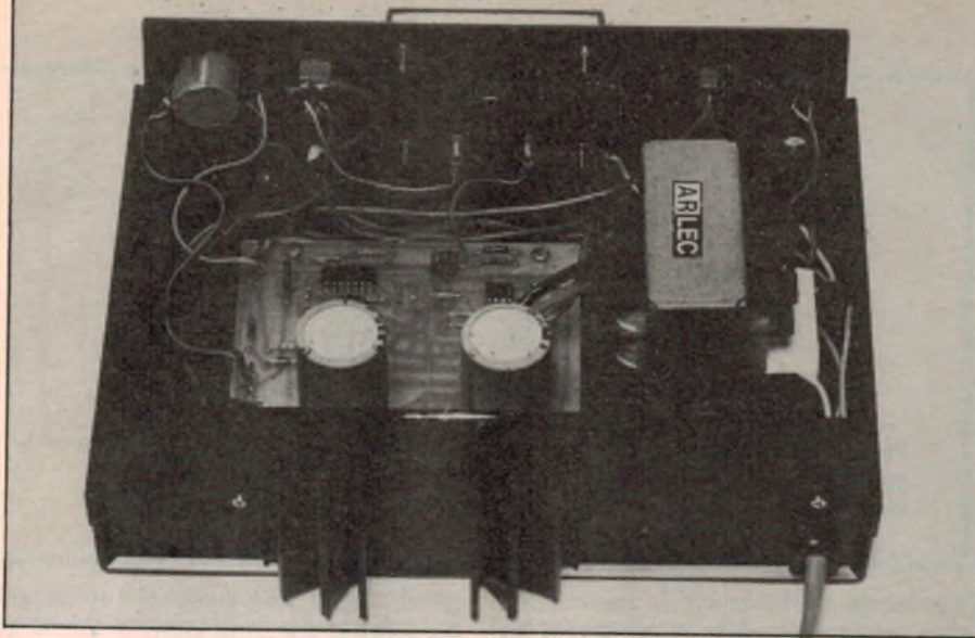
The finned heatsink aids heat dissipation and is secured to the rear panel using the transistor mounting screws. Note that the front and rear panels must be earthed (see Fig.4).
