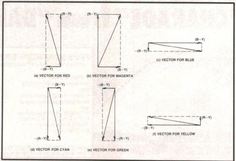
These vector diagrams show the colours produced by relative R-Y and B-Y voltages.
