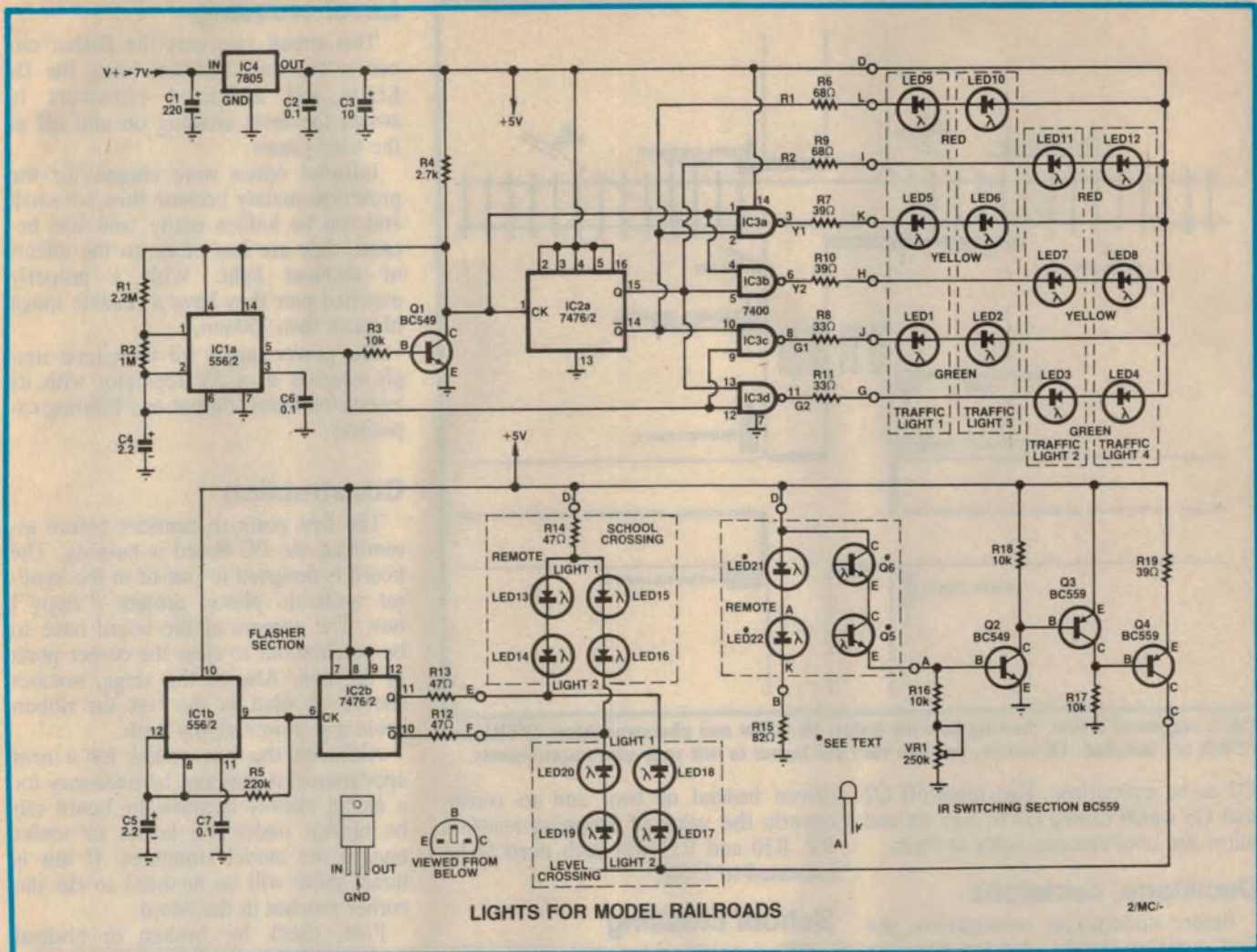
Fig.1: the circuit is built around just four ICs. IC1, IC2 and IC3 drive the various LEDs, while phototransistors Q5, Q6 and the two infrared LEDs switch the level crossing lights on and off as the train passes.
