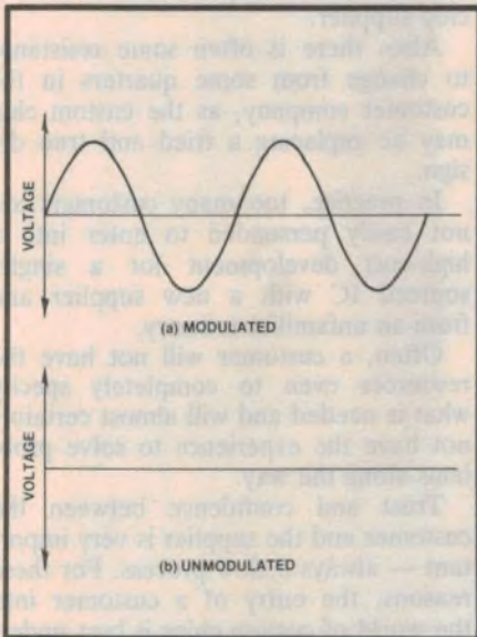
In suppressed carrier modulation, the waveform is present (a) when modulated by signal but absent when modulation is zero (b).
