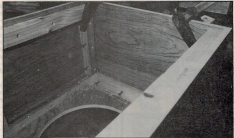
Photo 3: the partly assembled enclosure. Note the use of 45mm square cleats along the inside edges. The cleats should be glued and screwed into position as outlined in the text.
