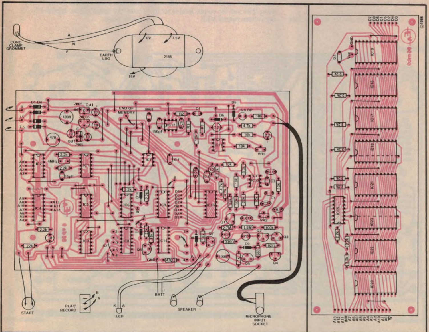
Above is the parts layout and wiring diagram for the main printed circuit board.
