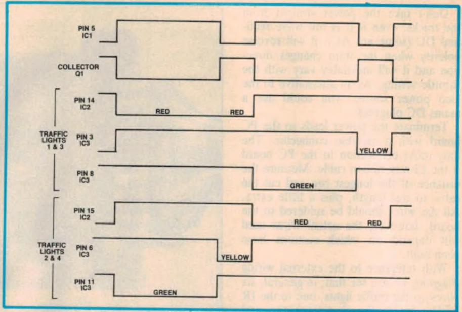
Fig.6: this timing diagram shows the pulse sequence for the traffic lights at various points in the circuit diagram.
