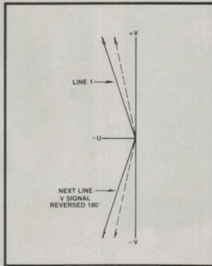
In the PAL system, phase distortion is corrected. The dotted lines show how phase distortion has delayed the red vector, taking it towards magenta. Averaging the phase errors restores the colour to red.
