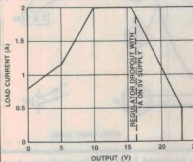
Fig.1: maximum output current vs. output voltage.
