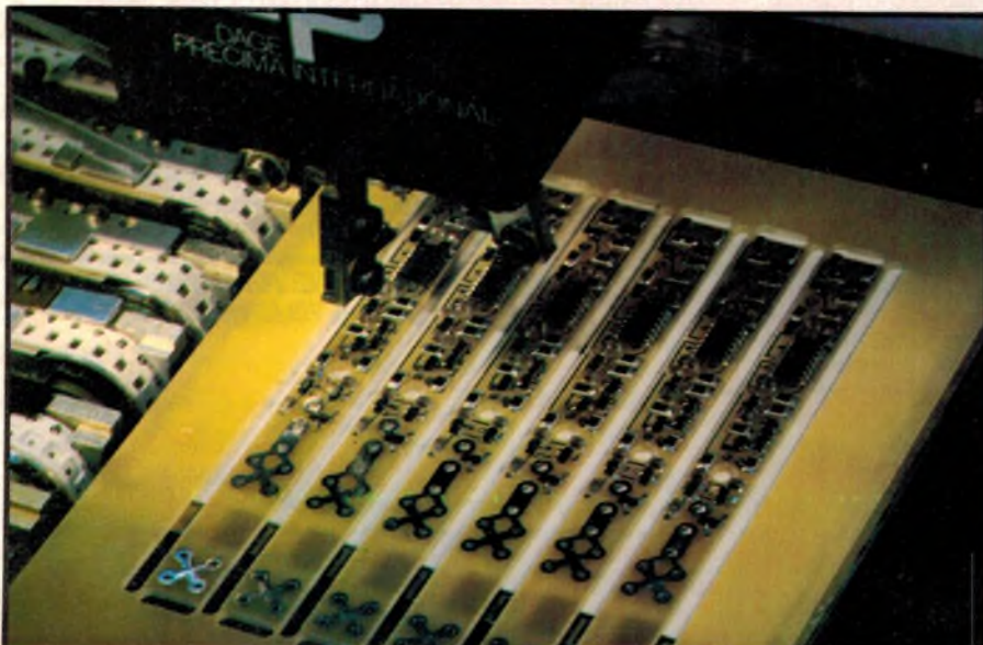
Automatic placement of small components before flow soldering.
