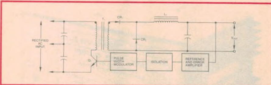
Fig.2: the forward converter is used for powers up to 200 watts.
