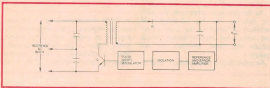
Fig.1: the flyback converter is a popular switchmode supply configuration.
