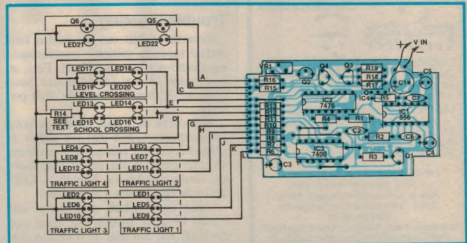
Fig.5: parts layout and wiring diagram. Note that, depending on the options used, R12, R13 and R14 may have to be replaced by wire links (see text).
