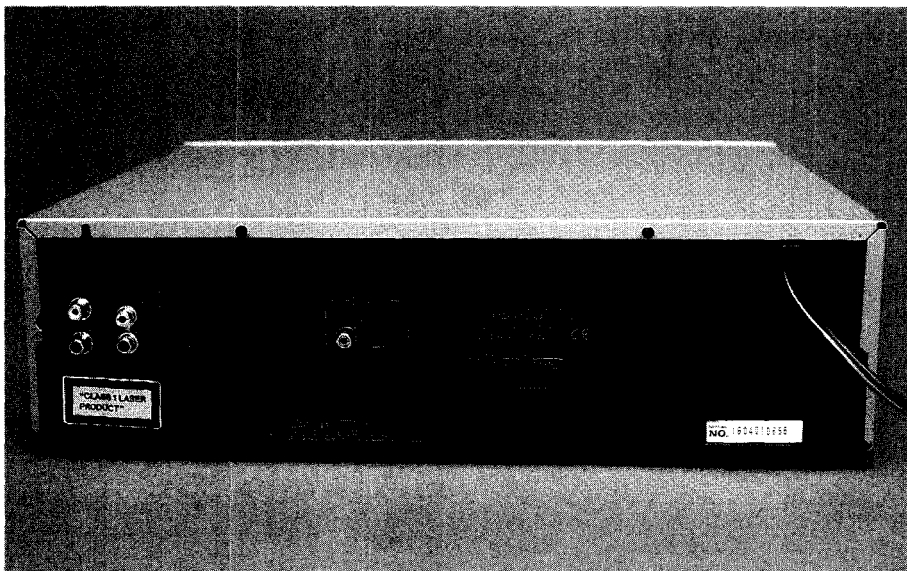
The rear of the Onkyo DX-7911. It provides both optical and electrical digital outputs for external D-A converters (centre), together with both fixed and variable analog outputs (left).
