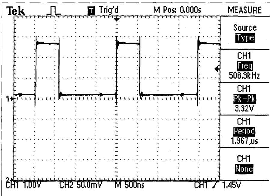
A typical hard copy printout from the TDS 220, with only one channel in use. Note the auto measurements down the right-hand side, and the vertical and timebase settings along the bottom.
