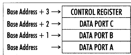
Fig.1: The registers inside the 8255 chip occupy the base address and the three addresses above it.
