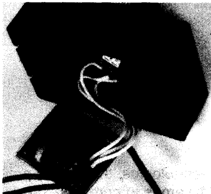
Left: This is the PCB that sits near the radio. The pot is fixed to the plastic box, rather than being mounted on the board. Note that changes have been made to the PCB design since this shot was taken. See the layout diagram for final component placement.
