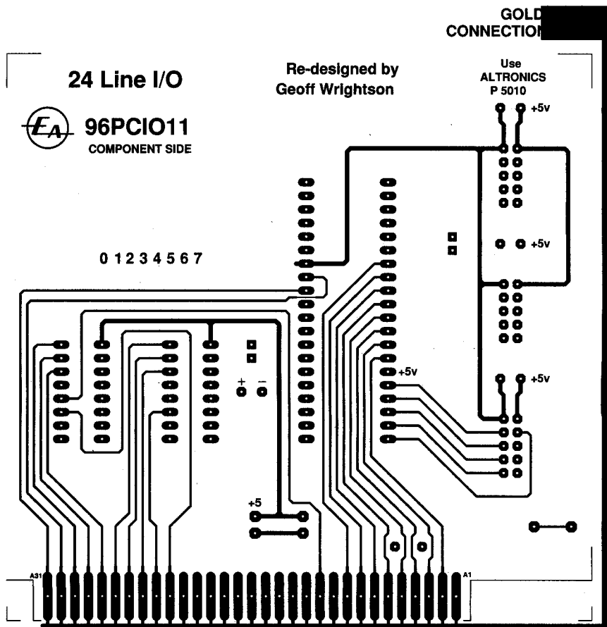
The copper patterns for both sides of the PCB, by courtesy of RCS Radio.
