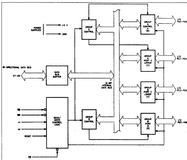
Fig.2: Taken from Intel's handbook, a block diagram showing the internal structure of the 8255 I/O controller.
