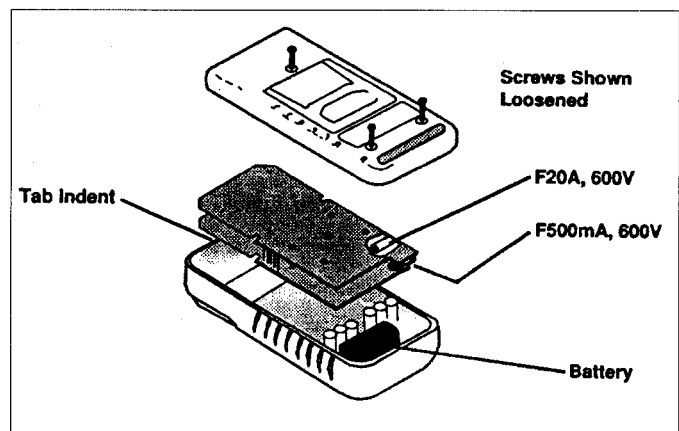
Fig.6: Battery and fuse replacement is very easy on the 8088 meter. However when changing the fuses ensure that they have the correct rating, otherwise meter damage may result.
