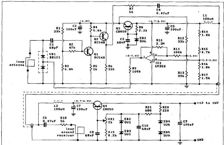
The top half of the circuit is on the PCB mount at the antenna end. The bottom half is at the radio. The antenna is tuned by the varicap diodes, whose capacitance varies with the voltage set by VR1.
