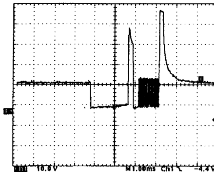
Fig.5: The injectors on a VL Commodore and some other vehicles are current controlled, and a pulsed wave form makes it difficult for the 8088 to measure injector open time.
