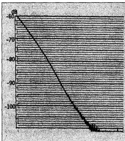
The measured 'fade to noise' performance, below -60dB; a small amount of nonlinearity, but very little jitter or dither thanks to Onkyo's refinements.
