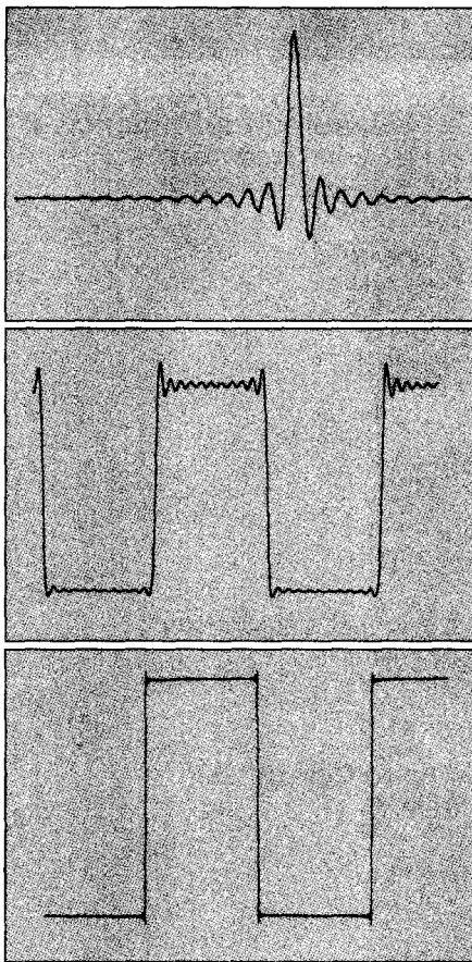
The Onkyo's measured impulse response (top), plus the square wave response at 1kHz (centre) and 100Hz (bottom). All are particularly well controlled, testifying to the careful design of the player's post-conversion filtering. An exceptional result!
