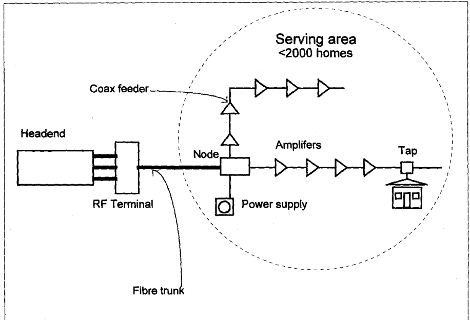
Fig.1: The main components of a hybrid fibre/coax (HFC) broadband network. The signals travel from the headend and the RF terminal via a fibre-optic trunk to each area node, from which they are distributed via co-axial cable feeders. Amplifiers boost levels and maintain signal quality in the coax, and taps split off the individual subscriber drops. Australia's new HFC networks have an RF bandwidth of 750MHz, compared with 550MHz in the USA and 860MHz in Europe.
