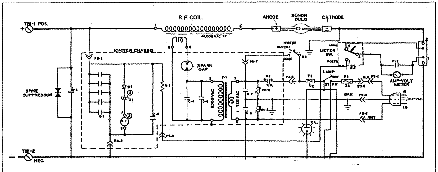
The circuitry for igniting and running the 3600W Xenon arc projector lamp, as discussed in Reg Leahy's drive-in story. The ignitor is essentially a spark gap driving a Tesla coil, to produce a burst of high voltage RF.
