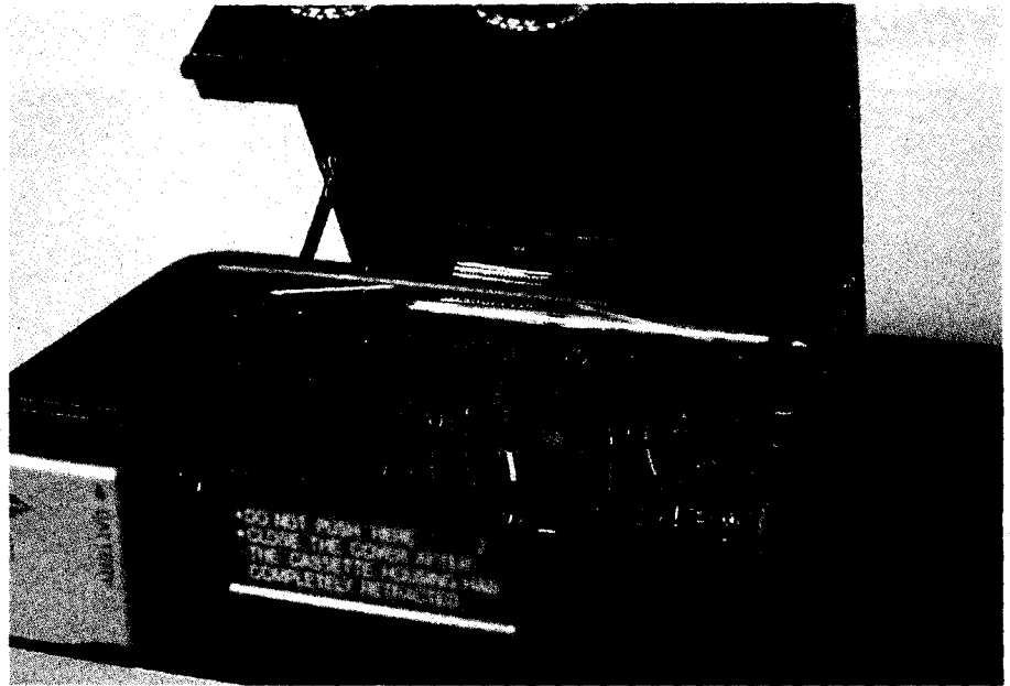
Inside the JVC Cybercam's tape well. A head drum speed of 9000rpm demands a hard wearing tape coating.
