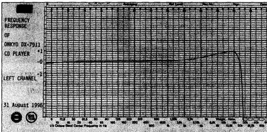
The measured replay frequency plots for the right and left channels. Arguably preferable to the 'ruler flat' response of some CD players, the modest 1dB peak around 16kHz is inaudible and is one consequence of the low-pass filter's characteristic. Another is a relatively gentle roll-off above 20kHz, with less phase shift.
