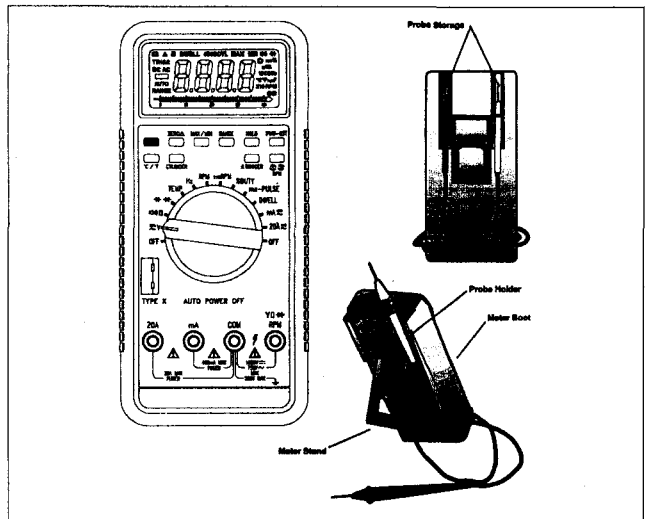
Fig.2: With the CIE 8088 Automotive meter, the rotary dial selects the particular function and the buttons select the required mode. The protective boot also provides a place to keep the leads when they are not being used.
