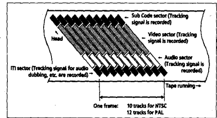
Above: The track pattern used for the DV format. (Courtesy Sony)
