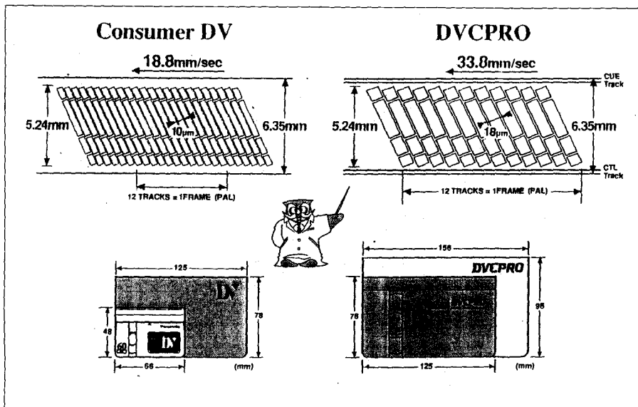
Above: The track pattern used for the DV format. (Courtesy Sony)
