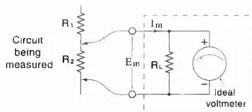
Figure 1 Voltmeter equivalent circuit
