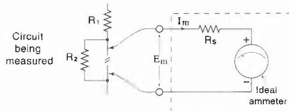
Figure 2 Ammeter equivalent circuit
