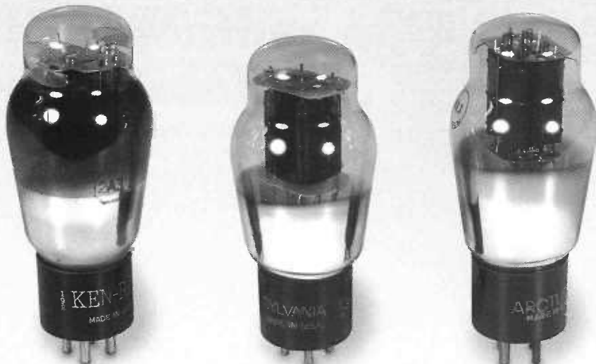
Ken-Rad Bi-Plate 2A3 (1940s); Sylvania Bi-Plate 2A3 (1940s); Arcturus Bi-Plate 2A3 (1938)
