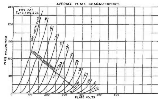
Original 2A3 Specifications from 1933 RCA Tube Manual
