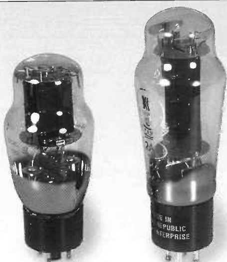
Svetlana 6B4G (1982); KR2A3 (1990s)
