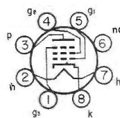
EL34 Specifications from 1965 Amperex Tube Manual
