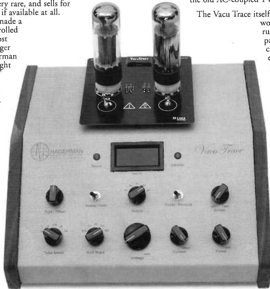
Hagerman Vacu Trace Curve Tracer
