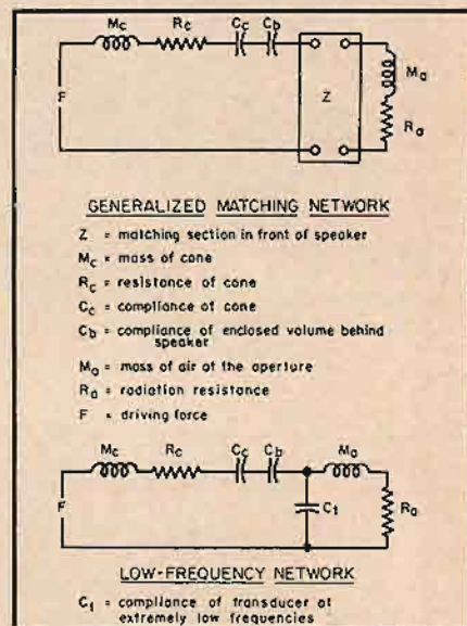
Fig. 4. Equivalent mechanical networks of exponential slot enclosure.
