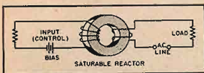
Fig. 2. In the saturable reactor, the core remains stationary, but its permeability is varied by a control circuit in which d.c. flows.
