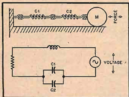
Fig. 4-4. Mechanical system with springs in tandem, and analogous electrical circuit.
