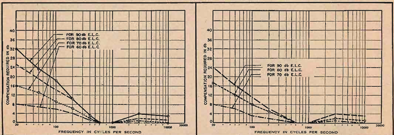
Fig. 2 (left). Compensation required when reproducing the 90, 80, 70, and 60 db equal loudness contours at a level of 50 db. Fig. 3 (right). Compensation required for reproduction at a level of 60 db.
