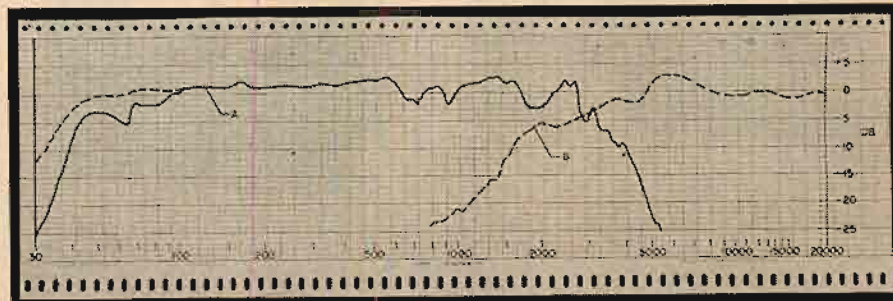
Fig. 7. Frequency response of individual LF (curve A) and HF (curve B) units when assembled and enclosed in the 606A corner cabinet.
