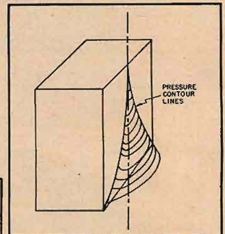
Fig. 2. Sketch of pressure contours from the exponential slot.
