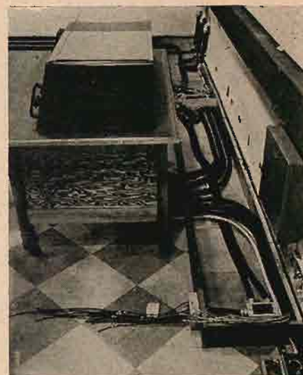
Fig. 6. Interconnection Cable Trough. Racks are to be located at the far end of the console. At top right, cables of three level groups converging on the control room run down the wall to the trough and thence to the racks and console. See Fig. 1 of preceding installment for front view. Most of the floor circuits are run in flexible conduit which is ordinarily not required in trough work. Official Defense Dept. Photo.
