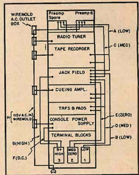
Fig. 3. Rack Cabling Layout. There are relatively few circuits and, if necessary, the low-level pairs as well as the medium- and zero-level circuits could all have been carried on terminal block 2. Note Wiremold distribution system which eliminates a.c. terminal block. Also note that high-level and power circuits are on opposite side of rack from lower levels.
