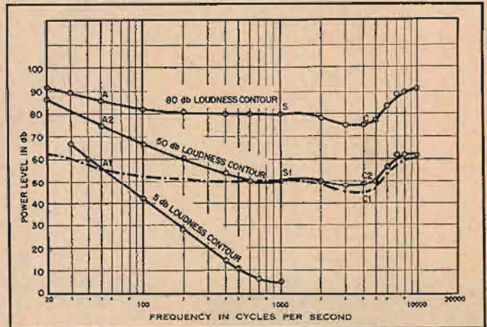
Fig. 1. Effect of reducing volume with normal volume control.
