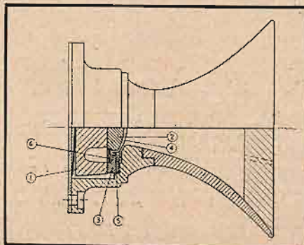
Fig. 2. Cross section of the 3000A high-frequency unit and horn assembly.
