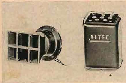
Fig. 4. The high-frequency horn and driver assembly together with its matching crossover network.
