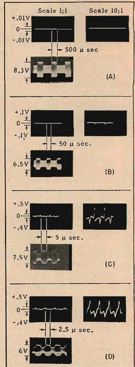
Fig. 12. Magnetic flip flops driven at high rates. Upper pair of photos in each box show input pulses which are, in each case, minimum amplitude required to set flip flop. Increased pulse amplitude is required at higher rates. The lower photos show r.f. envelopes. (A) Pulse repetition rate = 2000 pps. (Time between pulses = 500 \mu sec) R.F. envelope = 1.42 mc. (B) Pulse repetition rate = 20,000 pps. (Time between pulses = 50 \mu sec) R.F. envelope = 1.32 mc. (C) Pulse repetition rate = 200,000 pps. (Time between pulses = 5 \mu sec) R.F. envelope = 1.4 mc. (D) Pulse repetition rate = 400,000 pps. (Time between pulses = 2.5 \mu sec) R.F. envelope = 1.5 mc.
