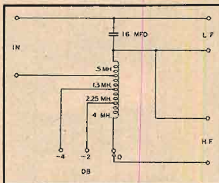
Fig. 5. Schematic of the N-3000A crossover network.
