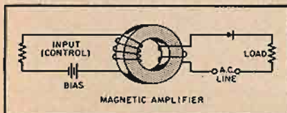
Fig. 3. The addition of a rectifier in the load circuit improves performance by eliminating self-saturation.
