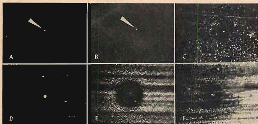
Fig. 1. Microphotographs showing the development of a typical nodule in magnetic tape: (A) Pinhole in virgin tape; (B) tape sample including the hole after one passage over the head assembly; (C) same sample after five passages; (D) after 12 passages; (E) after 1000 passages; and (F) after 1800 passages.
