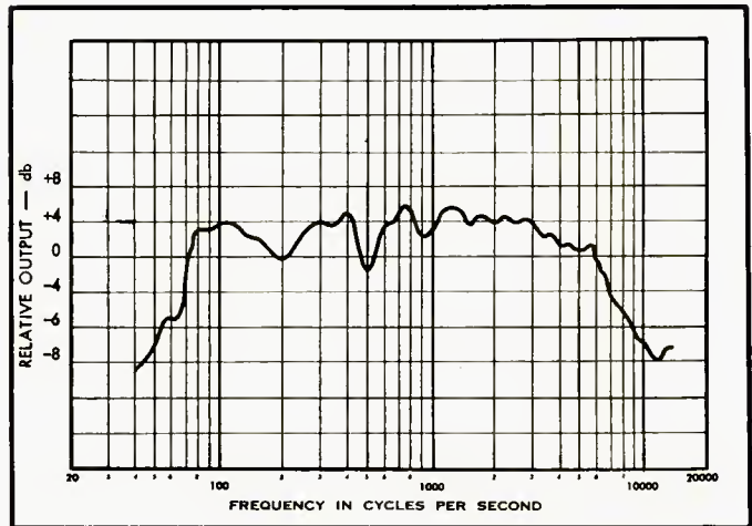
Fig. 4. Unequalized response measurement of the complete system.
