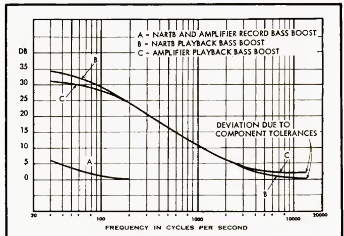
Fig. 7. NARTB and amplifier bass equalization curves.
