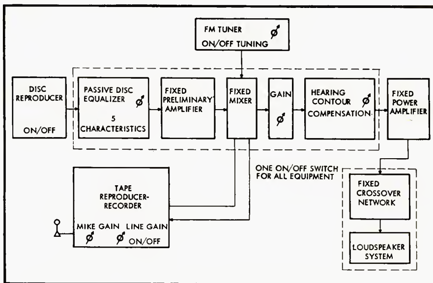
Fig. 2. Block diagram of ideal arrangement for an audio system.
