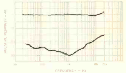
Fig. 1 — Frequency response and separation.
