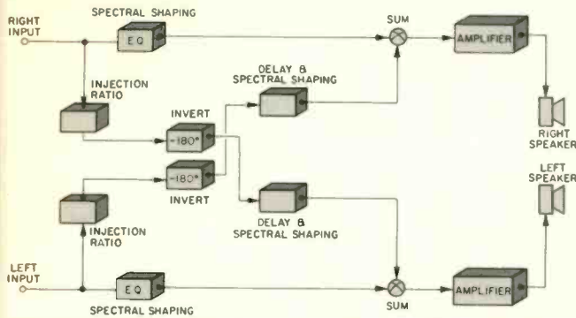
Fig. B2—Basic block diagram of the Sonic Hologram Generator.
