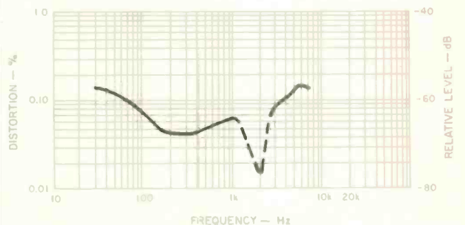
Fig. 6—Third harmonic distortion vs. frequency in Dolby mode at 10 dB below Dolby level with Denon DXM tape.
