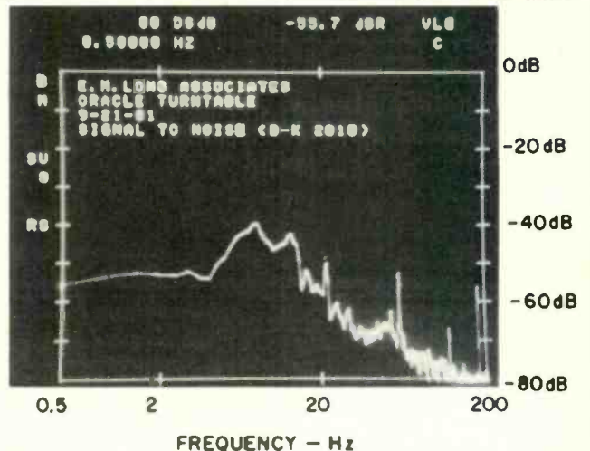
Fig. 8B—As in Fig. 8A but from 0.5 to 200 Hz with log scale. Tonarm resonance is responsible for most of the increase from 7 to 10 Hz, but the level is over 40 dB down from the 10 cm/S reference.
