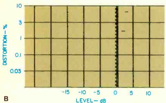
Fig. 5 — A slight improvement in 3rd-order harmonic distortion is noted when 16-bit mode is used on Sony PCM-F1 (A), but so long as recording level does not exceed 0-dB (B), 3rd-order HD is insignificant in both 14- and 16-bit modes.
