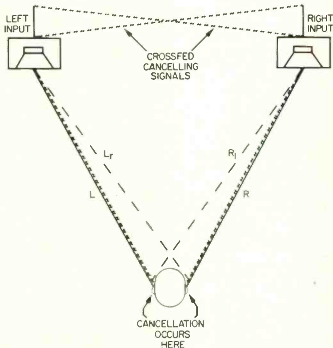
Fig. 4— Careful addition of the crossed cancelling signals will cause the L_r and R_l signals to drop out of the sound field at a selected listening location.
