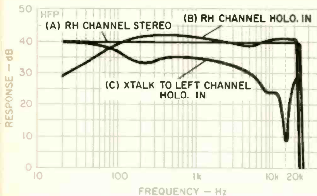
Fig. B3—Frequency shaping in the Hologram Generator: (A) Response in standard stereo, (B) contouring on main channel through Generator, and (C) relative level and contouring on cross-fed signal. Chart recorder causes roll-off above 20 kHz.
