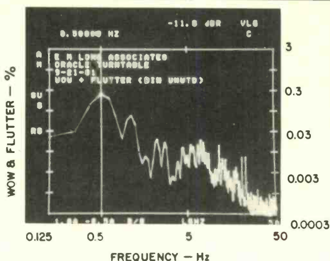
Fig. 5—Wow and flutter spectrum from 0.125 to 50 Hz, with main wow at 0.5 and 1 Hz (see text).
