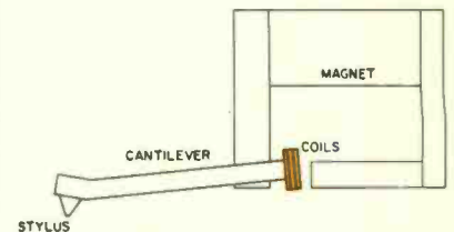
Fig. 2C — Simplified drawing of a moving-coil cartridge. (After Ortofon.)
