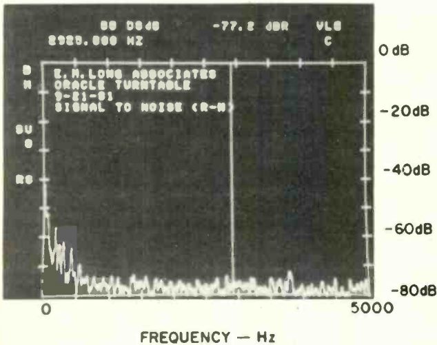
Fig. 9A—Similar to Fig. 8A but measured using Thorens Rumpel-messkoppler and showing an even lower noise floor.
