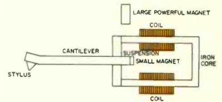
Fig. 2B — Simplified drawing of an induced-magnet cartridge. (After Ortofon.)
