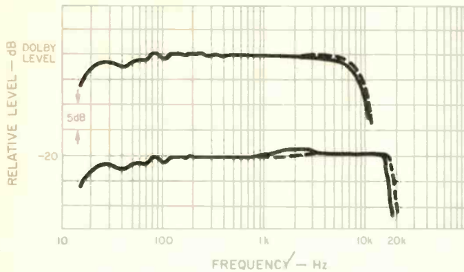
Fig. 1—Frequency responses with Denon DX3 tape with and without (---) Dolby NR.
