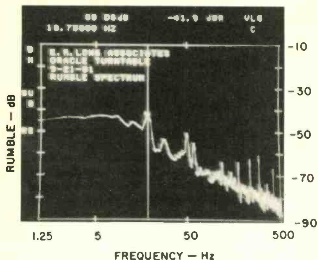
Fig. 4—Rumble spectrum, with most components below 20 Hz. Spikes are harmonics of hum and occur below -60 dB.
