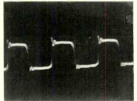
Fig. 2 — Square-wave response.
