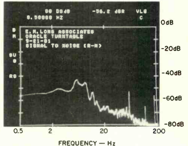
Fig. 9B—Similar to 8B but with the Rumpel-messkoppler. The arm resonance is still evident, but the spike at 20 Hz is not, indicating it is probably an artifact of the test disc.
