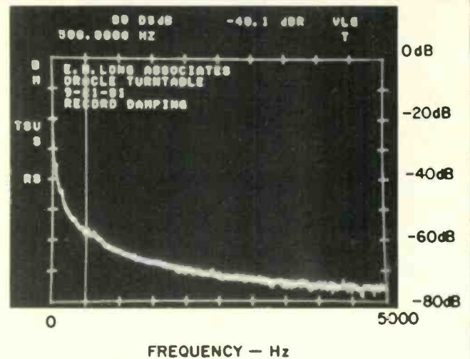
Fig. 11—Spectrum of a record's internal resonances. See text.
