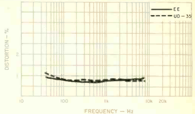
Fig. 4 — Distortion vs frequency.
