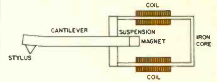
Fig. 2A — Simplified drawing of a moving-magnet type phono cartridge. (After Ortofon's "Everything You Need to Know About Cartridges.")
