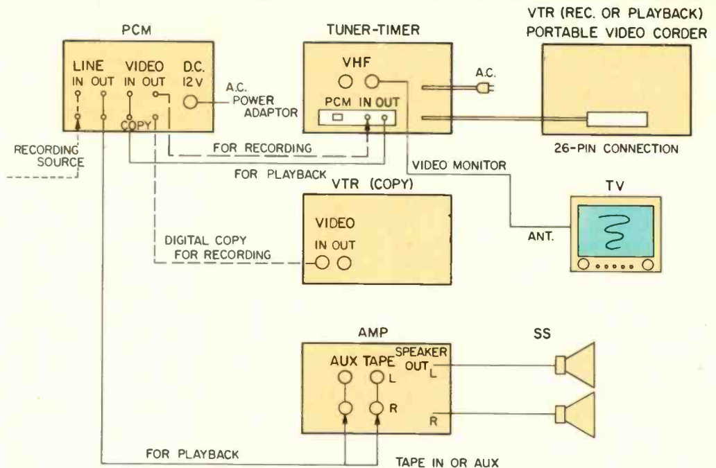
Fig. 2 — Digital audio PCM system connections.
