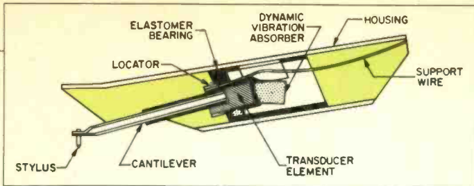
Fig. 1 — Cut-away view of the V-15 Type IV cartridge, courtesy Shure Bros.
