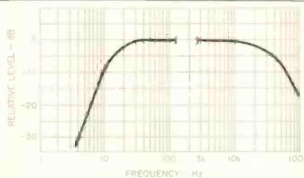
Fig. 1 — Frequency response of 4100 filters.
