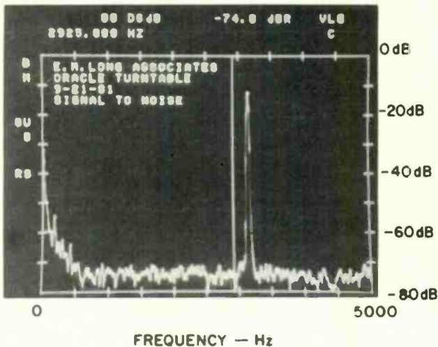
Fig. 8A—Spectrum of signal-to-noise ratio with 3150-Hz tone from B&K 2010 test disc. (Note: Scale is linear.)
