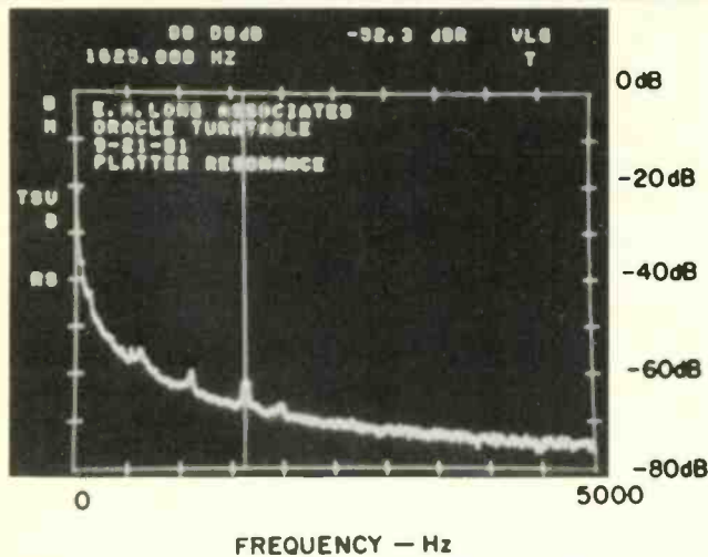
Fig. 10—Spectrum of platter resonance. See text.
