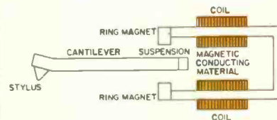
Fig. 5 — Simplified drawing of Ortofon's Variable Magnetic Shunt principle. (After Ortofon.)
