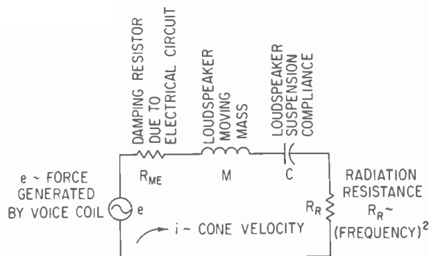
Figure 2. The analog circuit of a loudspeaker installed in an infinite baffle enclosure.
