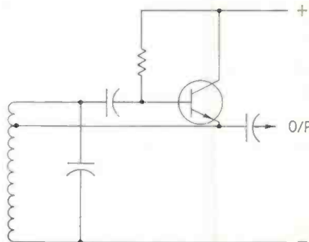
Figure 1. A type of tuned circuit oscillator that can operate in more than one way, according to circuit proportions.
