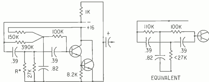
Figure 4. The same circuit as in Figure 3 redrawn to show the twin-T feedback reduced to more familiar relationship. On the right, the values are simplified to an equivalent simple twin-T.
