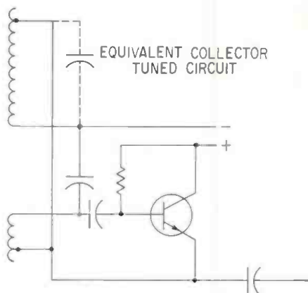
Figure 2. The same circuit redrawn to make the emitter the "ground" reference point, to help visualize transistor operation.
