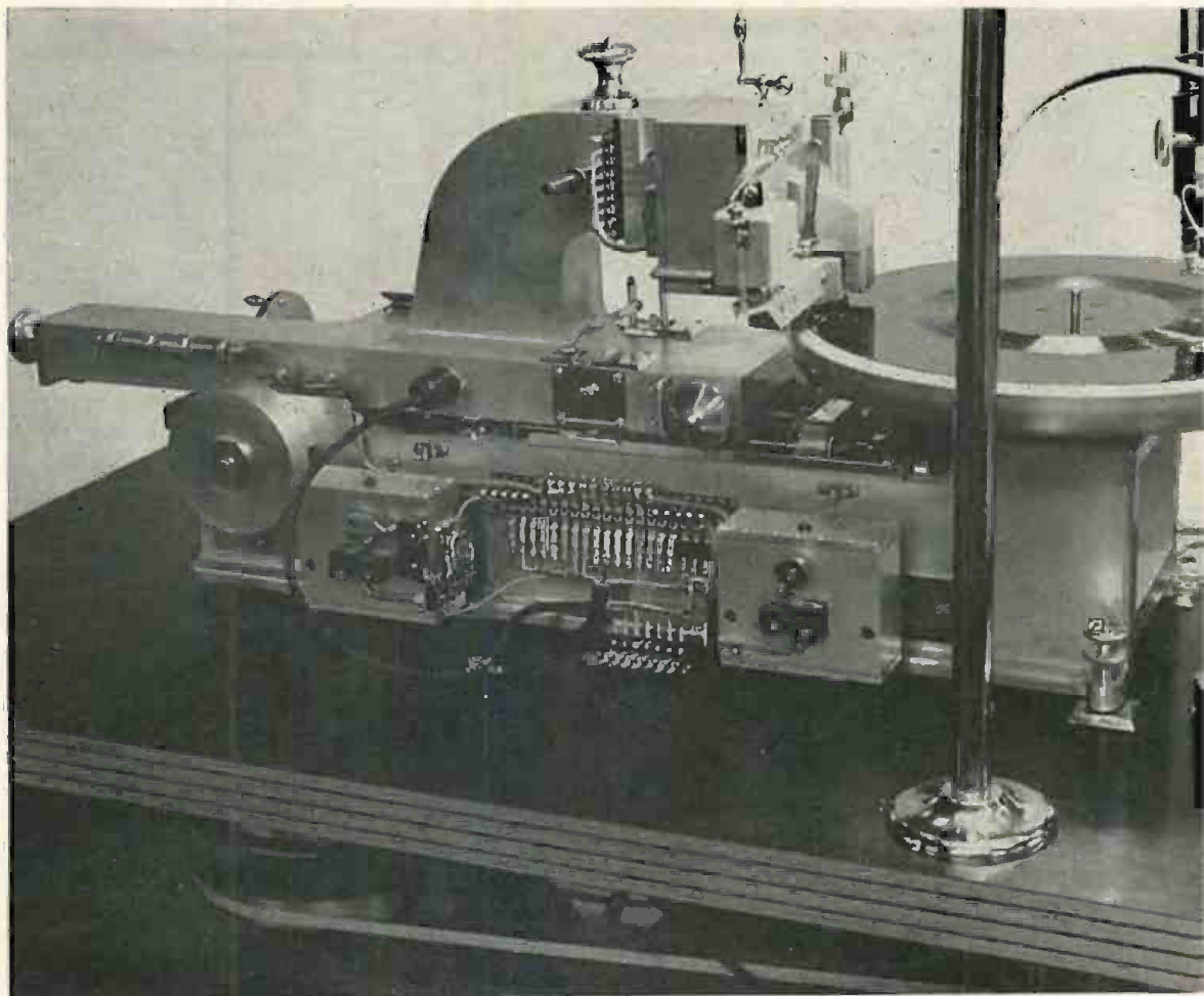
Art in metal: a Scully variable-pitch recording lathe.
