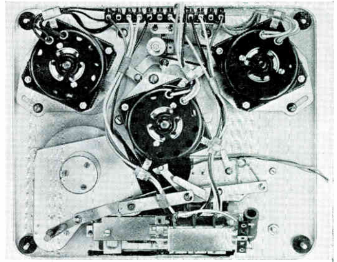
The underside view of the Collaro Studio Deck
