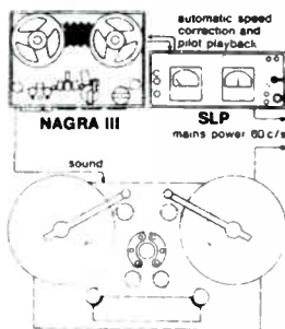
Layout showing the SLP connected to the Nagra III
