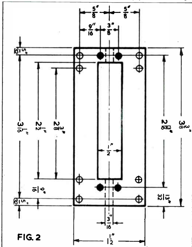
Fig. 2. The frame, \frac{1}{4} Paxolin. Holes marked solid are 10 BA tapped. Holes in outline are 8 BA clearance
