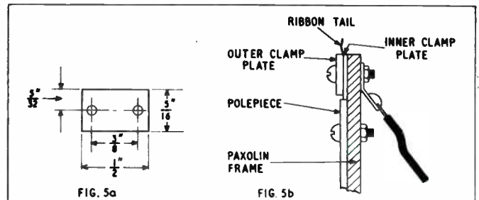
Fig. 5a. Ribbon clamping plates. Make two at \frac{3}{32} " thick and two at \frac{1}{4} " thick. Holes are 10 BA clearance. Fig. 5b is an enlarged edge-on view of one end of frame showing part of poles, ribbon and ribbon clamp
