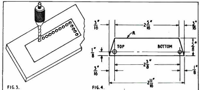
Fig. 3. A method of cutting out the central slot in the frame, using a drill Fig. 4. Pole-piece dimensions. Note that the 8 BA clearance fixing holes are filed oval
