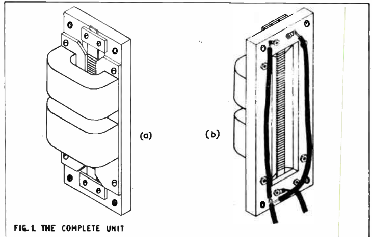
FIG. 1 THE COMPLETE UNIT
