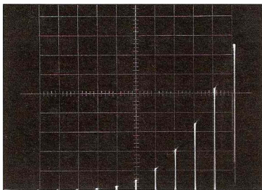
Figure 1 Normal 12AT7
