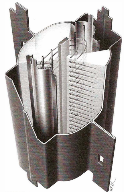
6L6 Cutaway
