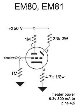
Figure 2: connection of some common eye tubes as audio level meters.
