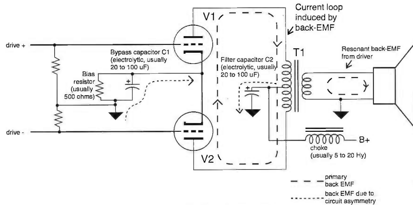
Figure 4: Path of back-EMF in push-pull triode amplifier.
