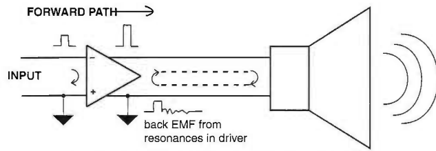
Figure 1: Back-EMF resonances.
