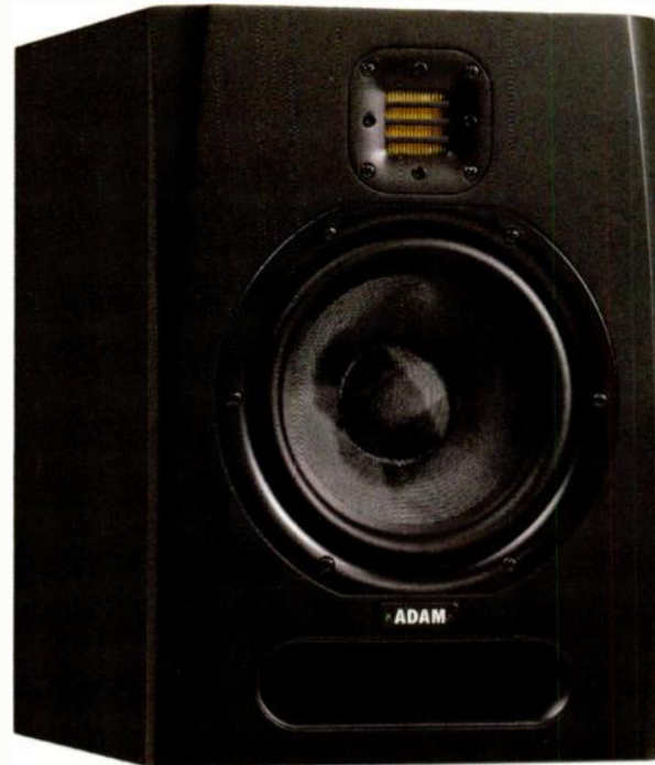
The affordable F7s use the same air motion transformer tweeter found in ADAM's more expensive models
