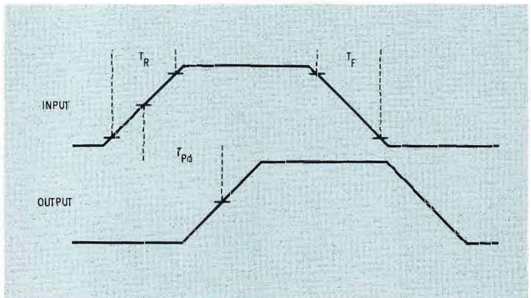
Fig. 2 Timing parameters of digital signals. Propagation delay time ( T_{pd} ) is a measure of how fast an output responds to a change in an input measured from the 50 percent point. Rise time ( T_r ) and fall time ( F_t ) are measured from the 10 to 90 percent points.
