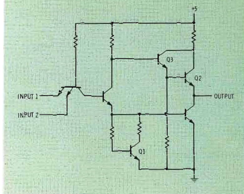
Fig. 8 74H00 TTL. By replacing the pull down resistor R3 on Fig. 7 with an active pull down Q1 and replacing the upper output transistor and diode with a Darlington pair Q2, Q3 the speed of the 7400 gate is vastly increased.
