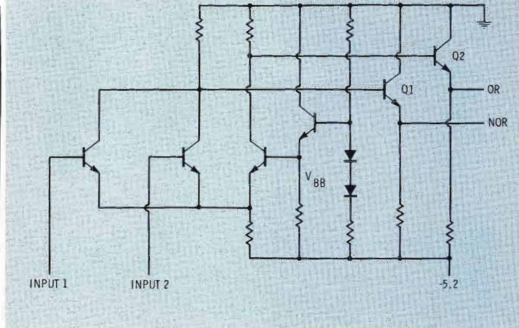
Fig. 10 Basic ECL Gate. ECL is the fastest form of logic today. Its differential outputs and wide acceptance make this a flexible family to design with. Where high speed is a major concern, ECL is often used.
