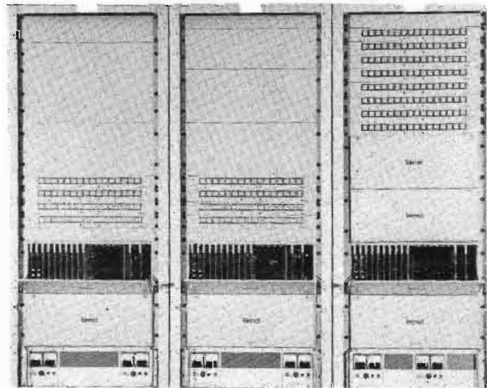
Routing Switchers
