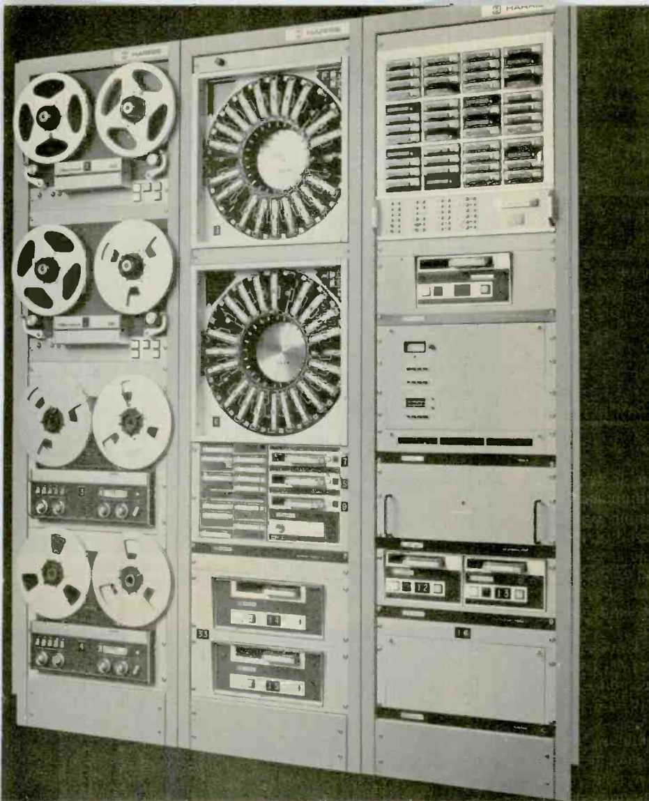
Harris System 90 (left) has minicomputer, memory, audio switching and power supply in third rack, below multicart machine. Example shown has one audiofile, two Carousels, four reel-to-reel machines; other configurations are readily made (system handles up to 16 inputs).
