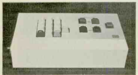
Control box for Audio Services' System 1 automation system (above) can be used remote from studio, connected to studio by FSK digital signals over telephone lines. Remote man has same control of system has in studio.
