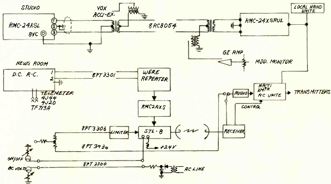
Block diagram shows main features of remote control system, together with metering for the STL transmitter.
