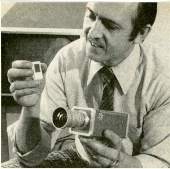
Experimental solid-state TV camera shown by Bell Labs. Chip is charged-coupled image sensing device.
