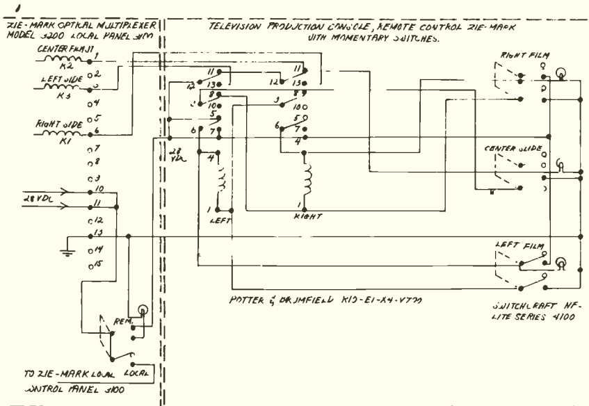
Optical Multiplexer remote control designed by Davis
