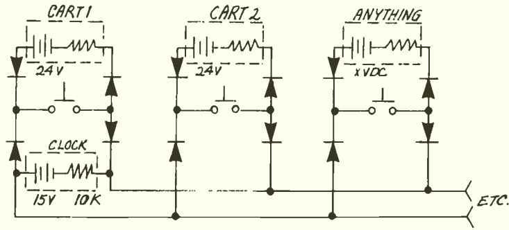
Burnham's Control Circuit
