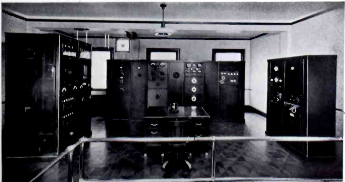
THE 1.8 RCA VICTOR TRANSMITTER RECENTLY INSTALLED ATOP THE WORCESIER TELEGRAM AND EVENING GAZETTE BUILDING IN WORCESIER, MASS. THE LOFTY ANTENNA IS SUSPENDED BETWEEN STEEL MASTS LOCATED ON THE ADJACENT ROOFS OF THE PARK BUILDING AND THE BANCROFT HOTEL. THE STATION OPERATES ON 500 WATTS AND IS EQUIPPED WITH A CATHODE-RAY MODULATION INDICATOR
