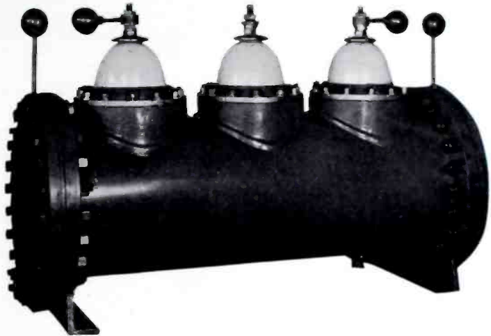
FIGURE 1—RCA VICTOR'S NEW 2000 KVA HIGH-PRESSURE CAPACITOR DEVELOPED FOR USE IN 50 KW TO 200 KW TRANSMITTER
