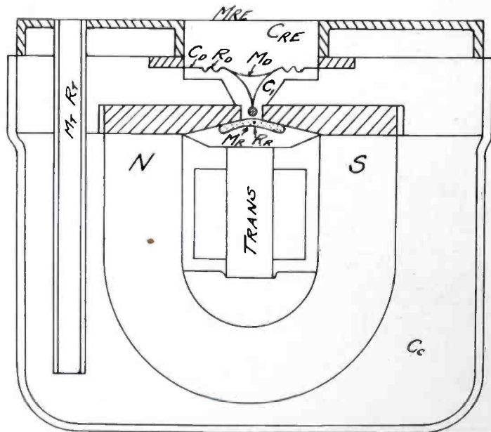
FIGURE 5—THE NEW RCA VICTOR TYPE 50-A INDUCTOR MICROPHONE, ARRANGED FOR OVERHEAD SUSPENSION
