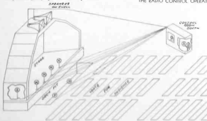
RCA VICTOR SOUND INSTALLATION FOR STATION WCAU AT ROBIN HOOD DELL
