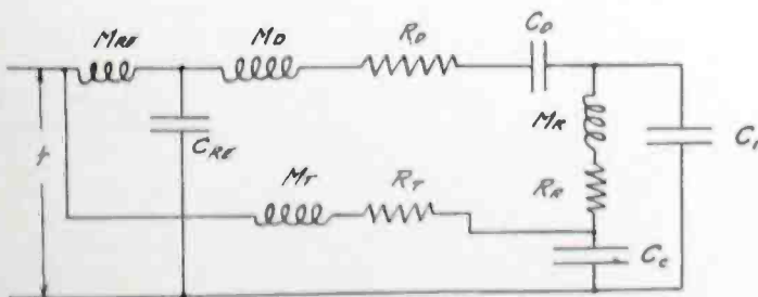
FIGURE 9—EQUIVALENT ELECTRICAL CIRCUIT OF THE MECHANICAL SYSTEM
