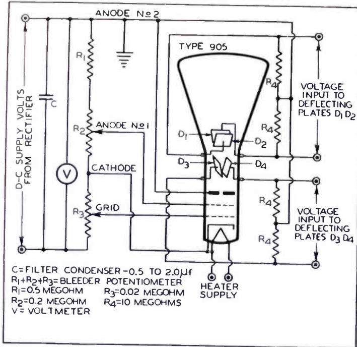
FIGURE 1—DIAGRAM FOR A MODERN TUBE
