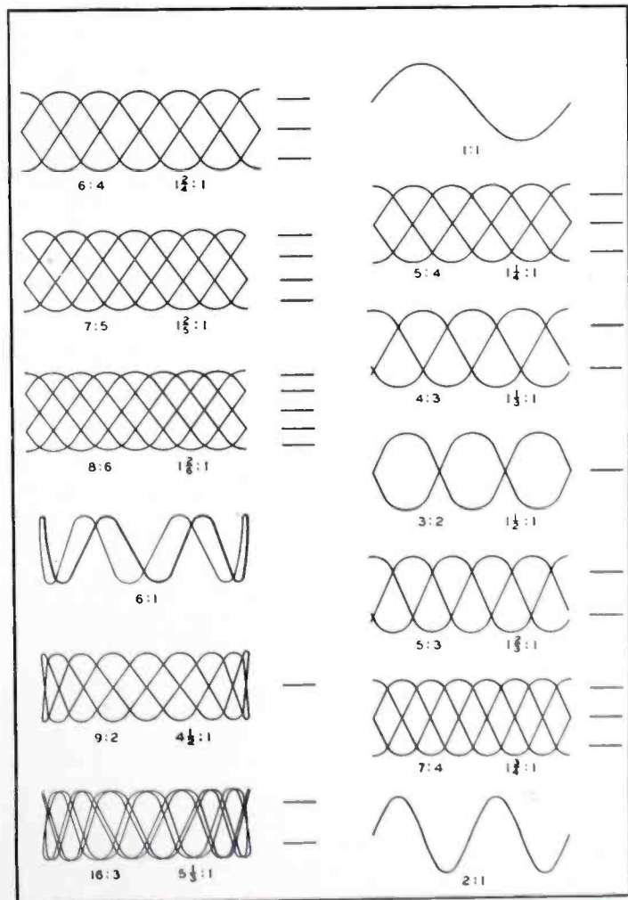
FIGURE 4—LISSAJOUS FIGURES
