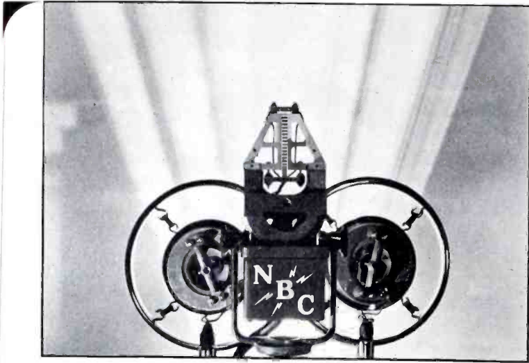
"MIKES"—A NAKED VELOCITY MICROPHONE AND TWO OF THE CARBON TYPE
