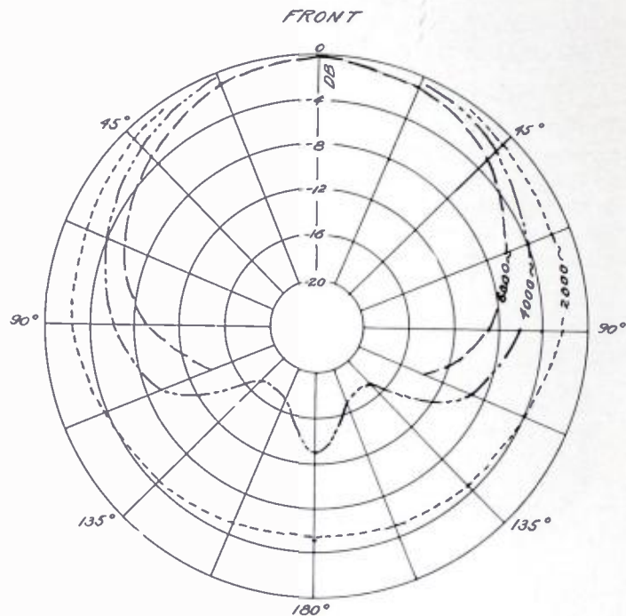
FIGURE 3—DIRECTIONAL CHARACTERISTICS OF THE NEW INDUCTOR MICROPHONE
