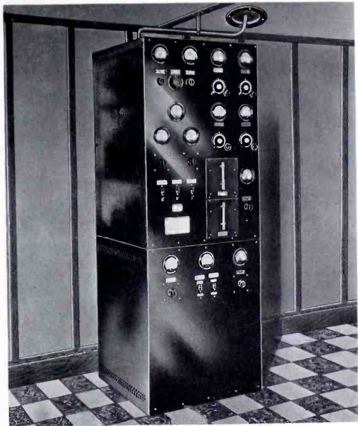
FIGURE 1—FRONT VIEW OF ET-4230 TRANSMITTER. NOTE MULTIPLICITY OF METERS
