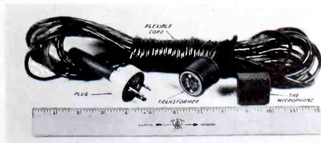
THE RCA VICTOR TYPE 30-A LAPEL VELOCITY MICROPHONE A PRACTICAL INSTRUMENT CAREFULLY DESIGNED FOR RUGGED COMMERCIAL SERVICE FURNISHED COMPLETE WITH COUPLING TRANSFORMER, 95 FEET FLEXIBLE RUBBER CORD AND PLUG
