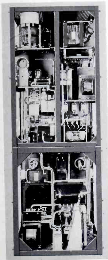
FIGURE 3—BACK VIEW. THE UPPER PART OF THE TRANSMITTER IS DIVIDED INTO TWO COMPLETELY SHIELDED COMPARTMENTS. ON THE LEFT IS LOCATED ALL THE RADIO FREQUENCY EQUIPMENT AND ON THE RIGHT THE AUDIO AND RECTIFIER EQUIPMENT
