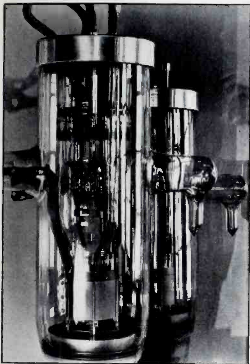
TRANSMITTING RADIOTRONS—DRAMATICALLY SILENT RADIO GIANTS
