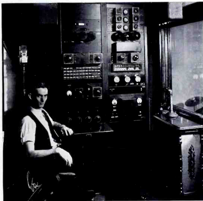
J. E. ADAMS, CHIEF CONTROL OPERATOR AT WFBC, IN THE CONTROL ROOM WHICH NOW INCLUDES AN RCA VICTOR 41-B PREAMPLIFIER, A NEW 4-CHANNEL MIXER, AND A VELOCITY MICROPHONE
