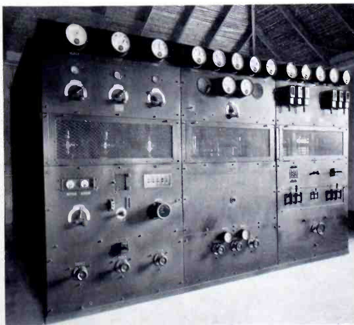
RCA VICTOR 5 KW TRANSMITTER AT CARACAS, VENEZUELA
