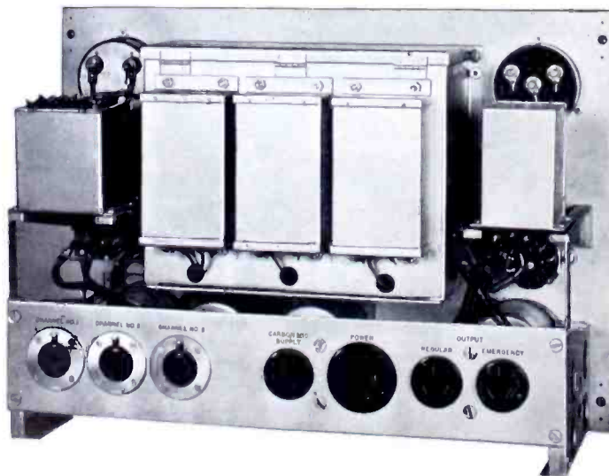
FIGURE 1—CHASSIS OF THE AMPLIFIER-CONTROL UNIT (REAR VIEW)
