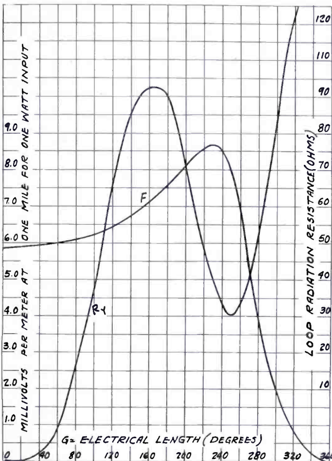
FIGURE 6—RADIATION RESISTANCE AND FIELD STRENGTH AS A FUNCTION OF ANTENNA LENGTH. INPUT POWER EQUALS 1 WATT. (1) TO OBTAIN FIELD STRENGTH FOR ANY OTHER POWER THAN 1 WATT, MULTIPLY VALUE ON CURVE BY THE SQUARE ROOT OF THE POWER IN WATTS. (2) TO OBTAIN THE RADIATION RESISTANCE REFERRED TO THE BASE, DIVIDE VALUE GIVEN ON CURVE BY \sin^2(G)
