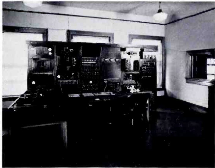
WTAR, NORFOLK, VA.—AMPLIFIER AND CONTROL BOARD, STUDIO MASTER CONTROL ROOM, SHOWING RCA VICTOR 33½ AND 78 R. P. M. TRANSCRIPTION EQUIPMENT
