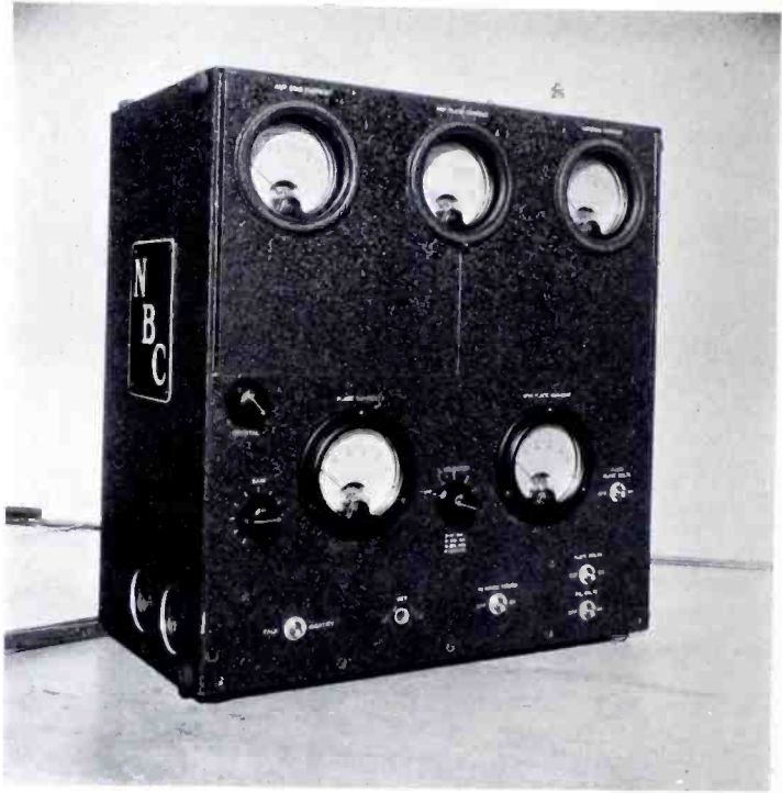
BEFORE THE ASCENT THE COMPACT LITTLE 8-WATT TRANSMITTER THAT MADE HISTORY
