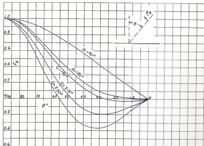
FIGURE 5—VERTICAL RADIATION CHARACTERISTICS OF VERTICAL ANTENNAS
