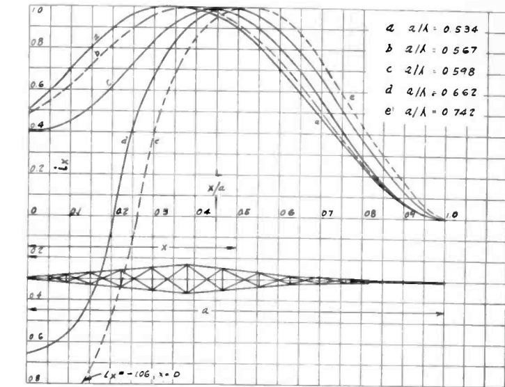
FIGURE 5—CURRENT DISTRIBUTION ON TYPE A ANTENNA AS A FUNCTION OF FREQUENCY
