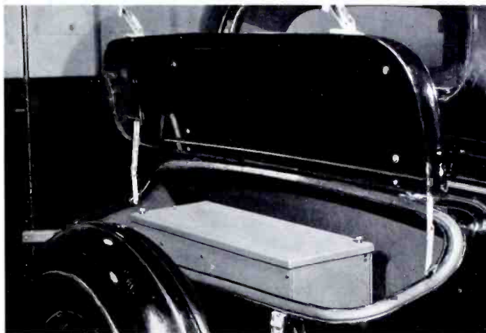
HOW THE ET-5022 MOBILE TRANSMITTER MAY BE CONVENIENTLY INSTALLED IN THE REAR OF A COUPE
