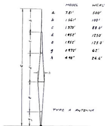
FIGURE 3—DIMENSIONS OF TYPE A MODEL ANTENNA
