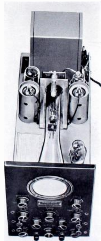
INTERIOR VIEW OF TMV-122 B OSCILLOGRAPH
