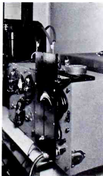
FIGURE 5—THIS VIEW SHOWS HOW THE ADJUSTABLE SCALE DEVICE IS APPLIED TO THE RCA TMV-75-B FIELD-INTENSITY METER
