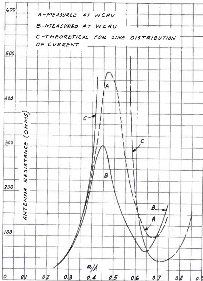
FIGURE 15—RADIATION RESISTANCE VS. a/\lambda .
