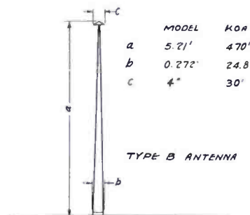
FIGURE 7—DIMENSIONS OF TYPE B MODEL ANTENNA
