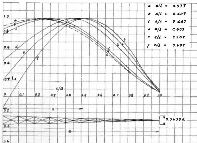
FIGURE 9—CURRENT DISTRIBUTION ON TYPE B ANTENNA WITH A SMALL CAPACITY
