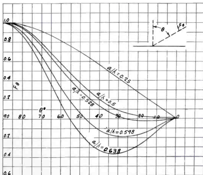
FIGURE 14—VERTICAL RADIATION CHARACTERISTICS OF STRAIGHT VERTICAL WIRE
