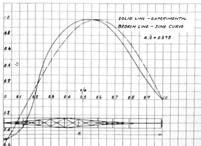
FIGURE 17—CURRENT DISTRIBUTION ON TYPE A ANTENNA EQUIPPED WITH OUTRIGGER AND VERTICAL WIRES.
