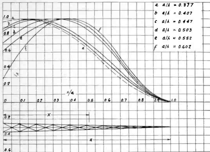
FIGURE 8—CURRENT DISTRIBUTION ON TYPE B ANTENNA
