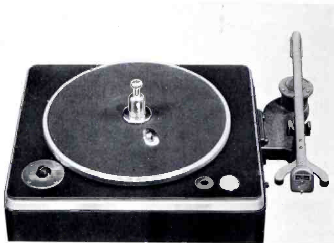
TOP VIEW OF THE NEW RCA VICTOR TYPE 70-A CONSOLE, SHOWING THE TURNTABLE, SUSPENSION ARM, PICKUP, AND SELECTOR SWITCHES. THE SPEED SHIFT BUTTON IS LOCATED ON THE TURNTABLE DISC ITSELF. THE VERTICAL PICKUP TYPE 71-A IS NOT SHOWN
