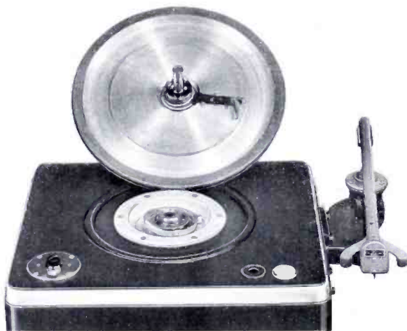
THIS VIEW SHOWS THE TURNTABLE DISC TURNED OVER TO DISCLOSE THE INGENUOUS BALL-BEARING SPEED REDUCTION MECHANISM. THE PAWL ON THE BOTTOM OF THE DISC ENGAGES THE SLOT IN THE CLUTCH RING WHEN 33- \frac{1}{3} R.P.M. OPERATION IS DESIRED
