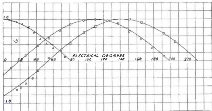
FIGURE 11—CURRENT DISTRIBUTION ON VERTICAL WIRE ANTENNA
