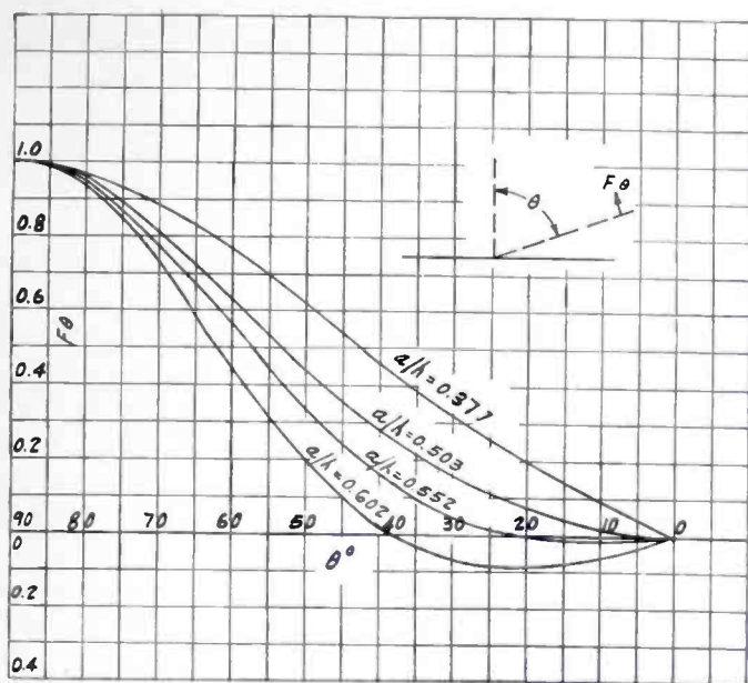
FIGURE 13—VERTICAL RADIATION CHARACTERISTICS OF TYPE B ANTENNA
