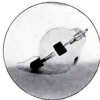
Figure 3. The de Forest Audion.
