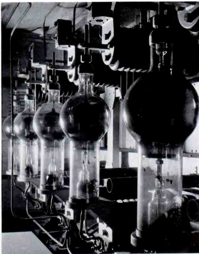
Lineup of rectifier tubes in the 50-C.
