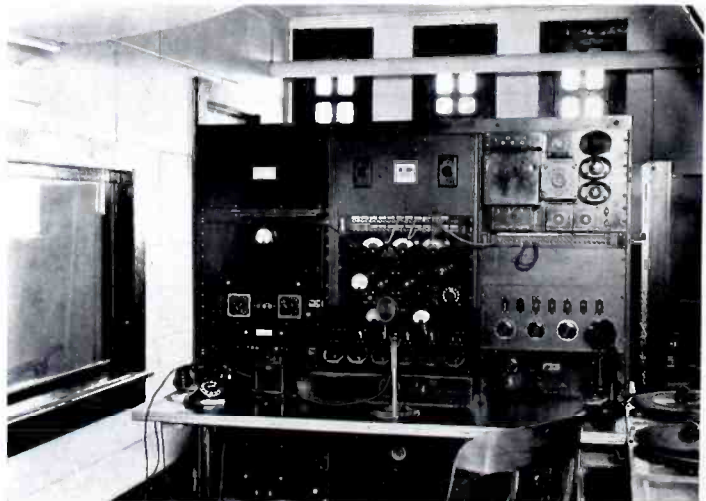
Some of the equipment at WDOD.
