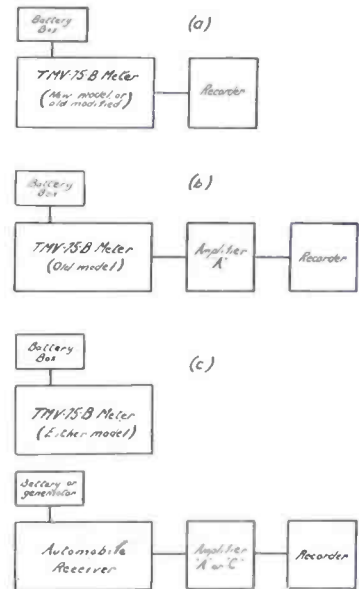
FIG. 9. Alternative arrangements suggested for making recordings in the field. The several advantages are discussed in the text.
