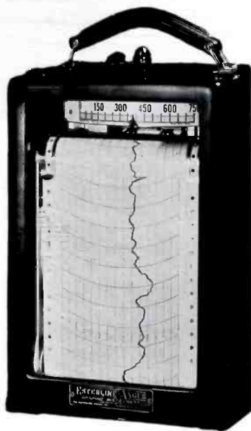
FIG. 3. A graphic recording instrument particularly suited for recording of field intensities. Current of 5 mills is required for full scale deflection.
