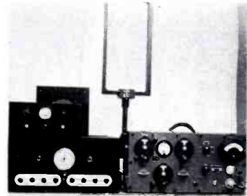
FIG. 13. An arrangement of equipment, similar to Fig. 10f, for making records at a fixed point. The recorder (not shown) is driven by the receiver-amplifier combination, the meter being reserved for calibration. The amplifier operates from the AVC circuit of the receiver, and also takes its power supply from the latter.
