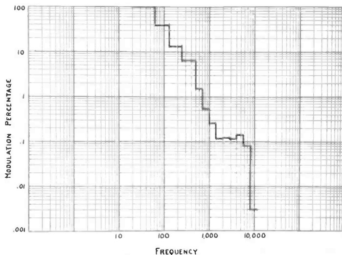
FIG. 1 ABSOLUTE SOUND PRESSURE
