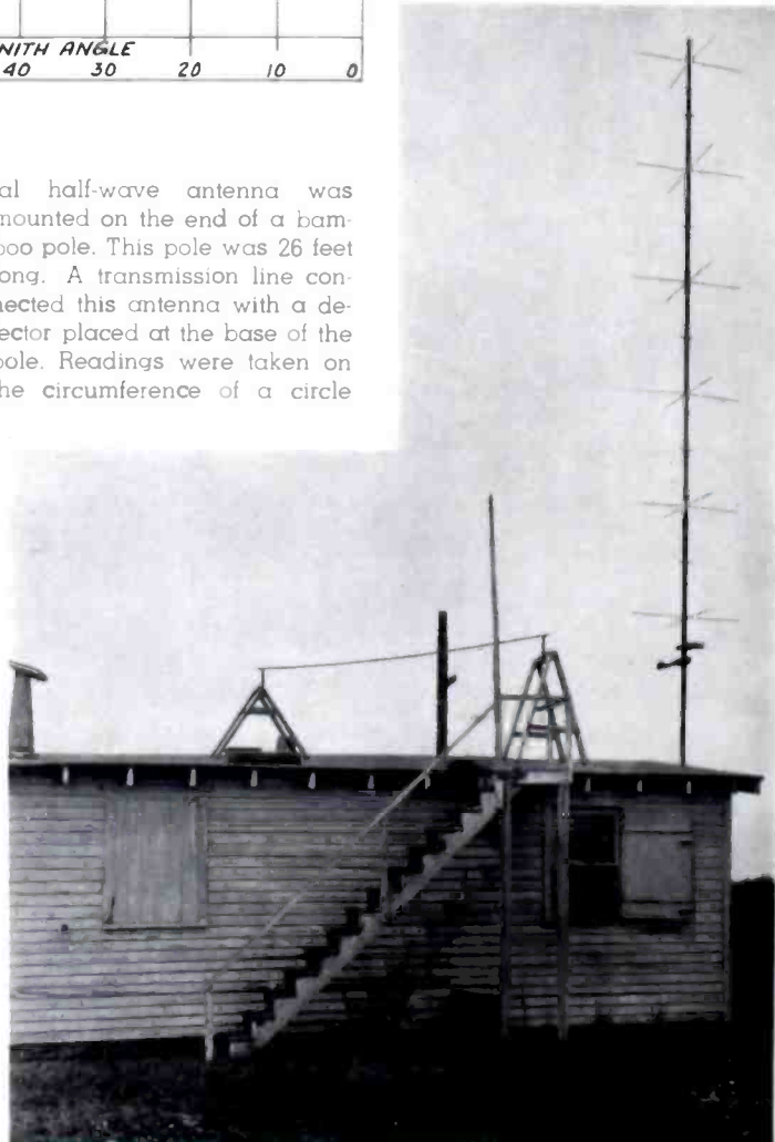
Fig. 9. The experimental model of the turnstile antenna.
