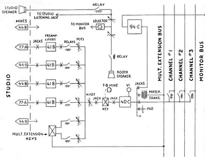
Typical Studio Channel at KEHE.
