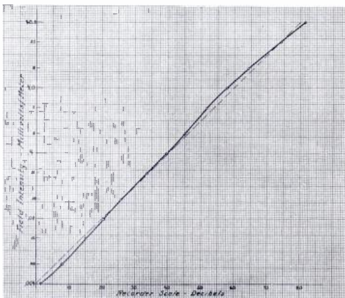
Fig. 6. An actual response curve of the receiver-amplifier combination, made by a direct comparison with readings of the field intensity meter -- such a curve should be made for each station to be observed. It can be done quite easily, either by direct observation of station signals or by using a signal generator.
