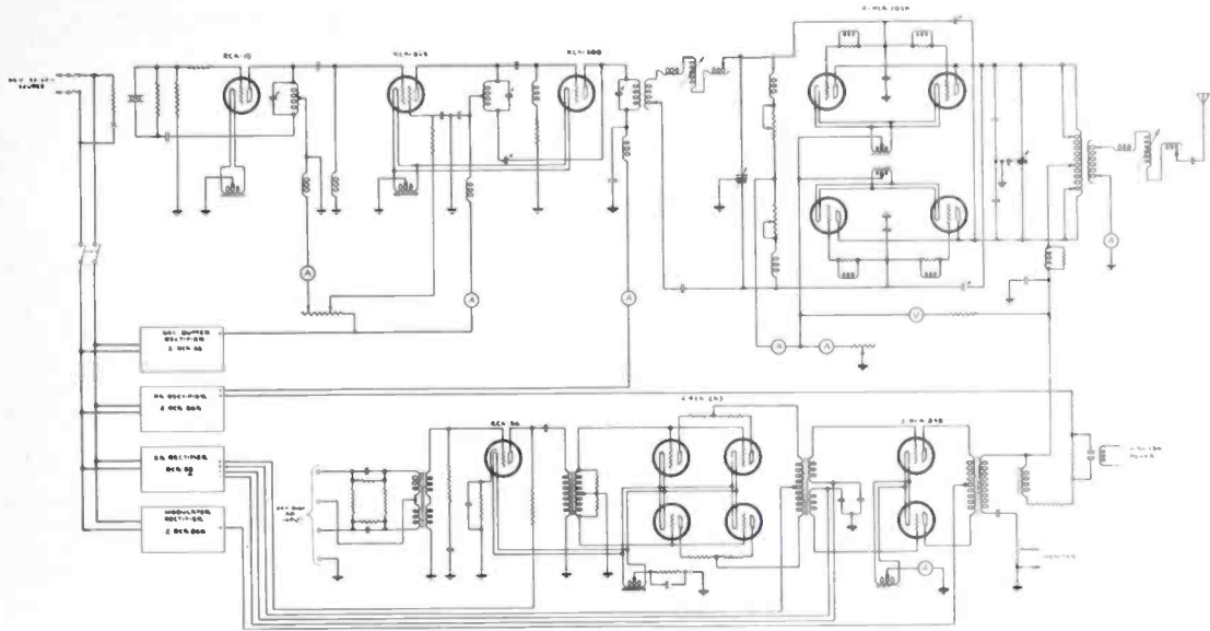
Simplified Schematic of the 250-E
